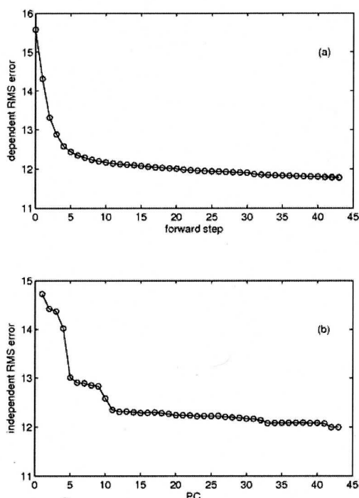
Figure 2: (a) Evolution of dependent RMS error during forward stepping procedure. (b) Evolution of independent RMS error as the new rotated predictors are added. The rotated predictors are the principal components of the original predictor suite. They are ordered in terms of variance explained of the original predictors.
