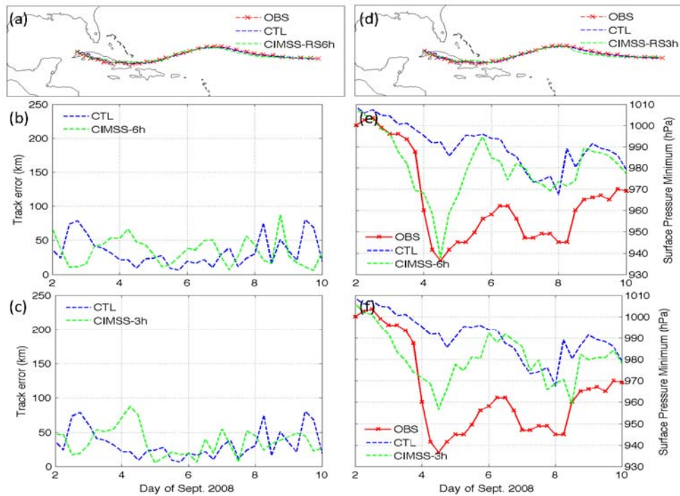
Figure 3: Analyses for Hurricane Ike, for (a-c) 6-hour intervals and (d-f) 3-hour intervals. The graphs represent analysis differences (not forecasts) at these intervals for 8 days of the experiment. NHC Best Track data is used in the validation.
