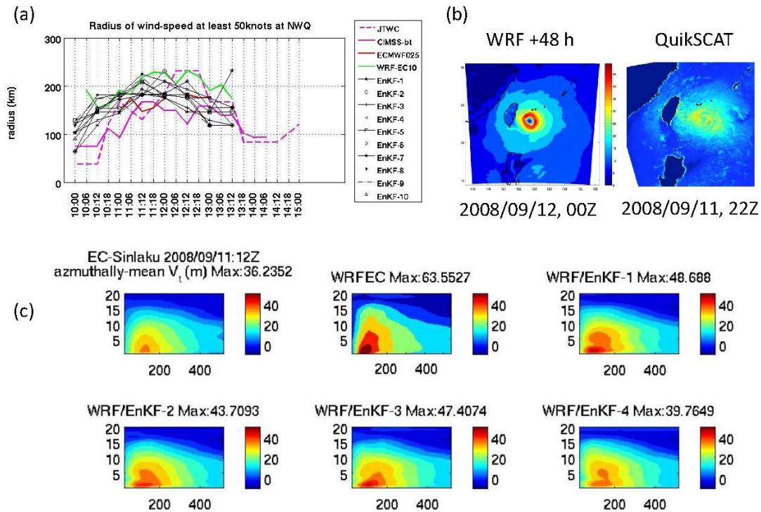
Figure 4: (a) Radius of 50 kt winds in the northwest quadrant of Typhoon Sinlaku, between September 10-15 2008, for ten members of the WRF/EnKF analysis, a high-resolution WRF forecast (WRF-EC10), the ECMWF analysis, and best tracks from JTWC and CIMSS. (b) Surface wind speed for 48-h WRF forecast and QuikSCAT-BYU. (c) Vertical cross-sections of azimuthally averaged tangential wind speed, for the ECMWF analysis, 2-km resolution WRF (WRFEC), and four WRF/EnKF analyses.
