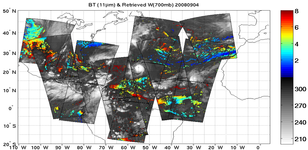
Figure 1. Clear sky 700 hPa AIRS SFOV water vapor mixing ratio (color) overlaid on 11 \mu m IR image (B/W), for (a)Typhoon Sinlaku on 10 September 2008 and (b) Hurricane Ike on 04 September 2008. Each color pixel provides vertical temperature and moisture soundings.
