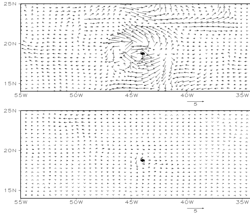
Figure 2: Hurricane Ike wind analysis increments using the CIMSS-RS6h AMV dataset (upper panel) vs. control (lower panel) at 300 hPa (m/s) for 12Z Sep 02, 2008.
