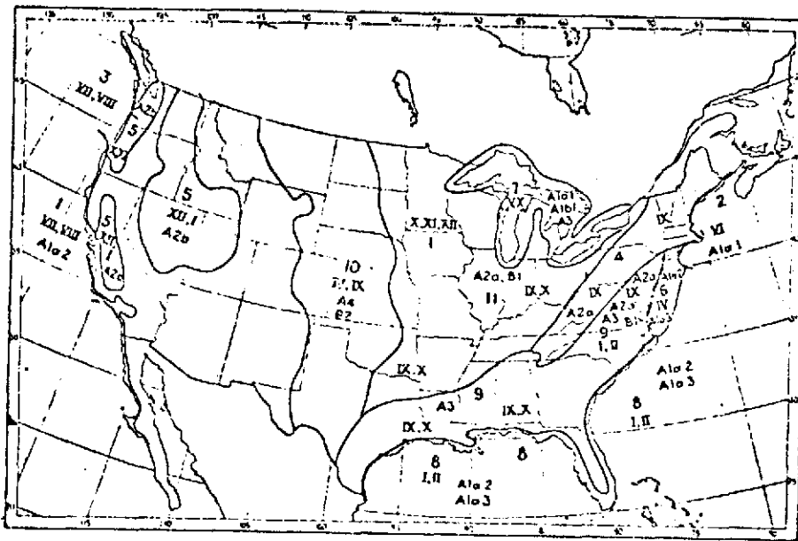
Figure 40. The fog regions of the contiguous United States. Large Arabic numbers correspond to the numbering of the regions as given in this section (e.g., 10 represents Great Plains). The letters and numbers such as A1a2 correspond to the lettering and numbering of the different kinds of fog in the classification at the beginning. The Roman numerals give the month of maximum fog occurrence (I for Jan., II for Feb. etc.)
