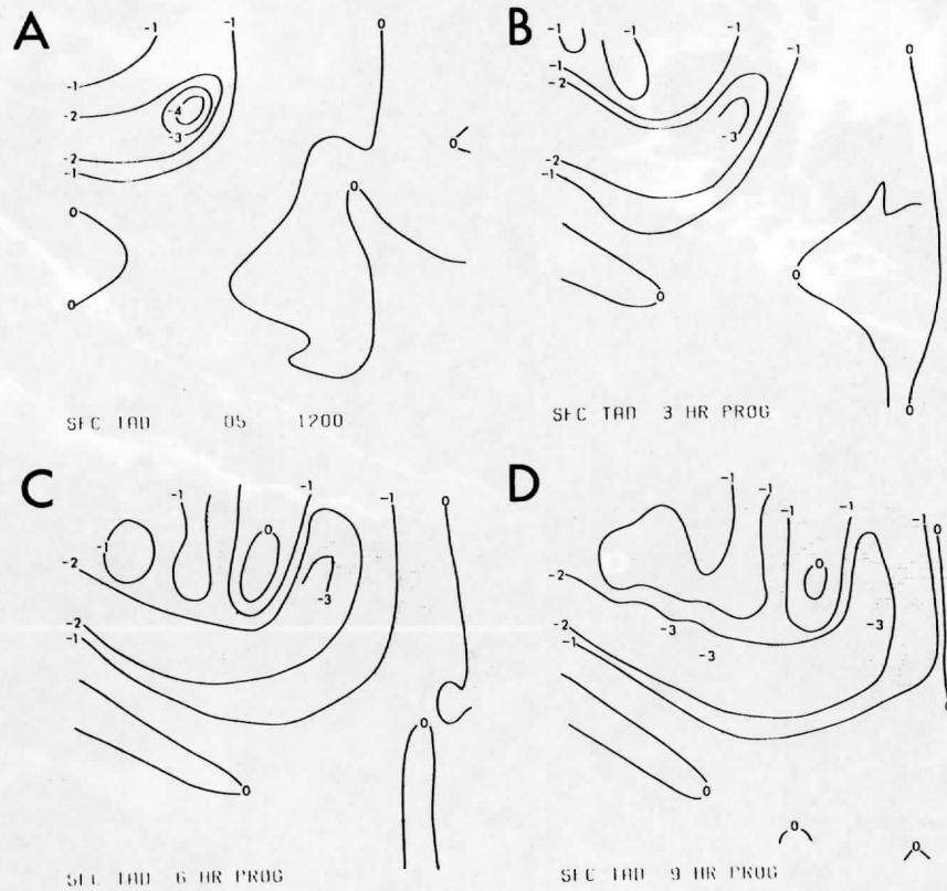
Figure 6. a. Observed surface temperature advection 1200 GMT 5 April 1979 (10°C day -1 ). b. 3 hour temperature advection forecast. c. 6 hour advection forecast. d. 9 hour advection forecast.
