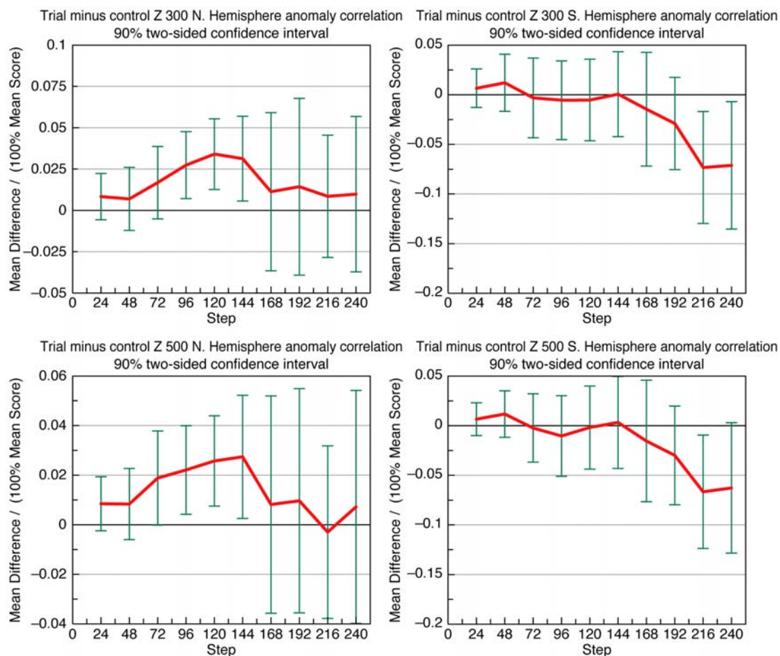
Figure 5: Difference between MET-8 assimilation and control anomaly correlation of height field forecasts. Line marks mean difference and error bars mark 90% confidence region adjusted for one-step autocorrelation.
