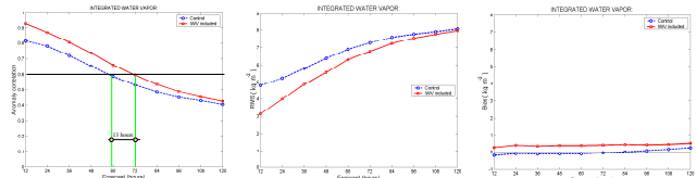
RMS analysis in low and medium levels of the troposphere
