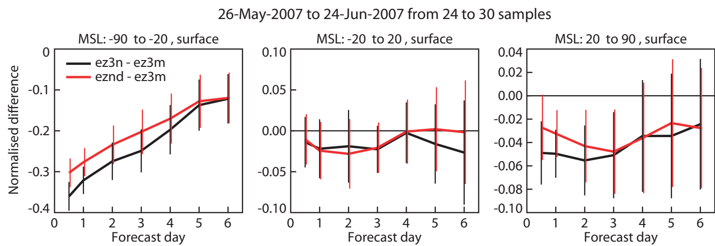
Figure 5 Impacts of normal (black) and noisy (red) AMSU-A data on geopotential height forecasts, relative to an observation 'poor' baseline experiment.
