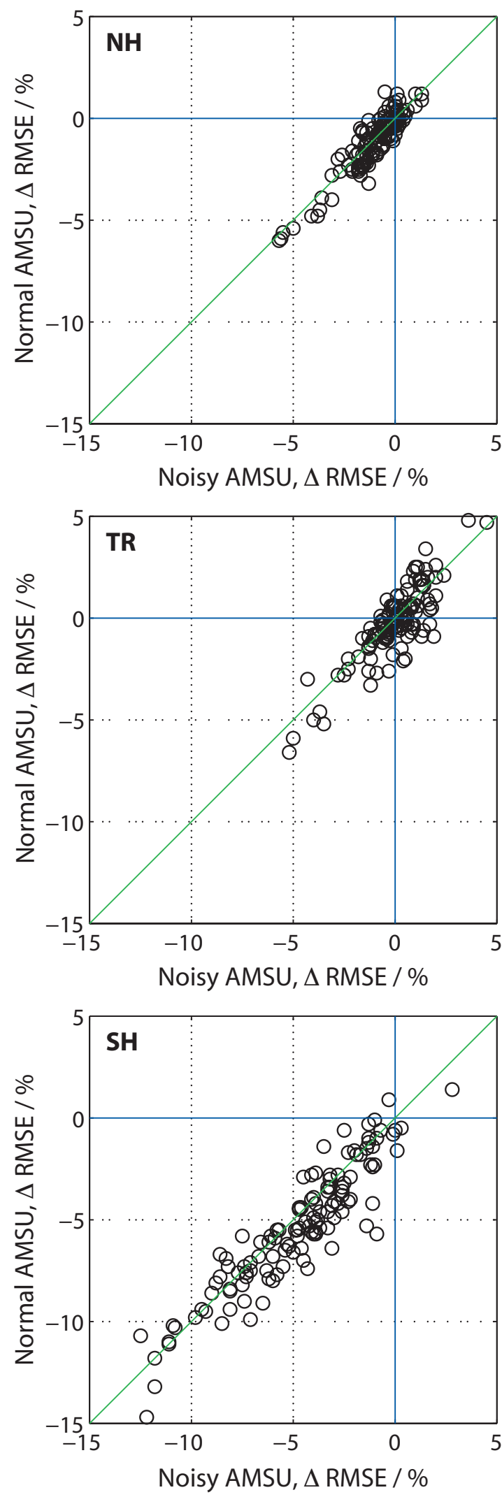
Figure 4 Impacts for an extended group of verification scores in NH, Tropics and SH for normal / noisy AMSU-A.
