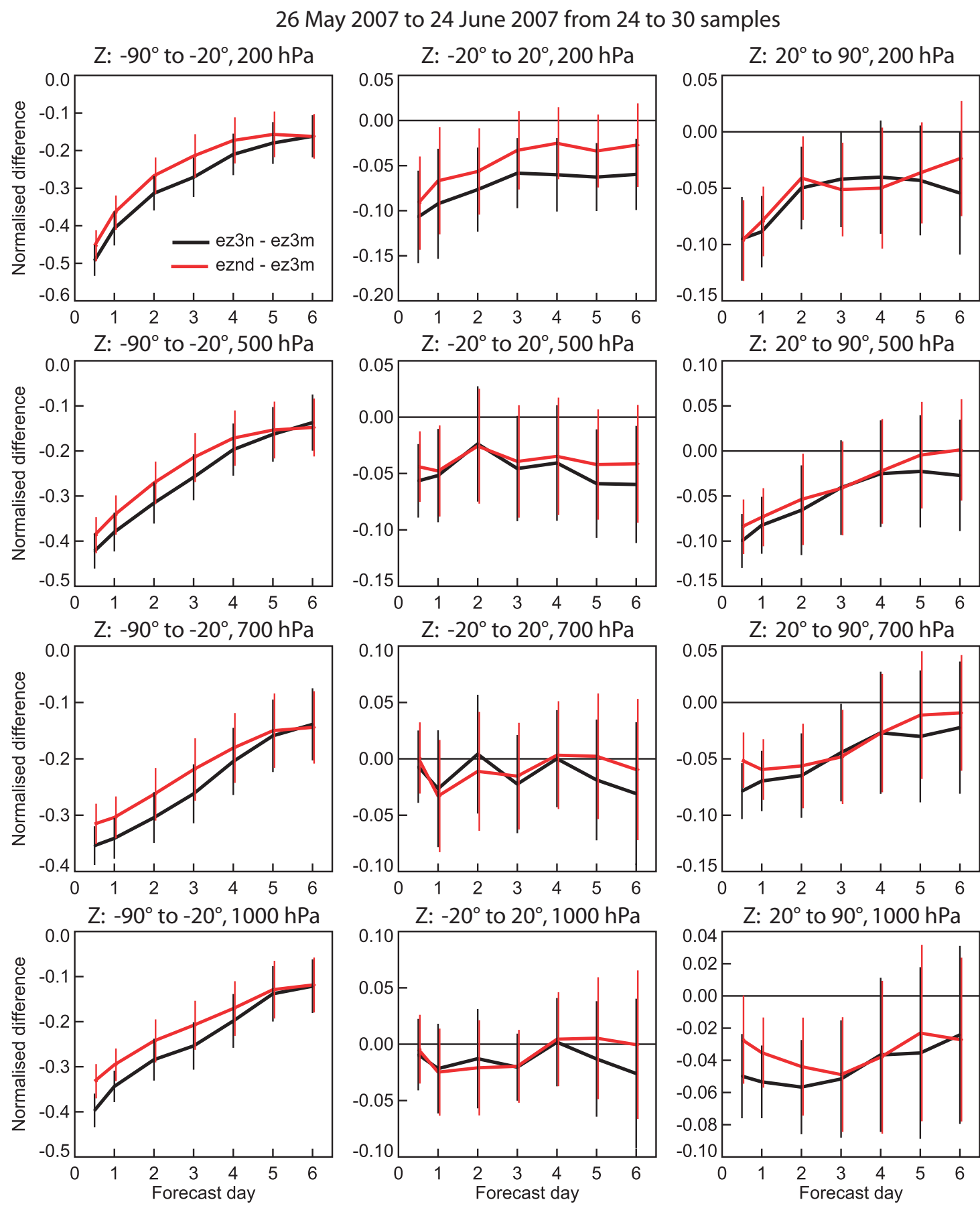
Figure 5 Impacts of normal (black) and noisy (red) AMSU-A data on geopotential height forecasts, relative to an observation 'poor' baseline experiment.
