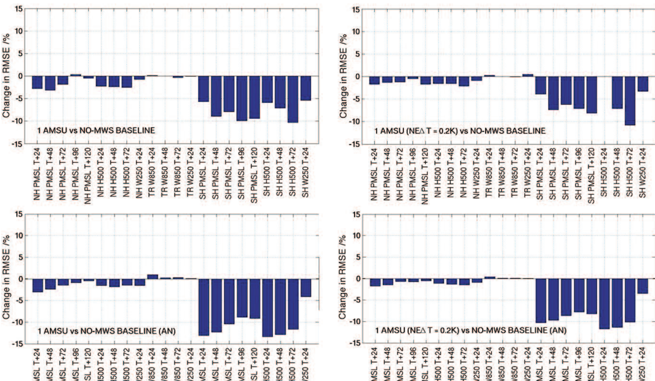
Figure 3 The impact of adding normal / noisy AMSU-A data to a NO MWS data baseline. Verification is derived relative to observations (top plots) and analysis (bottom plots).
