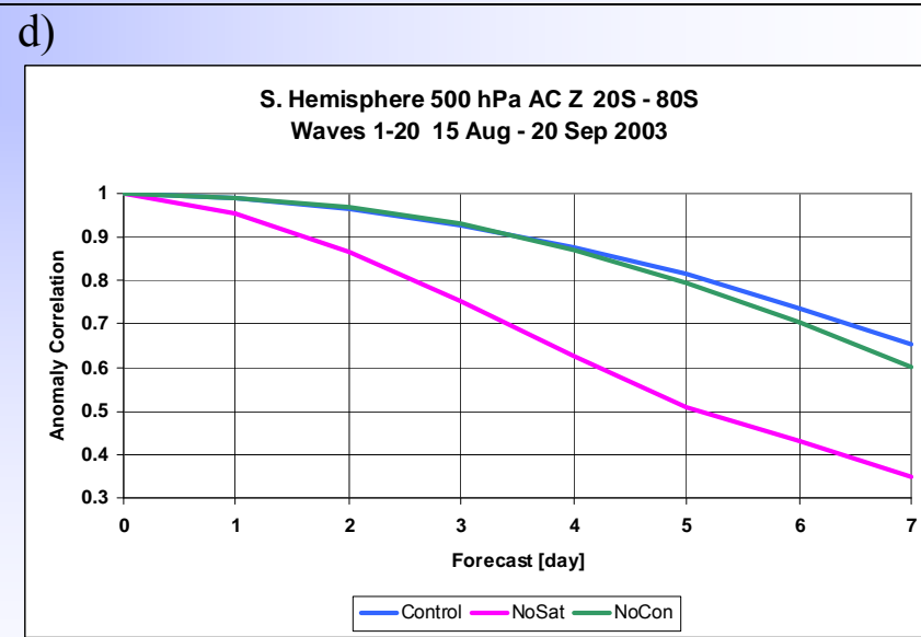
Fig. 6. Anomaly correlation for days 0 to 7 for 500 hPa geopotential height in the zonal band 20°-80° for each Hemisphere and season. The control simulation is shown in blue, while the NoSat and NoCon denial experiments are shown in magenta and green, respectively.
