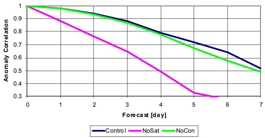
S. Hemisphere 500 hPa AC Z 60S - 90S Waves 1-20 15 Jan - 15 Feb 2003
