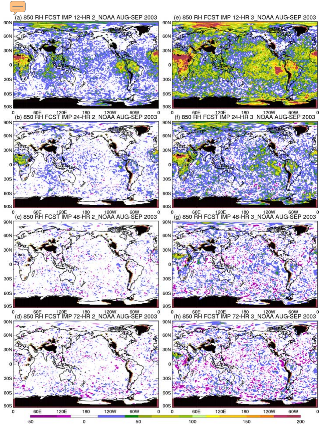
Fig. 15. Geographic distribution of Forecast Impact to 850 hPa relative humidity from the 2_NOAA and 3_NOAA experiments during August-September 2003. The 12, 24, 48 and 72-hr impacts are shown for each time period with the color contour interval 12.5%. Values within 12.5% of zero are white. Regions underground are shaded black.
