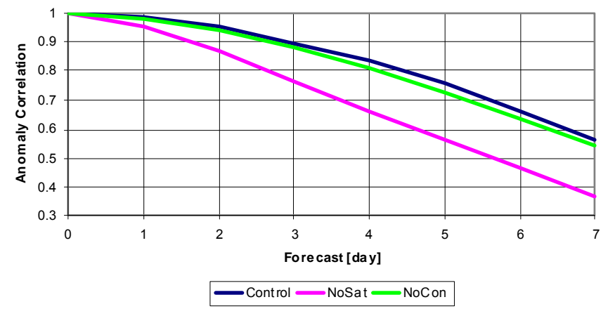
S. Hemisphere 500 hPa AC Z 60S - 90S Waves 1-20 15 Aug - 20 Sep 2003
