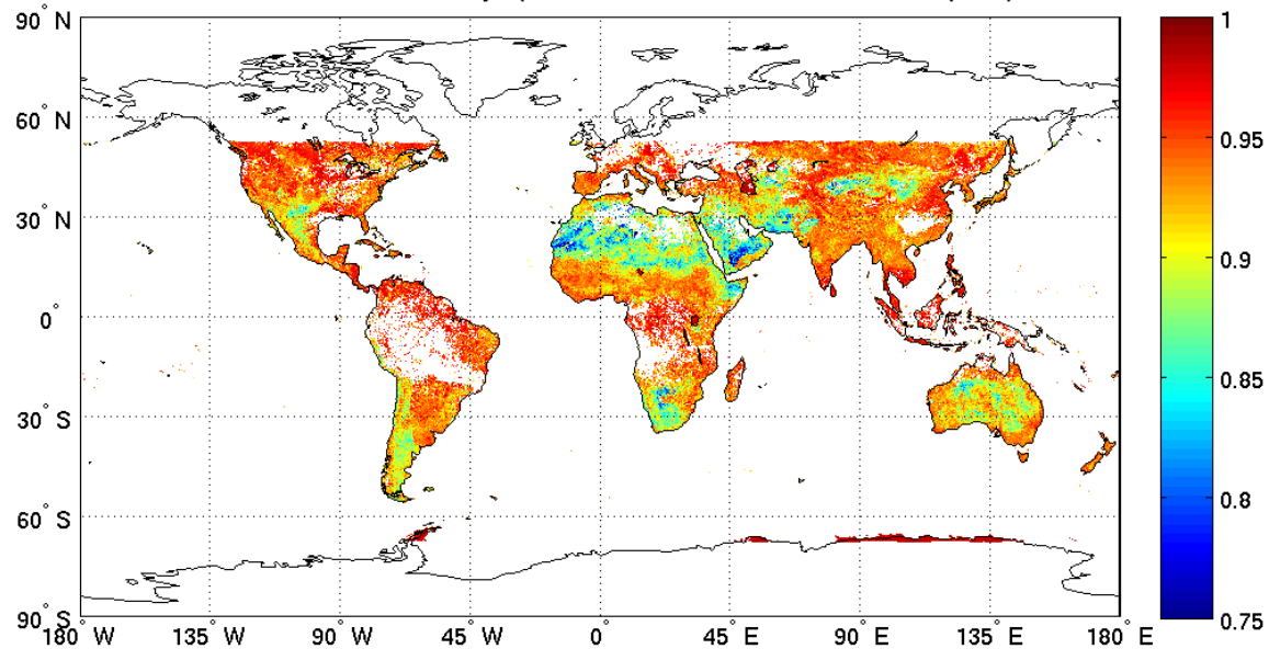
MODIS emissivity (MYD11C2/CH: 23/4.06 \mu\text{m} )
