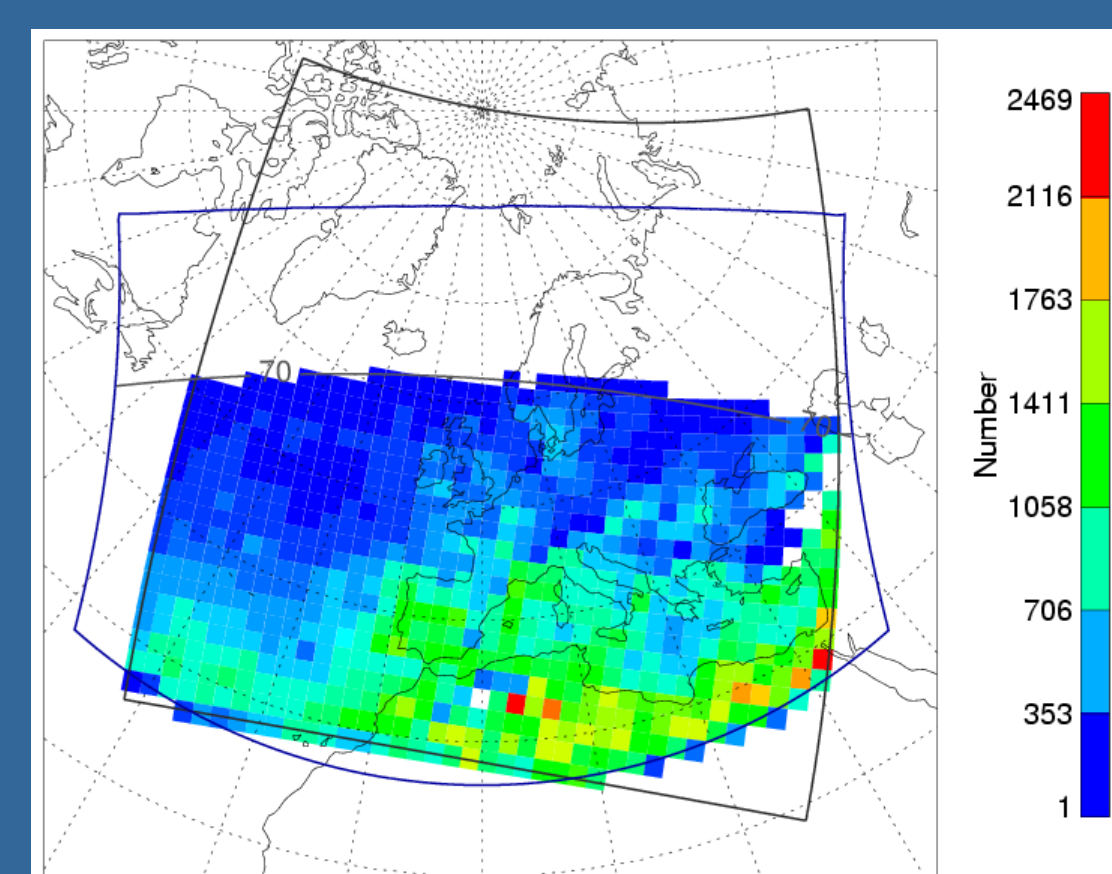
Fig.2: Spatial distribution of used SEVIRI pixels for a one month period with 4D-Var.
