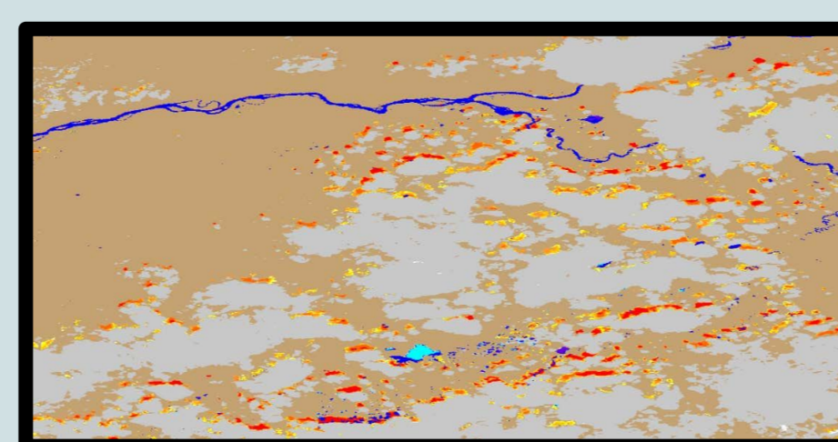
VIIRS flood map without cloud shadow removal, from May 30, 2013 at 22:48 (UTC)
