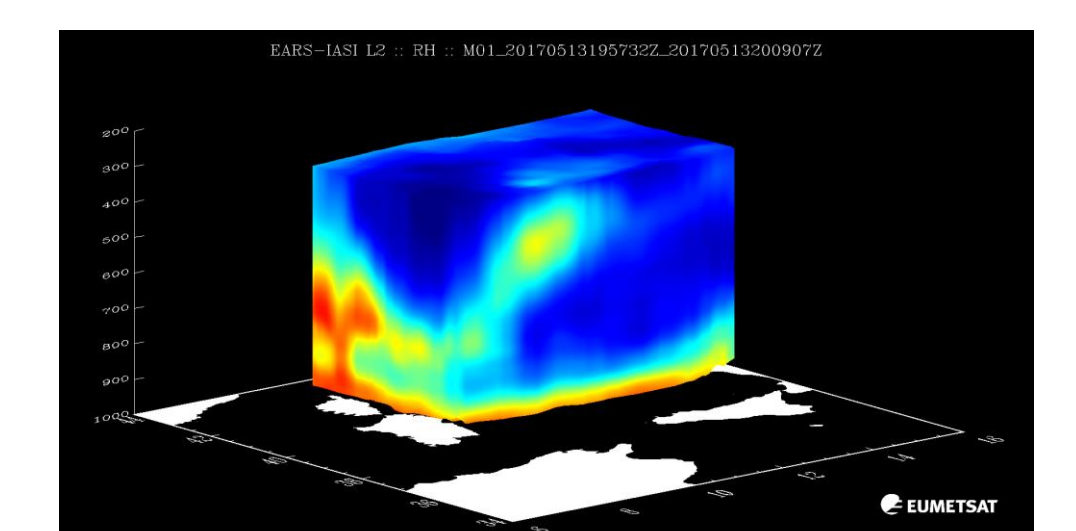
Specific humidity PWLR 3 IASI/AMSU/MHS
