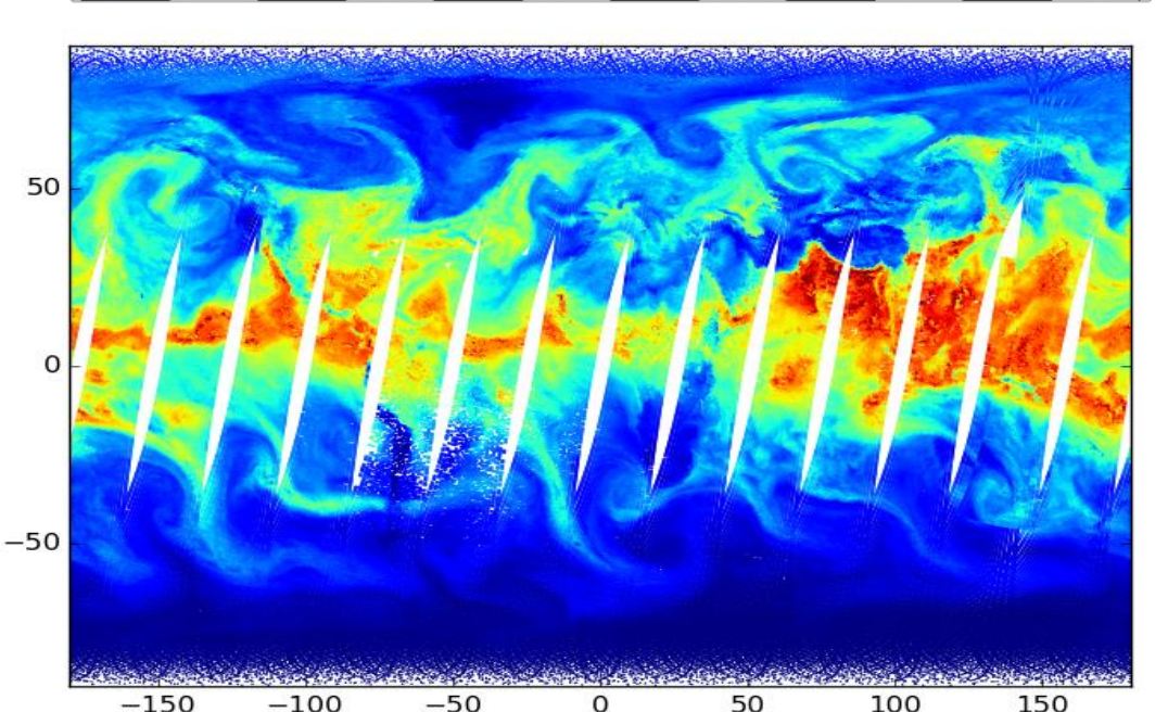
Total column water vapour PWLR 3 IASI/AMSU/MHS
