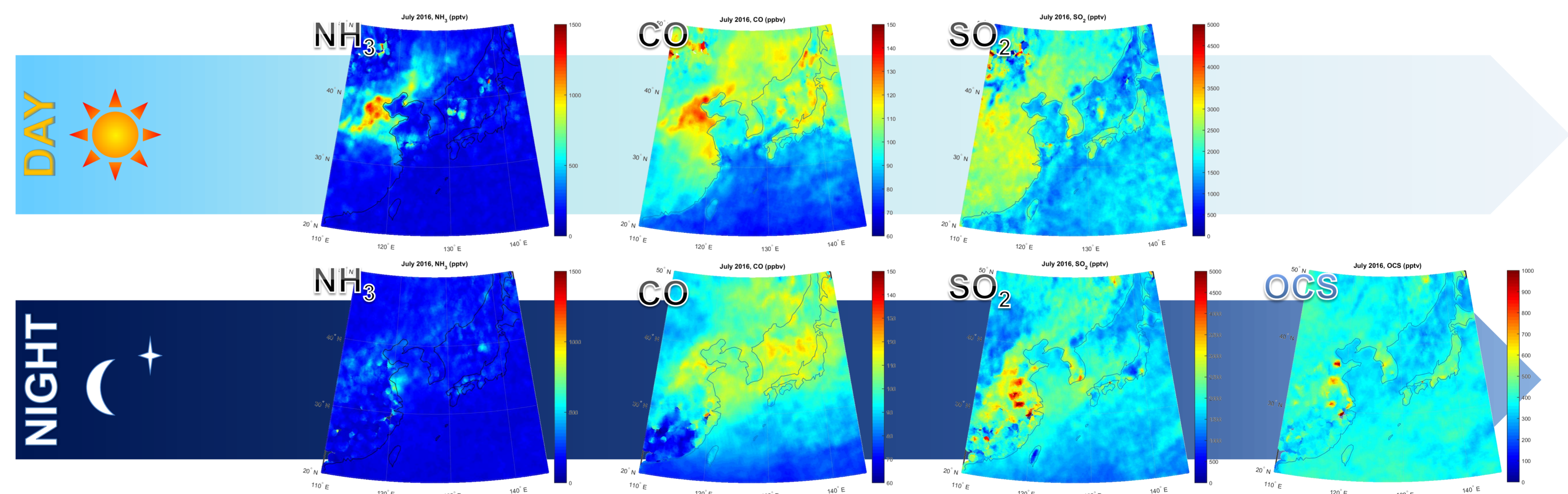
Monthly average maps. Retrieval results have been obtained for the clear sky spectra and averaged over a grid 0.5°x0.5° (~50 km x 50 km)
