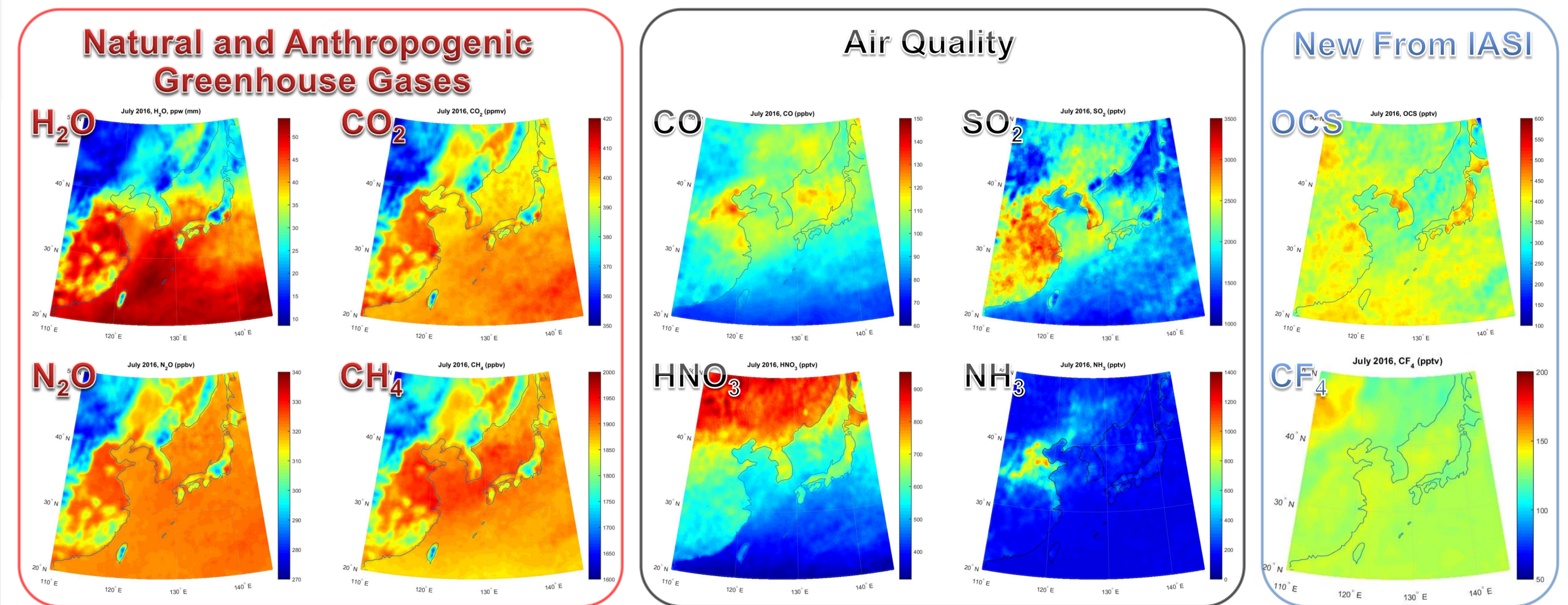
Monthly average maps. Retrieval results have been obtained for the clear sky spectra and averaged over a grid 0.5°x0.5° (~50 km x 50 km)
