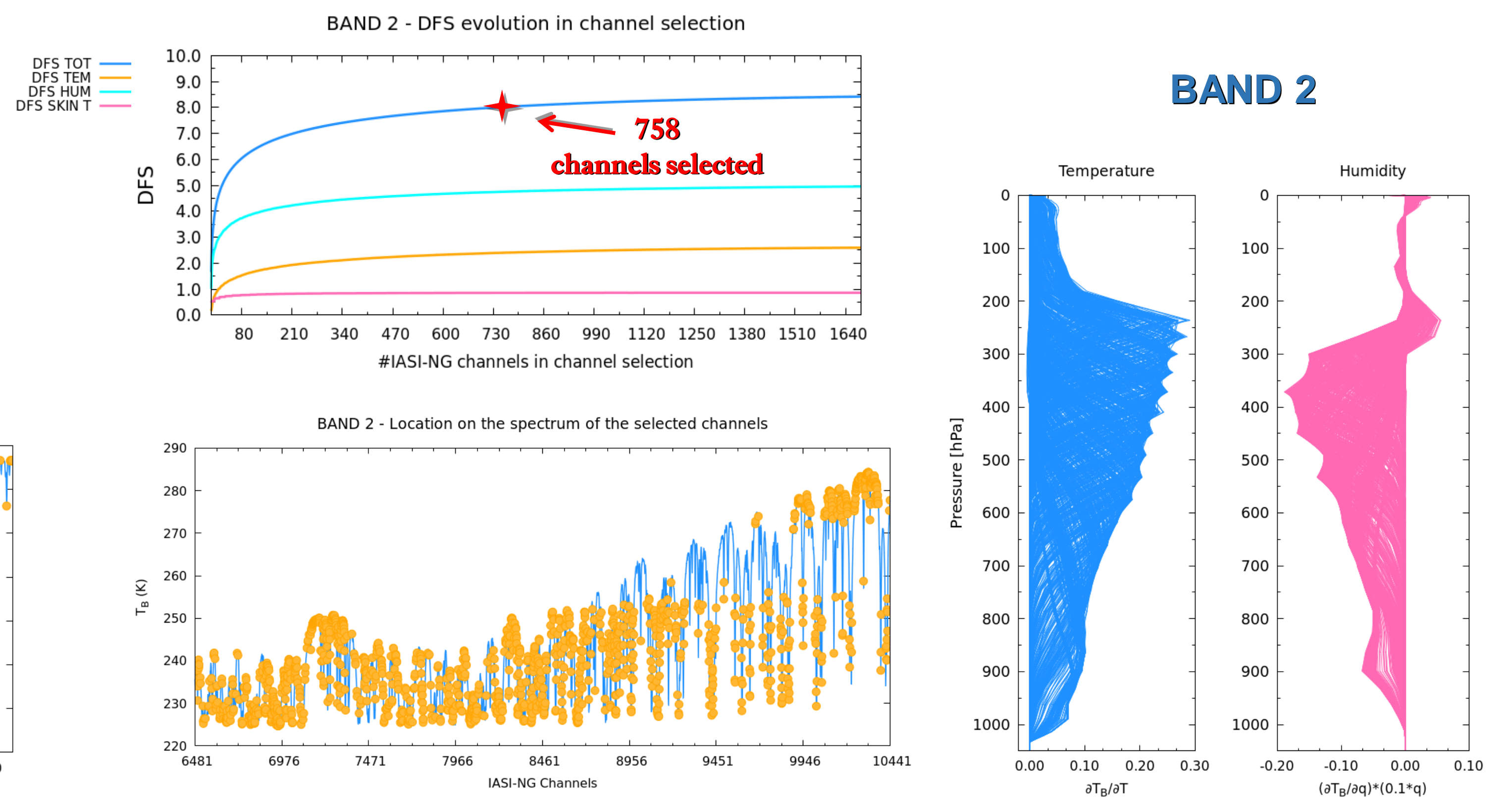
Figure 5: Main channel selection results for BAND 2. Top Left: Total DFS growth with amount of channels selected and contribute of Temperature, Humidity and Skin Temperature DFS. Bottom Right: Temperature and Humidity Jacobians for the 758 channels selected. Bottom Left: position on the spectrum of such 758 selected channels.
