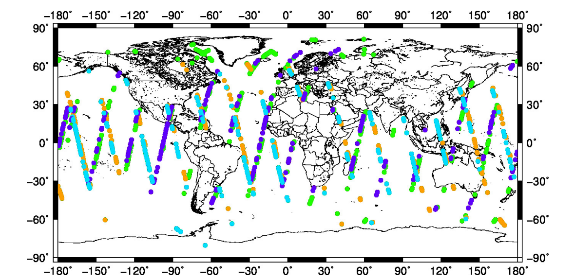
Figure 2: Subset of selected observations for preparing the IASI-NG channel selection: May/day, May/night, August/day, August/night data.
