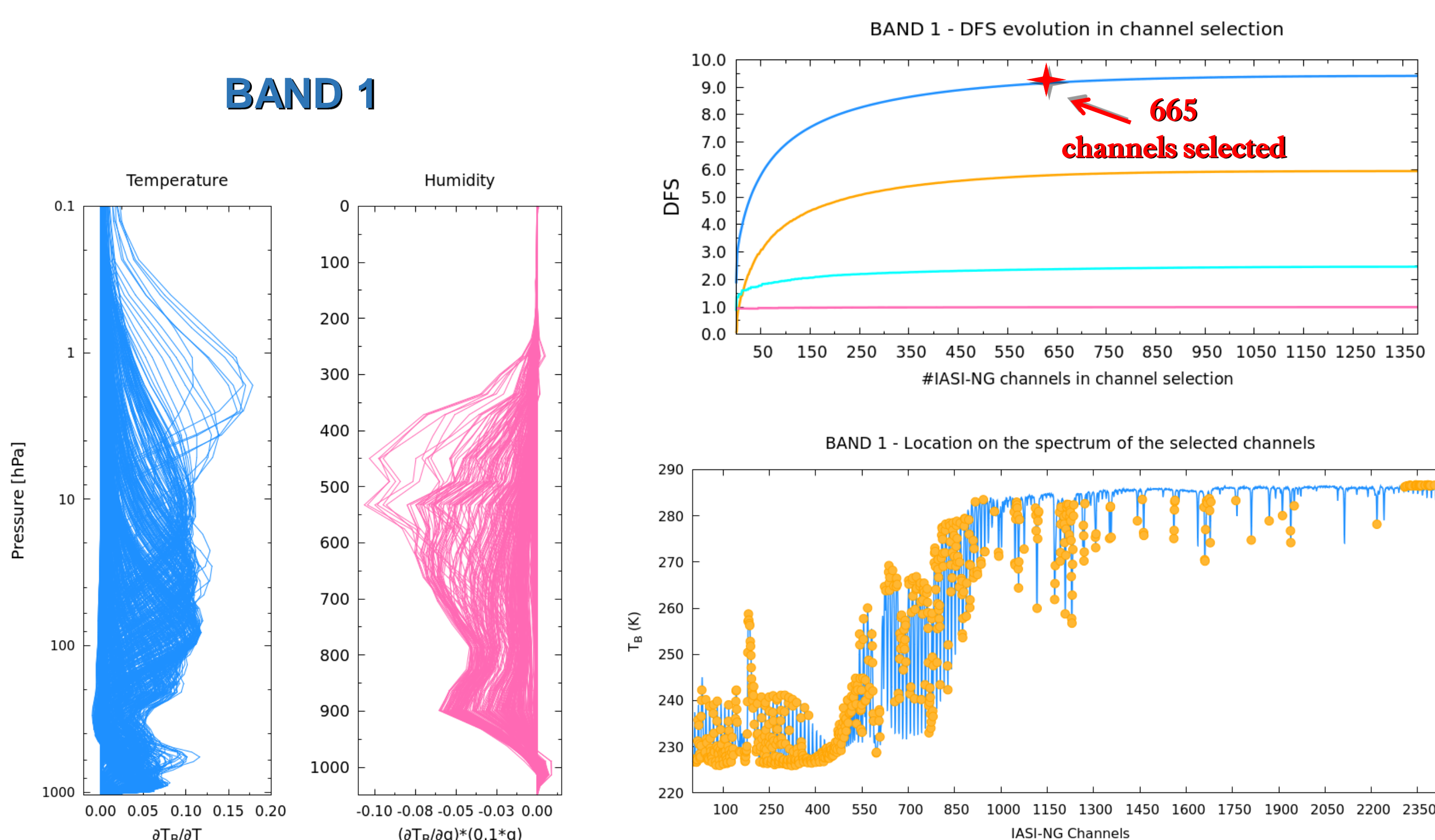
Figure 4: Main channel selection results for BAND 1. Top Right: Total DFS growth with the amount of channels selected (the contribute of Temperature, Humidity and Skin Temperature DFS at each iteration are shown as well). Bottom Left: Temperature and Humidity Jacobians for the 665 channels selected. Bottom Right: position on the spectrum of such 665 channels.
