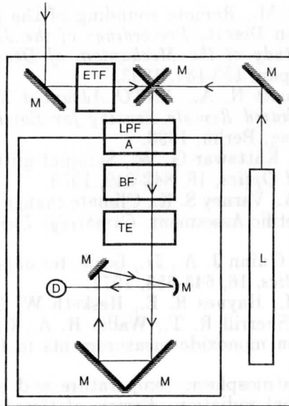
Fig.3 Block diagram of ground-based TERSE, where ETF is the etalon, BF is the interference filter, TE is the tunable etalon and L is the HeNe laser.
