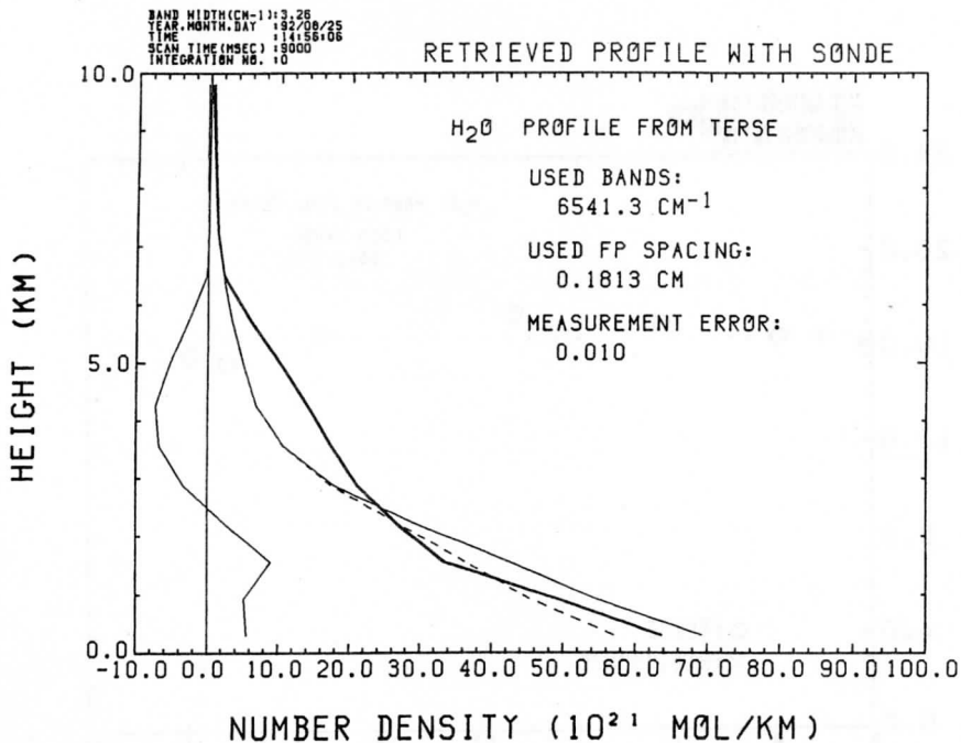
Fig.6 Comparison between retrieved vertical profile of water vapor (thin solid line) and sonde observation (thick solid line). The dashed line is the initial profile and the curve on the left hand side is the difference between retrieved and sonde observed profiles. The measurements were made at Tsukuba, Japan.
