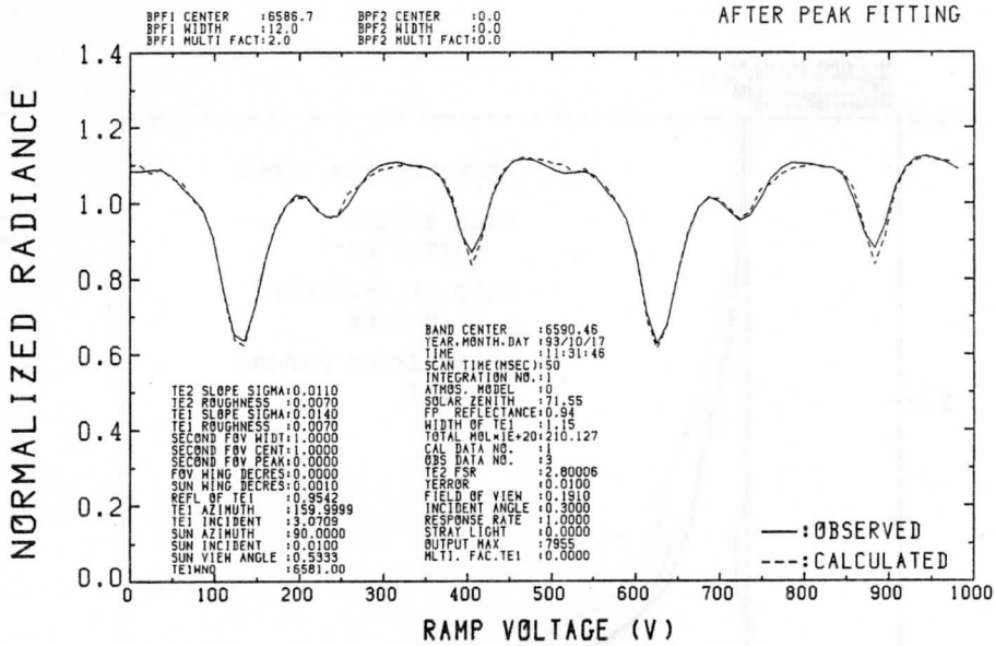
Fig.5 An example of the normalized output of measurement (solid line) with TERSE and calculated one (dashed line). The abscissa is the electric voltage given to the piezo element of the tunable etalon.
