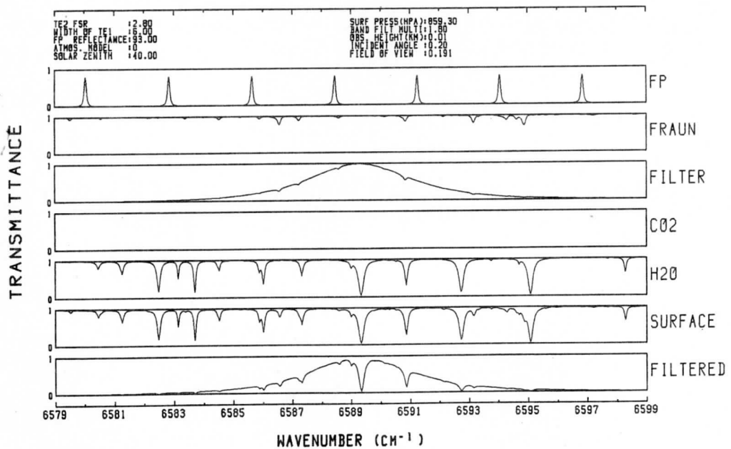
Fig.4 Spectra of the wavenumber region for the H 2 O sounding. The lowest two panels are the transmittance of the column atmosphere (the bottom panel is the filtered), the next two are those of the H 2 O and CO 2 , respectively. The panel signed as "FILTER" is the transmittance of the band pass filter. The next panel is the relative intensity of the extraterrestrial solar radiation and the top panel is that of the tunable etalon for some value of etalon plate separation.
