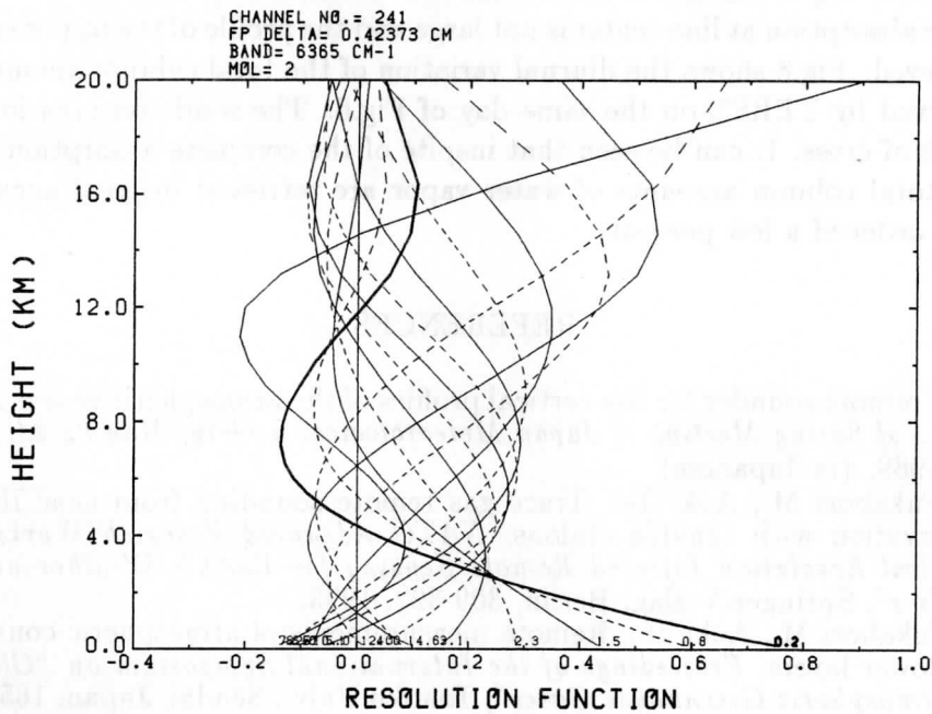
Fig.2 Height resolution function for the sensitivity function shown in Fig.1.
