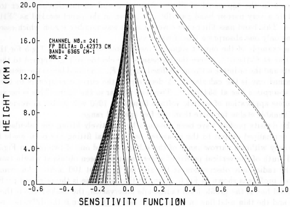
Fig.1 An example of sensitivity function for carbon dioxide sounding by TERSE. The solid and dashed lines are alternately used for easy look.
