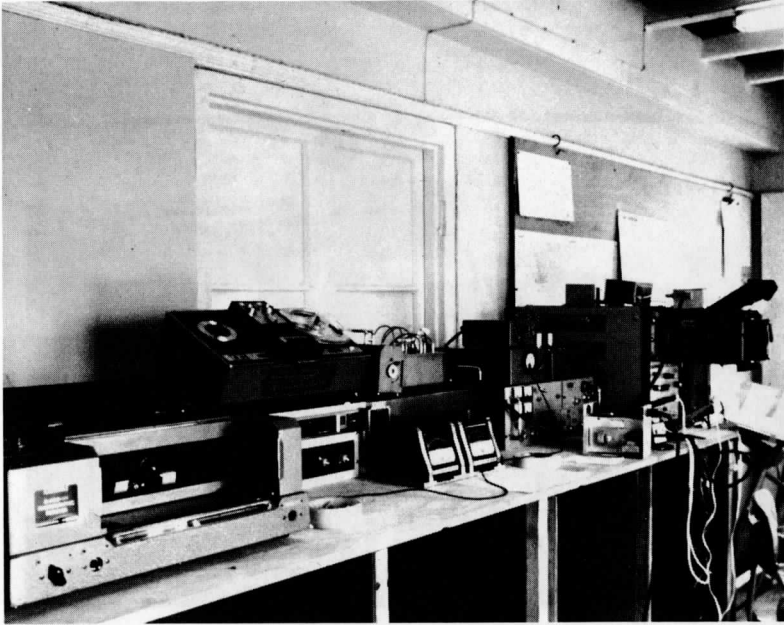
Figure 11. The University of Wisconsin satellite receiving system installed in the BOMEX operations building on Barbados. This equipment was operated during May, June and July, 1969, received the passing satellite data and stored them on magnetic tape. The data were played back on a photo recorder to produce the final satellite picture. These satellite pictures served as the basis for real time decisions on sending aircraft into the BOMEX array.
