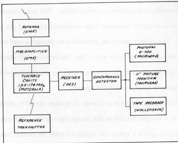
Figure 12. Block diagram of the satellite data receiving system installed on Barbados.
