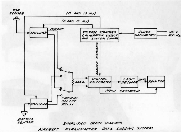
Figure 8. Block diagram of the aircraft pyranometer data logging system which was used on three RFF aircraft to record the data from the Epley pyranometers of the Wisconsin Radiation Experiment.
