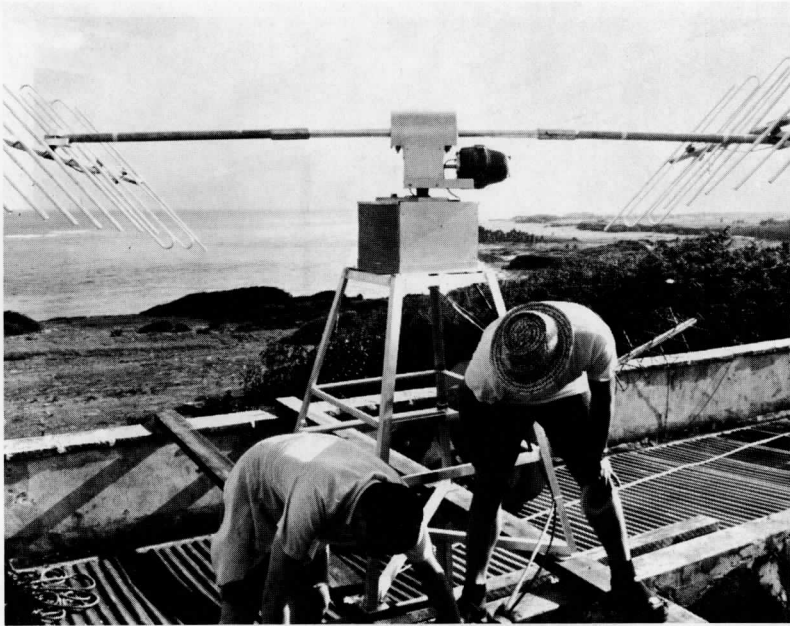
Figure 10. The APT (satellite receiving) antenna being installed on the BOMEX Operations Building on Barbados during May, 1969. This antenna is remotely controlled by operators within the building using computer computations of the orbital position of the satellites. The ESSA satellites in 0900 and 1500 local time orbits were read-out daily, as well as the NIMBUS III satellite at noon and midnight local time. Pictures were also received from the ATS-III satellite which was nearly stationary over Barbados but drifting slowly eastward during the BOMEX observation period.
