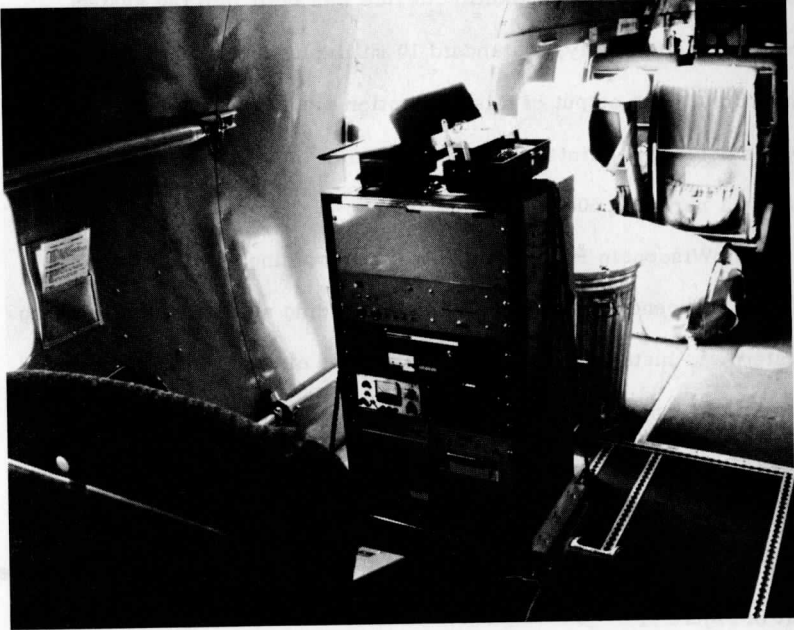
Figure 9. The data logging system for the Wisconsin Radiation Experiment installed on an RFF DC-6 aircraft.
