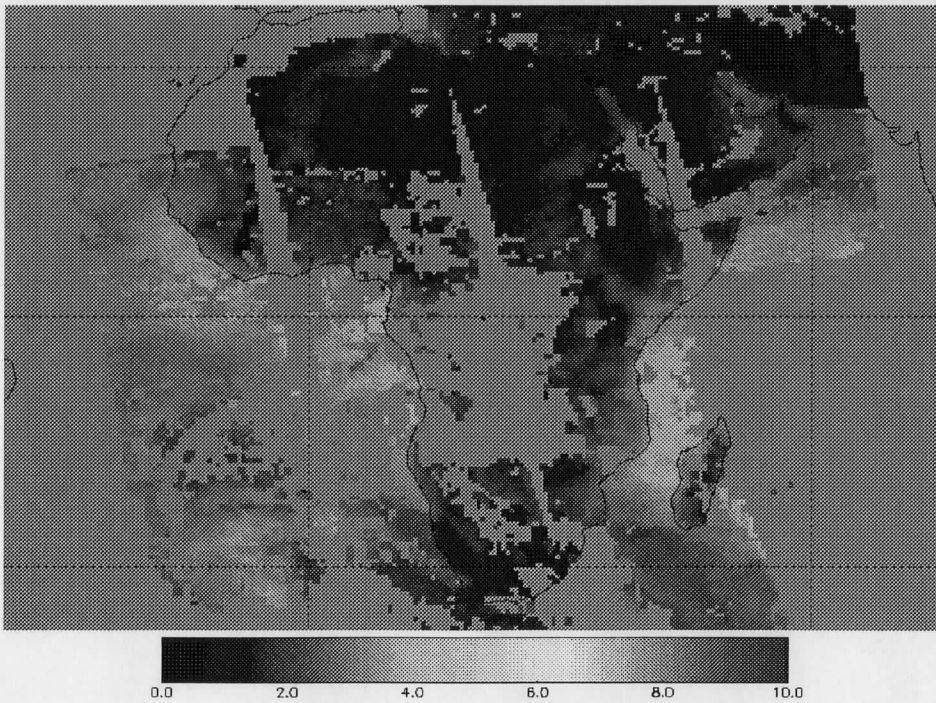
Figure 3: The nighttime TPW images of 07 December 2000 from MODIS with the current algorithm (upper panel, bands 24 and 25 are included) and the updated algorithm (lower panel, bands 24 and 25 are not included) in the South African.
