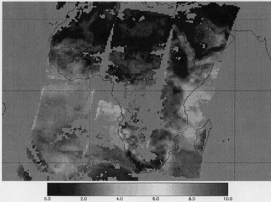
Figure 2: The daytime TPW images of 07 December 2000 from MODIS with the current algorithm (upper panel, bands 24 and 25 are included) and the updated algorithm (lower panel, bands 24 and 25 are not included) in the South African.
