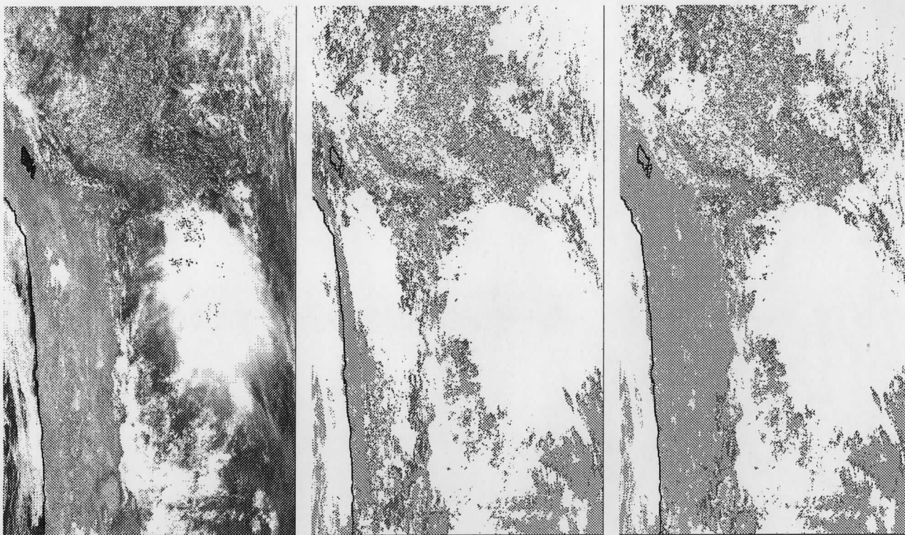
MODIS 0.66 \mu\text{m}
