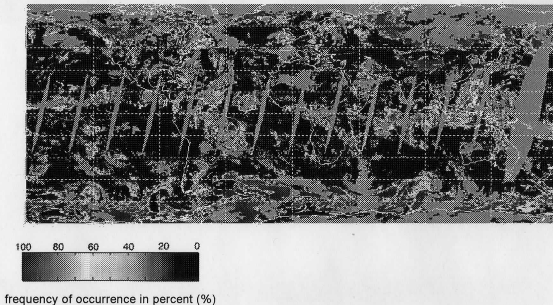
Figure 16: Frequency of the time that a cloud having a cloud top temperature between 253K and 268K is determined to have a water phase, 5 November, 2000 (daytime only).
