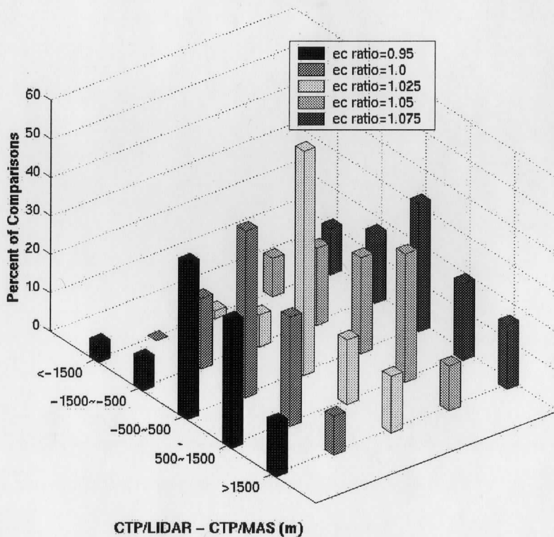
Figure 20: Comparisons of cloud top heights between from CLS and the MAS CO 2 slicing algorithm with different cloud emissivity ratio adjustments [0.95, 1.0 (no adjustment), 1.025, 1.05, and 1.075]. The MAS data is from single layer clouds and cloud top heights are greater than 4000 m on track 14 on April 16, 1996.
