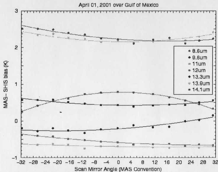
Figure 10: MAS-SHIS residuals as a function of scan angle for the LWIR spectral region. See Figure 9 for spectral band numbers. Most bands display some dependence on the MAS cross track scan mirror angle, which may be due to MAS scan mirror polarization sensitivity. The 8.6µm band (42) dependence stands apart from other bands with a large negative influence moving from nadir to limb across the scan swath.
