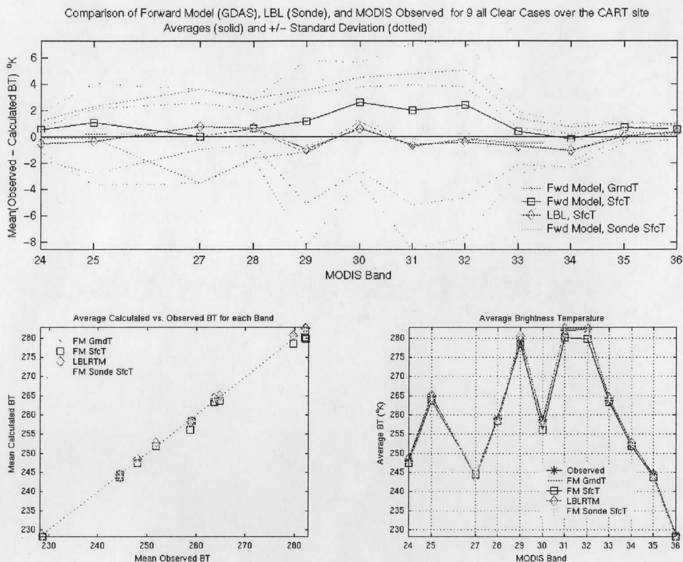
Figure 19: Average brightness temperature comparisons for 9 clear-sky cases over the CART site.
