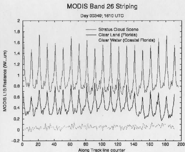
Figure 6: MODIS band 26 ( 1.38\ \mu\text{m} ) along track radiance profiles for three scene types. Striping appears to be non-existent over the clear ocean scenes south of Florida, while it quickly amplifies in the higher signal levels associated with land and cloud scenes. Striping is also evident in ocean scenes with sunglint (not shown). The 10–15% amplitude of striping is causing the MODIS Cloud Mask to determine false cloud in clear land scenes.
