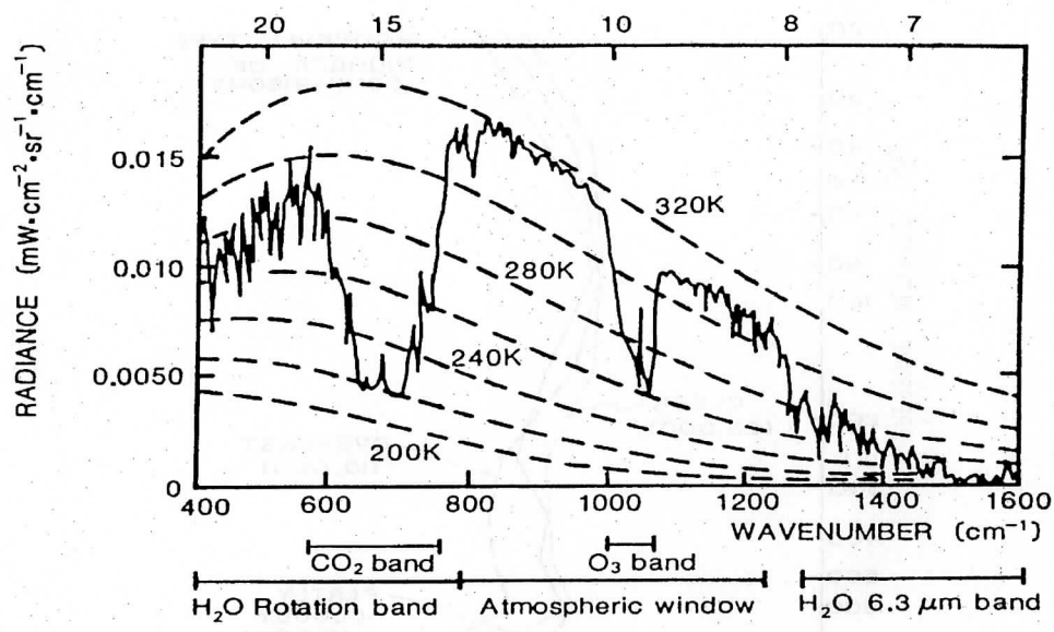
Figure 1.1. Infrared portion of the earth-atmosphere emitted radiation to space observed from Nimbus 4. Planck emission and line spectra are indicated.
