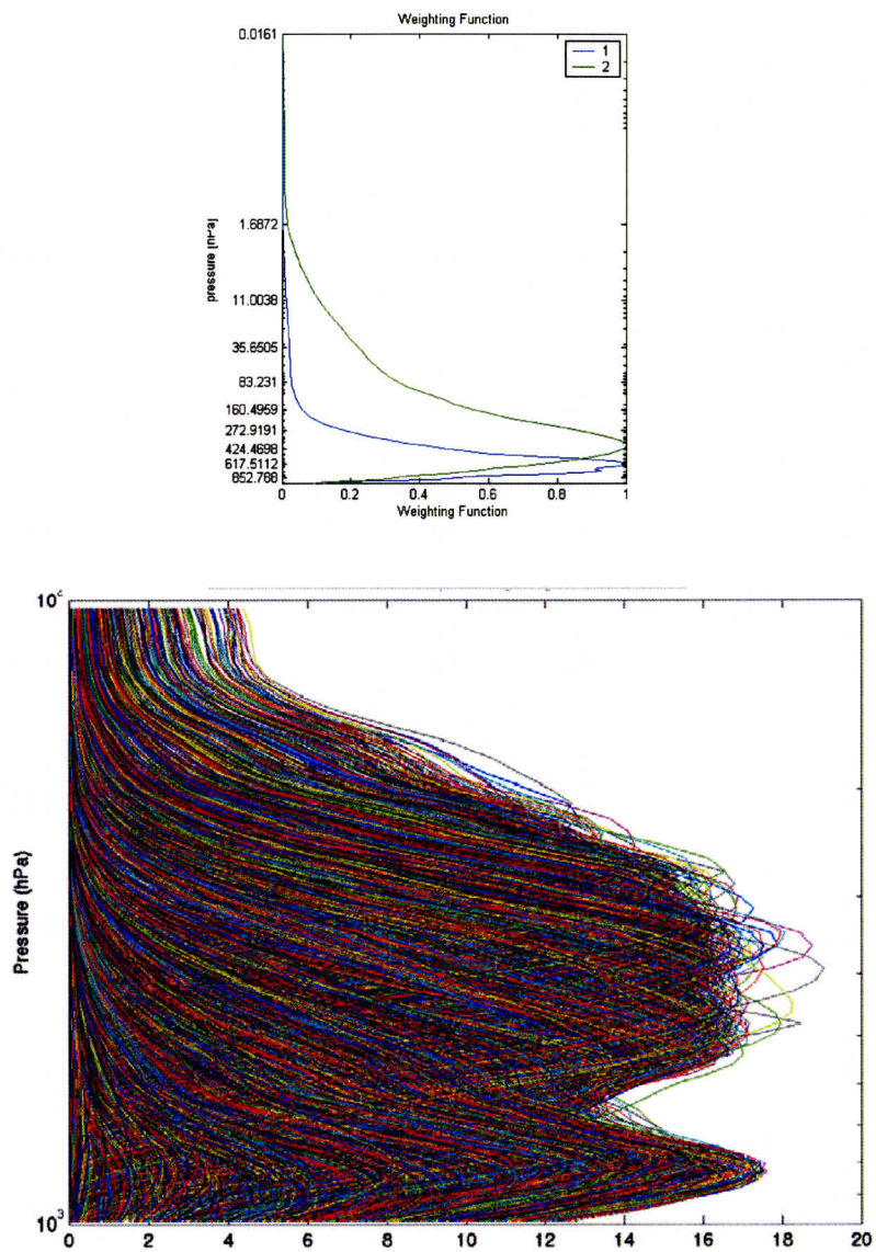
Figure 16.4. (top) Two weighting functions associated with off-line and on-line measurements at 735 \text{cm}^{-1} . Off-line peaks near 600 hPa while on-line peaks near 400 hPa; a small spectral shift changes the weighting function (and hence the radiance contribution significantly). (bottom) The weighting functions associated with roughly 3000 high spectral resolution micro-channels for a standard atmosphere.
