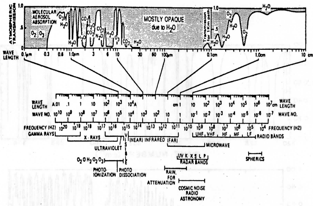
Figure 3.8a: Atmospheric transmission characteristics showing the major absorption bands.
