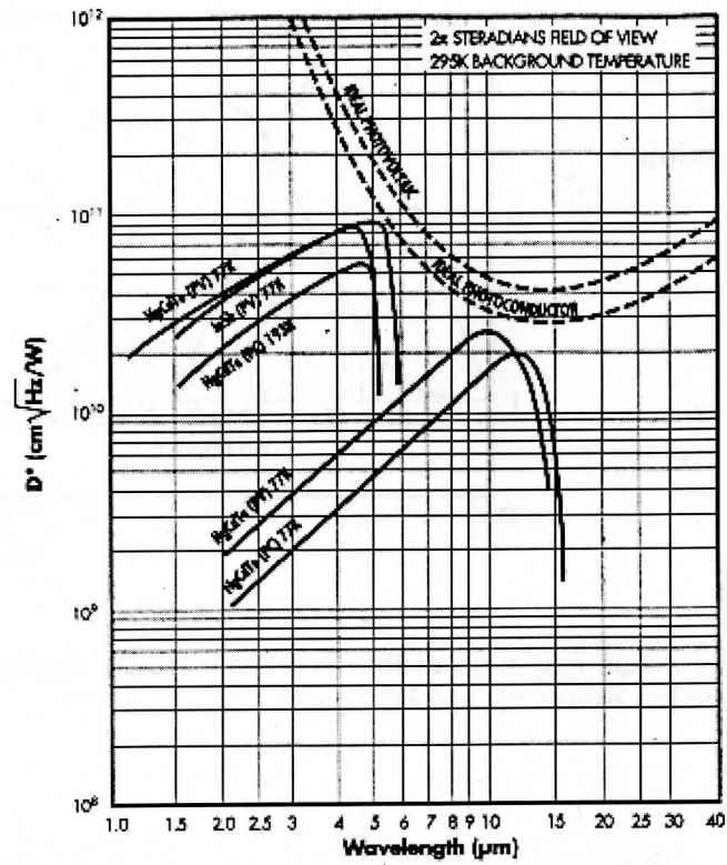
Figure 12.5: Detectivity of InSb and HgCdTe detectors as a function of spectral region.
