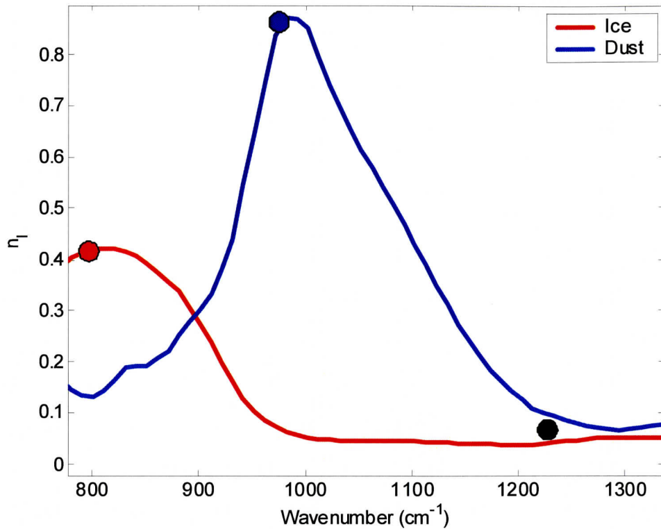
Figure 16.11. The imaginary index of refraction (related to the absorption) of ice and dust. Note between 850 and 950 \text{cm}^{-1} the absorption of ice decreases while for dust it increases. And between 1080 and 1120 \text{cm}^{-1} the absorption of dust decreases. These characteristics of the absorption are apparent in the measured spectra when viewing ice and dust.
