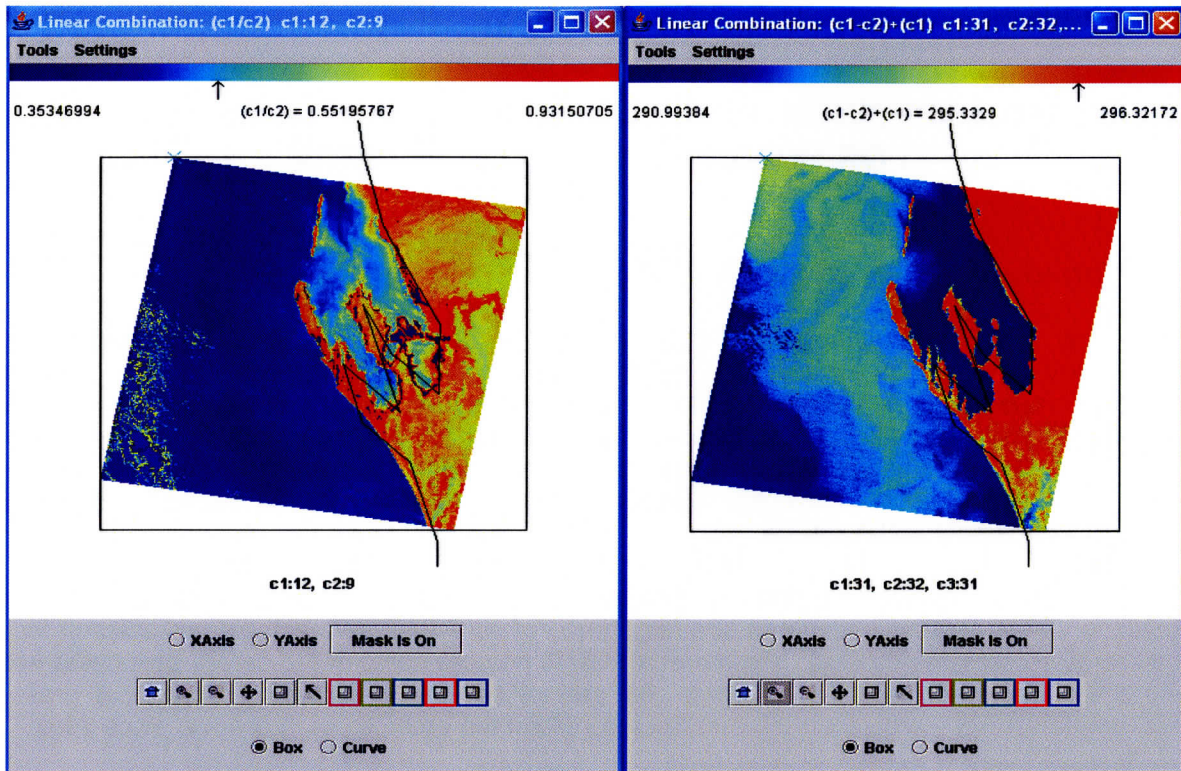
Figure 15.22: (right) Image of sea surface temperature estimated by [2*BT(11)-BT(12)] showing waters within Shark Bay (blue) are about 4 C cooler than the Leeuwin current waters (turquoise) along the WA coastline. (left) Image indicative of chlorophyll concentrations in Shark Bay estimated by band 12 ( 0.57\mu\text{m} ) / band 9 ( 0.44\mu\text{m} ) where high ratio values are an indication of more chlorophyll.
