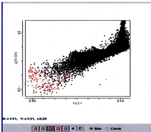
Figure 15.14: Scatter plot (left) of [BT31 (11 \mu\text{m} )] on the x-axis and [BT31 (11 \mu\text{m} ) - BT29 (8.5 \mu\text{m} )] on the y-axis. Cloud in BT31 image (right) shows negative [BT31-BT29] values in scatter plot, suggesting ice cloud.
