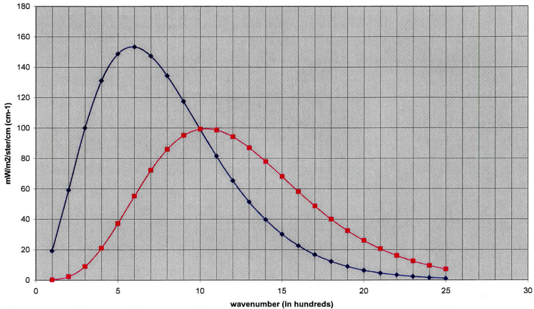
Figure 2.4: Planck radiance curves at 300 K. Wavenumber are given in units of 100 \text{cm}^{-1} ; the corresponding wavelengths in cm are determined from the reciprocal of the wavenumber. Purple boxes show B(\lambda, T) in units of \text{mW}/\text{ster}/\text{m}^2/\text{cm} (per unit wavelength) and blue diamonds show B(\nu, T) in units of \text{mW}/\text{ster}/\text{m}^2/\text{cm}^{-1} (per unit wavenumber). B(\lambda, T) is shown multiplied by a factor of 10^{-6} (e.g. B(10 \mu\text{m}, 300 \text{ K}) is 9.9 \times 10^7 ) while B(\nu, T) is shown multiplied by a factor of 1 (e.g. B(1000 \text{ cm}^{-1}, 300 \text{ K}) is 99.0). Note that Wiens law for B(\nu, T) becomes \nu(\text{max}) = 1.95T ( \text{cm}^{-1} ) while the more familiar form for B(\lambda, T) is \lambda(\text{max}) = .2897/T (cm).
