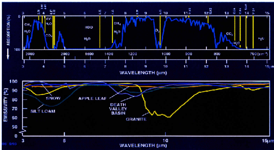
Figure 13.5d: Atmospheric absorption (top) & surface emissivity (bottom) from 3 to 15 micrometers.
