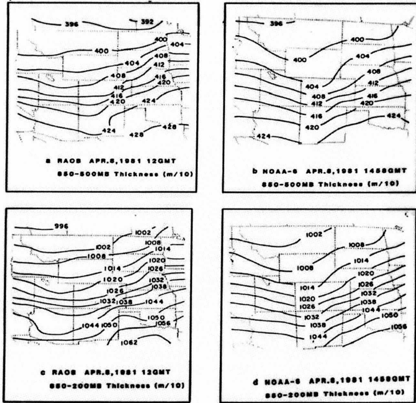
Figure 8.3: Comparison of NOAA-6 MSU estimates of 850-500 and 850-200 mb thickness patterns with those obtained from radiosonde observations.
