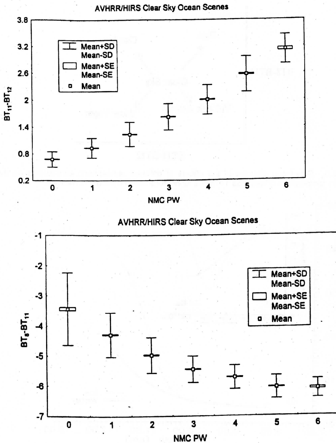
Figure 6.4. The dependence on PW of the brightness temperature difference between the various window channels. Observed AVHRR 11-12 micron (top panel) and collocated HIRS 8-11 micron (bottom panel) brightness temperature differences plotted versus global model (NMC) total column PW for January 1994 over clear ocean scenes.
