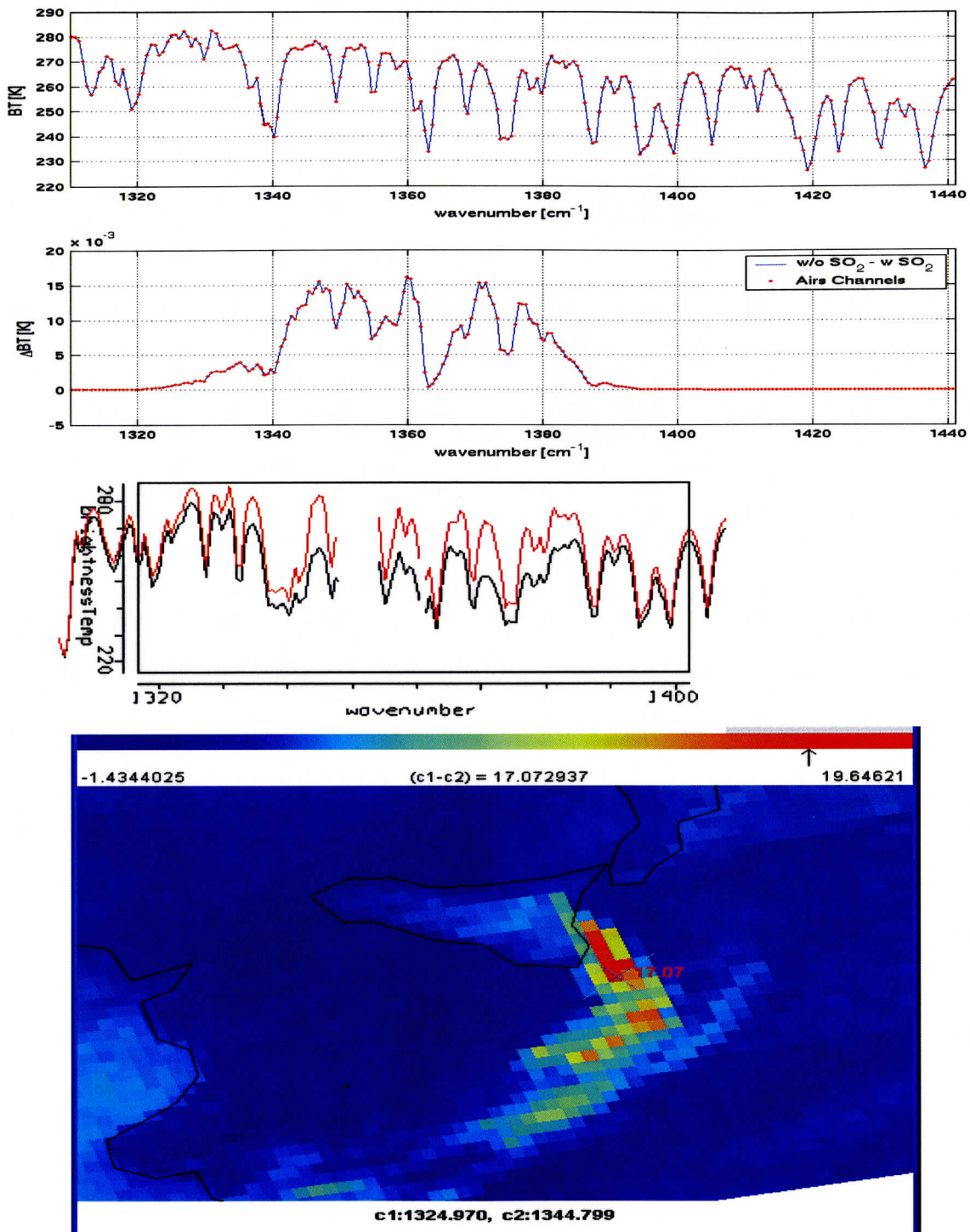
Figure 16.13. The spectral signature of SO 2 between 1320 and 1400 \text{cm}^{-1} (top) offers the opportunity to track volcanic SO 2 emissions. The spectrum for Mt Etna of 28 Oct 2002 (middle) suggests that the brightness temperature difference of 1325 minus 1345 \text{cm}^{-1} (avoiding water vapor absorption lines) effectively maps Volcanic SO 2 emissions.
