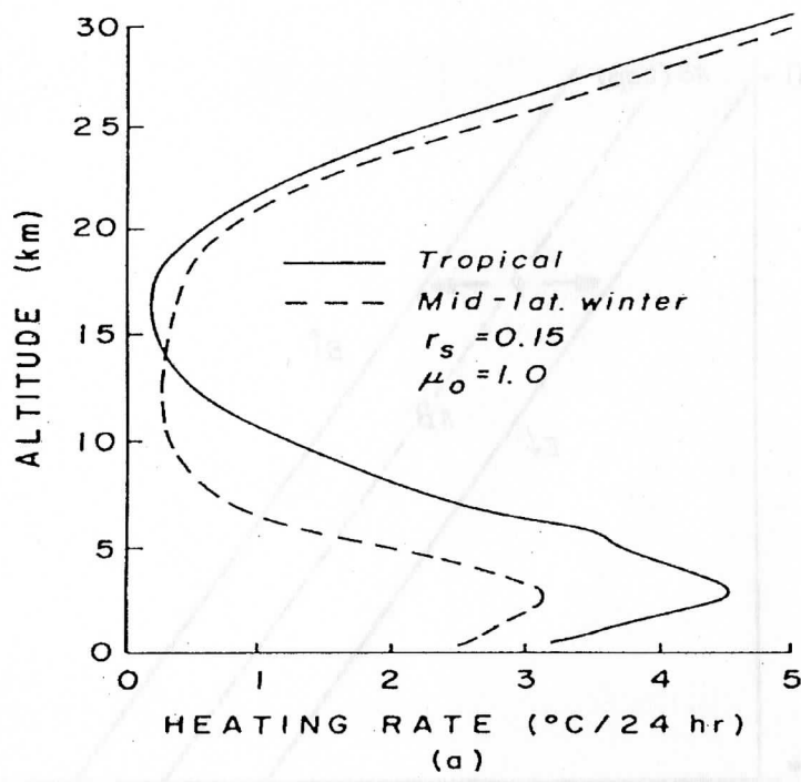
Figure 4.5: Solar heating rate calculated from atmospheric profiles appropriate for tropical and mid latitude winter conditions (Liou, 1980).
