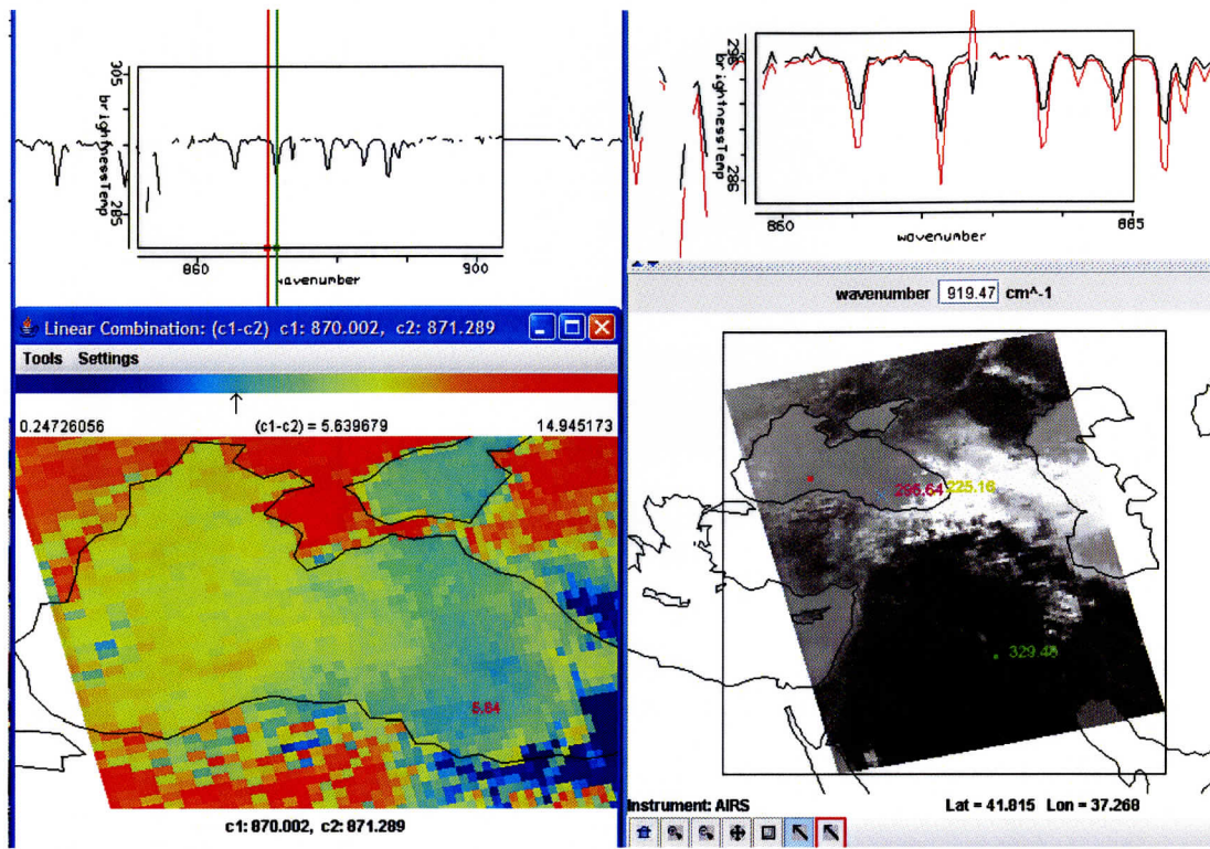
Figure 16.6. (left) Brightness temperature difference of spectral micro-channels at 870.0 cm -1 (off the H 2 O rotational line) minus 871.3 cm -1 (on the H 2 O rotational line). In the western portion of the Black Sea differences are about 9 C while in the eastern portion of the Black Sea they are more like 6 C. There is more low level moisture over the western portion of the Black Sea. (right) The spectra in the window region for the western region (red) show more moisture absorption than the spectra from the eastern region (black).
