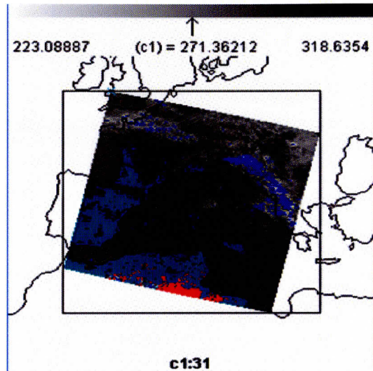
Figure 15.13: Scatter plot (left) of [BT31 (11 \mu\text{m} )] on the x-axis and [BT31 (11 \mu\text{m} ) - BT29 (8.5 \mu\text{m} )] on the y-axis. Negative [BT31-BT29] indicates ice cloud in BT31 image (right).
