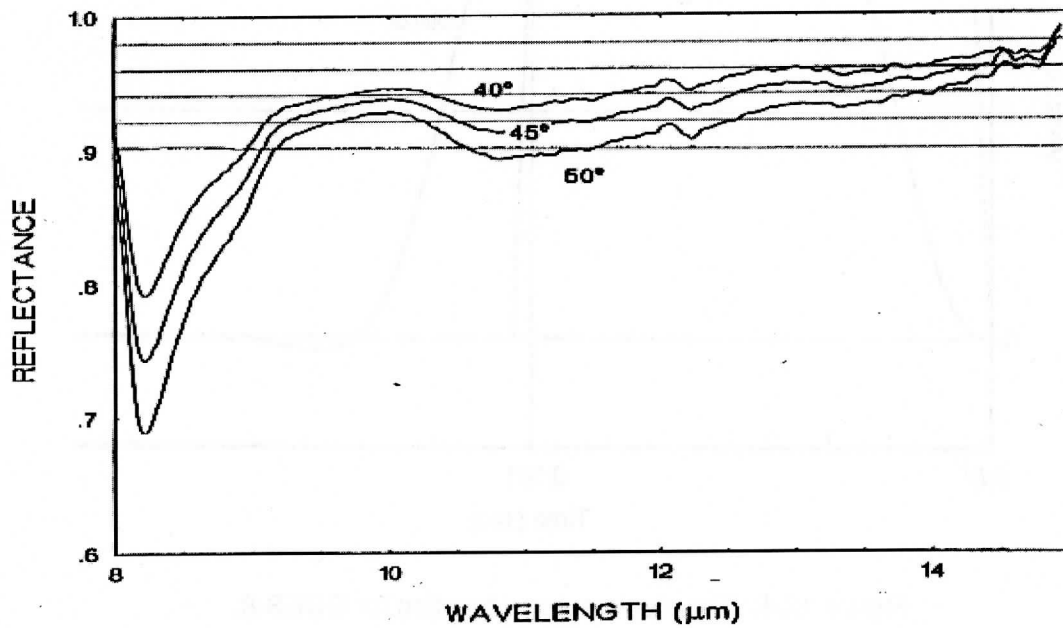
Figure 12.6: Emmissivity changes with angle and wavelength for GOES-8 scan mirror.
