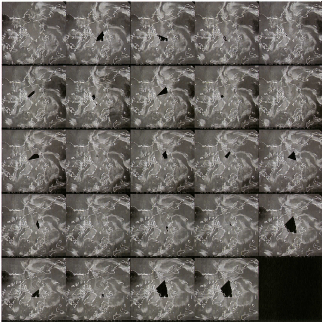
Figure 5. 24 hours of 1-hourly Arctic infrared composites for 25 August 2010.
