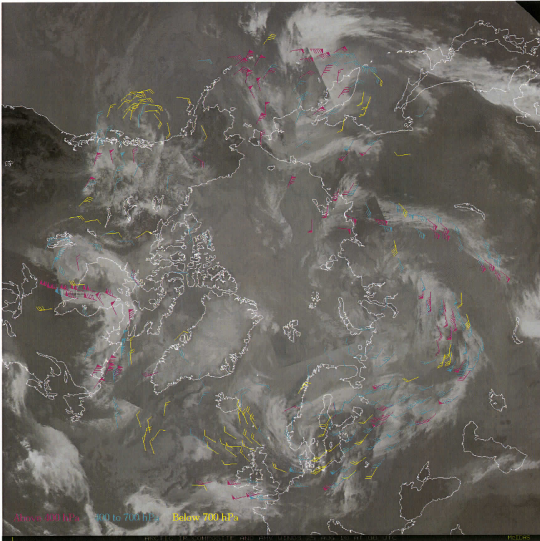
Figure 6. A sample infrared Arctic composite satellite image from 25 August 2010 at 00 UTC with atmospheric motion vectors (AMV) overlaid shows winds at three atmospheric layers: Below 700 hPa, 400 to 700 hPa and above 400 hPa.
