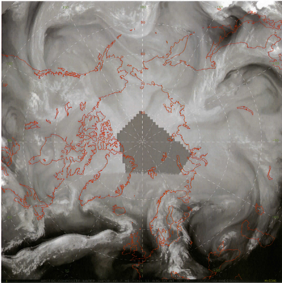
Figure 2. A water vapor channel (~6.7 micron) satellite composite over the Arctic shows traces of mid-tropospheric water vapor as well as cloud masses. The gray area over a portion of the Arctic basin is an area of missing satellite coverage where no satellite observations met the criteria for inclusion into the composite.
