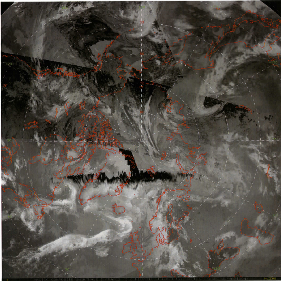
Figure 4. A short-wave infrared (~3.8 microns) Arctic composite showing the issues in compositing in this only semi-uniform spectral channel: Not all of the contributing satellites have the same peak wavelength - as some have 3.7 microns and others have 3.9 microns. Hence, the radiometric returns are slightly different between satellites (e.g. the polar orbiting passes are distinctive from the rest of the composite). Also, some of the geostationary satellites do have some quality challenges in this spectral band (as seen through Greenland and the North Sea).
