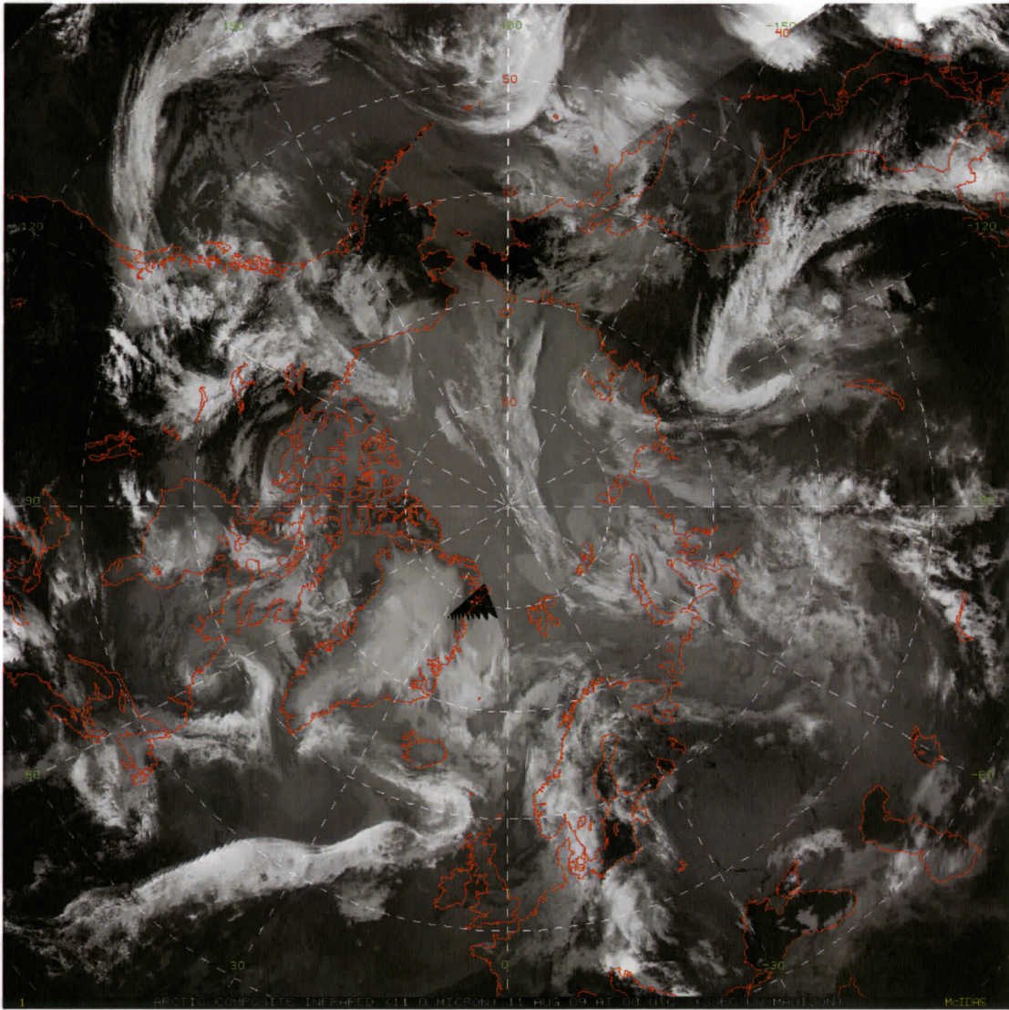
Figure 3. A long-wave infrared (~12.0 micron) Arctic composite satellite image depicting coverage much the same as the infrared composite.
