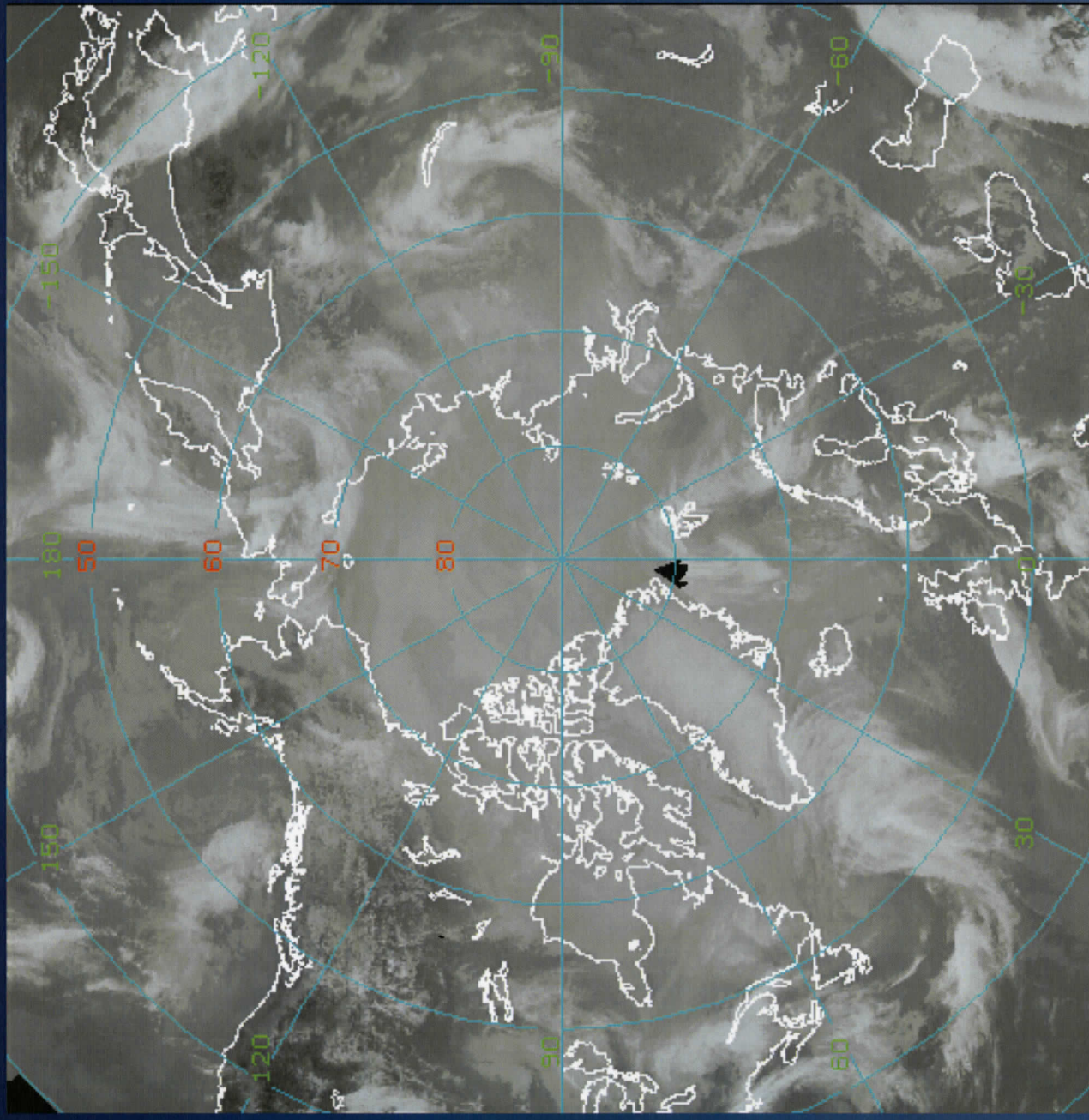
ARCTIC LONG WAVE COMPOSITE: 10 MAY 09 AT 00 UTC AMRC: SSE
