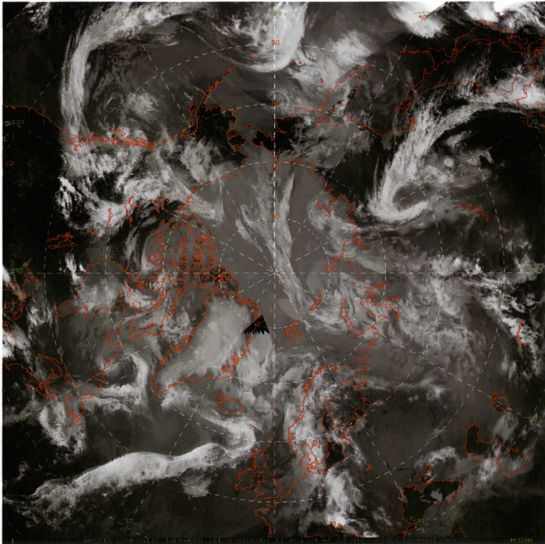
Figure 1. A sample Arctic infrared (~11.0 micron) satellite composite shows good satellite coverage over the Arctic basin and adjacent mid-latitude regions. Note the colder, white cloud masses and storm systems in the Westerly wind belt distinct from the warmer, darker summertime landmasses.
