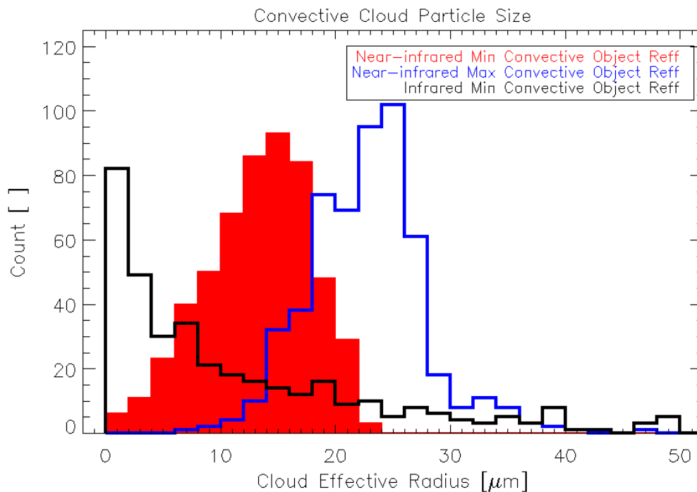
Figure 2.3.1. The histogram of the minimum value of effective particle radius ( r_{\text{reff}} ) in 541 deep convective cloud objects from an infrared retrieval as well as the histograms of the minimum and maximum values of r_{\text{reff}} in each cloud object from a near-infrared retrieval.
