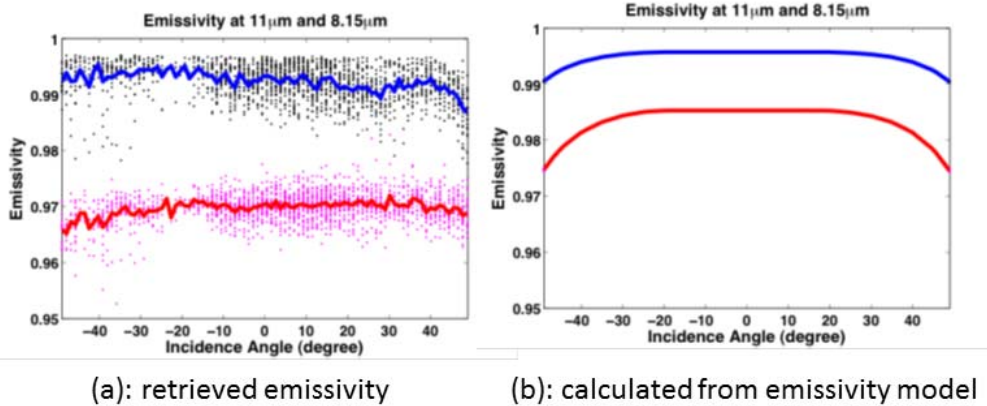
Figure 5.3.1. The retrieved emissivity versus the incidence angles (black: emissivity at 11 \mu\text{m} ; blue: mean emissivity at 11 \mu\text{m} for each angle; pink: emissivity at 8.15 \mu\text{m} ; red: mean emissivity at 8.15 \mu\text{m} for each angle) over ocean for Granule 046 on 03 September 2008.
