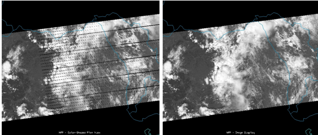
Figure 17.4.2. Original (left) and re-projected (right) VIIRS I-Band 1.
