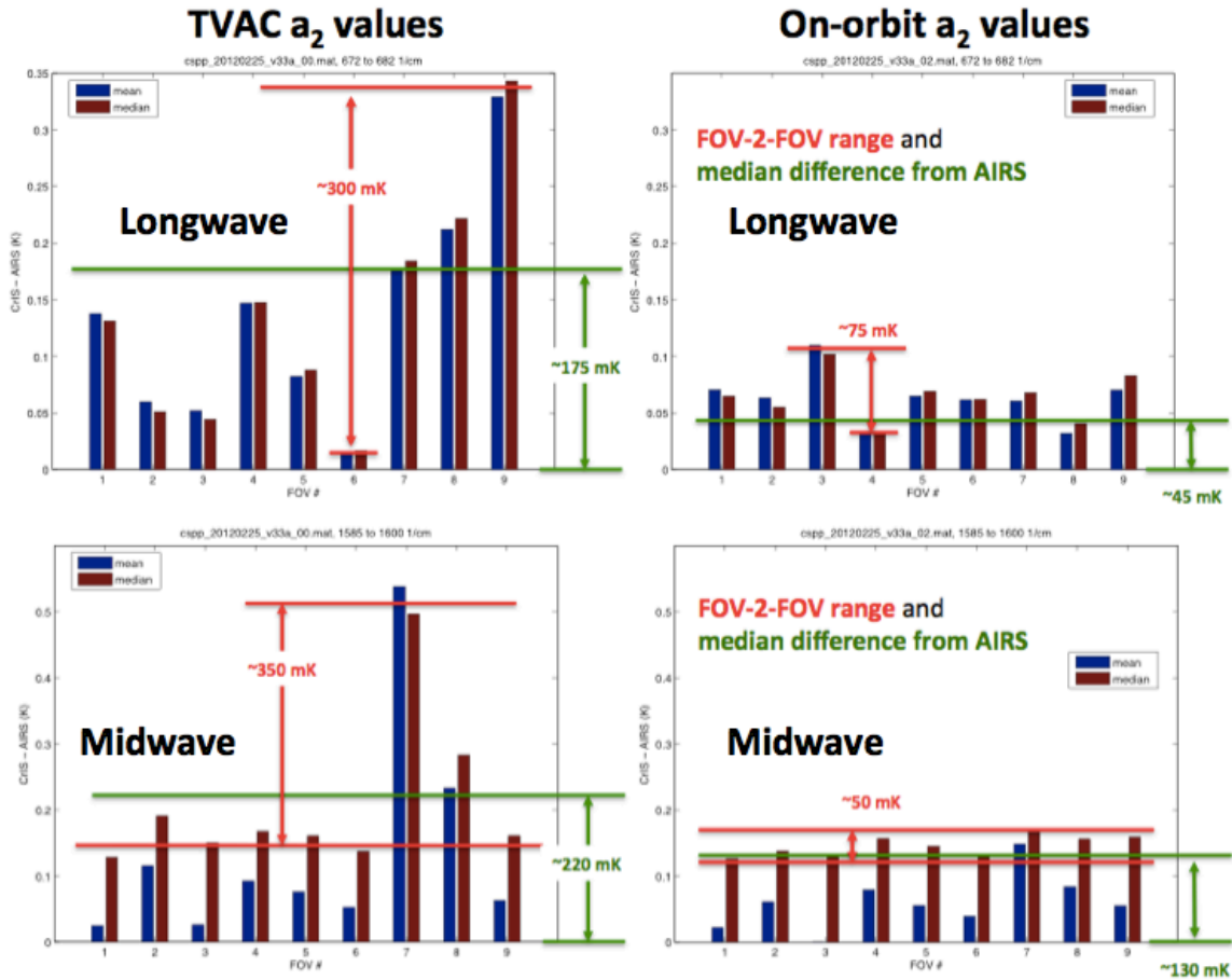
Figure 23.1.2. Example comparisons of CrIS and AIRS radiances (expressed in brightness temperature) using ~4800 SNOs collected on 25 February, for wavenumber regions which are most sensitive to the CrIS radiometric nonlinearity corrections. The left hand panels show comparisons using the at-launch (v32 Eng. Packet) a_2 nonlinearity correction coefficients, while the right hand panels show comparisons using the refined a_2 values (v33 Eng. Packet). The top panels are for the Longwave CO 2 region, and the bottom panels are for the Midwave water vapor region. With the refined a_2 values, the FOV-2-FOV agreement and overall agreement with AIRS is significantly improved.
