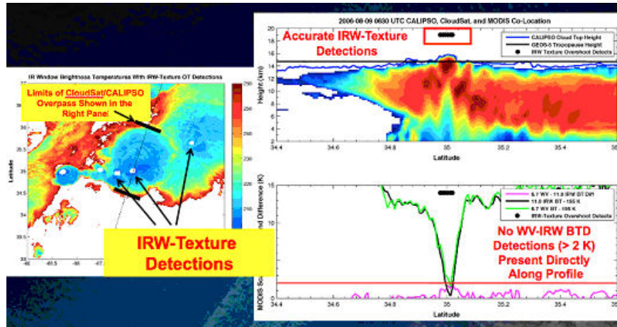
Figure 16.14.1. (left) Aqua MODIS 1 km 10.7 \mu\text{m} brightness temperature imagery with IRW-texture OT detections (white dots). (right) IRW-texture OT detections co-located with MODIS brightness temperatures, CloudSat radar reflectivity, CALIPSO cloud top height, and the NASA GEOS-5 model tropopause height analysis.
