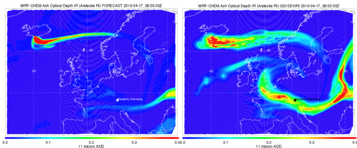
Figure 27.1. Forecasted (left) and GSI/SEVIRI assimilation (right) 11 micron volcanic ash Optical Depths at 08Z on April 17, 2010. The location of the ground based lidar in Maisach, Germany is indicated by an (*).
