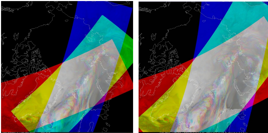
Figure 4.2.2. The gray region represents the overlap in three orbits where the polar winds are derived for MODIS (left) and VIIRS (right).
