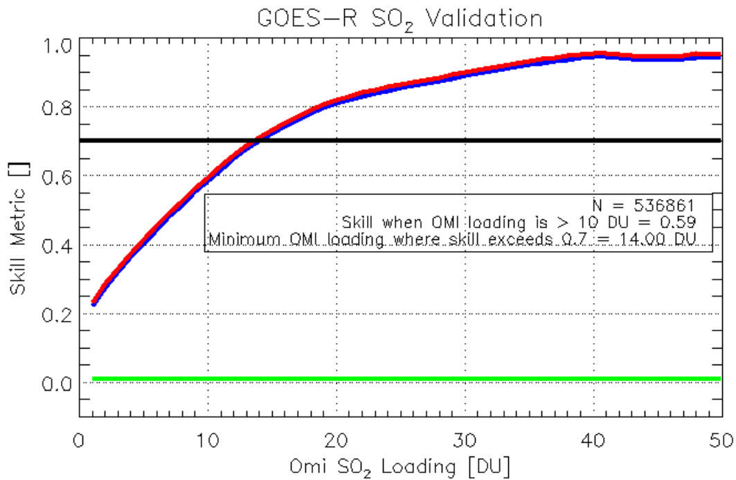
Figure 16.12.2. The true skill score statistic (red line) of the GOES-R binary SO 2 detection algorithm is shown as a function of the SO 2 loading estimated by the OMI. The hit (detection) rate is shown in blue and the false alarm rate is shown in green.
