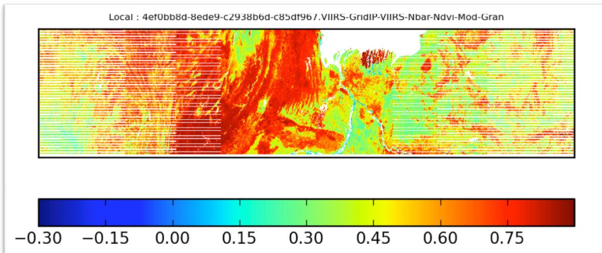
Figure 25.2: NDVI ancillary data processed in ADL using scripts developed at SSEC.
