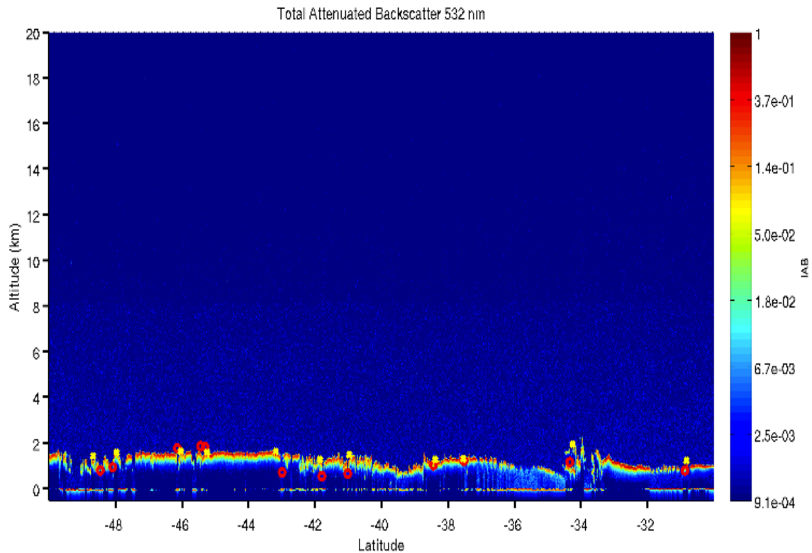
Figure 3.5.3. CALIPSO total attenuated backscatter with collocated AMV locations plotted in red and CALIPSO clouds in yellow.
