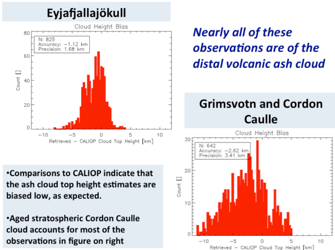
Figure 16.11.1. GOES-R Volcanic ash cloud height validation for Eyjafjallajökull (left) and Grimsvotn and Cordon Caulle (right) eruptions. The GOES-R retrieved height minus CALIOP cloud top height are displayed in each figure. The GOES-R ash cloud height low bias is expected given the coarser vertical resolution of broadband infrared measurements compared to visible lidar observations.
