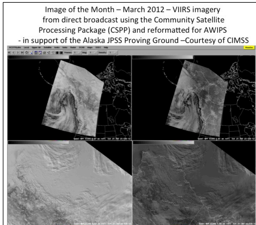
Figure 24.3.1. Example of VIIRS data as displayed in AWIPS I over Alaska. The data were reprojected and reformatted using the CIMSS VIIRS to AWIPS tool. Displayed are the VIIRS I-Band .64 micron reflectances (left panel) and the 1.61 micron reflectances (right panels). This figure was part of the Image of the Month as distributed by the JPSS Program Scientist, Dr. Mitch Goldberg.
