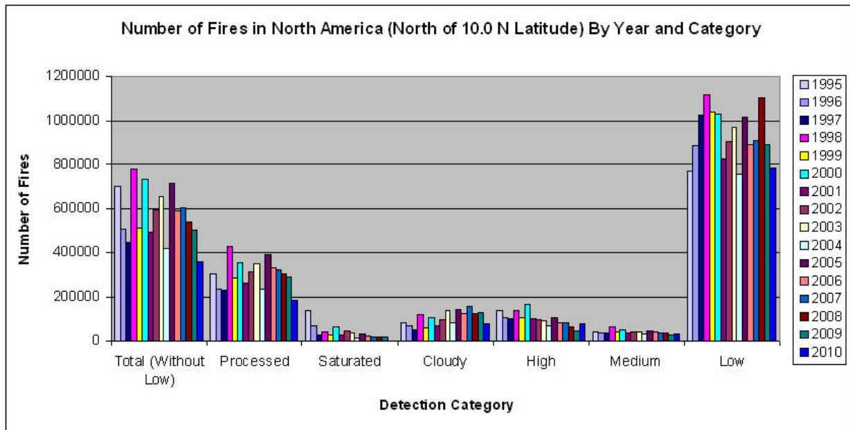
Figure 3.3.2. GOES East WF_ABBA v65 satellite coverage corrected total number of fires for each fire category for 1995-2010 over North America.
