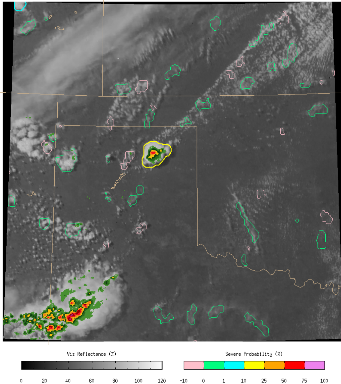
Figure 3.7.1. GOES-12 visible satellite imagery (grayscale shading), NEXRAD composite reflectivity (colored shading), and Bayesian model output for cloud objects (colored contours around various cloud objects) all valid 1945 UTC 15 May 2009. The developing supercell thunderstorm over the northeastern Texas panhandle has an enhanced probability (the only cloud object with an enhanced probability at this time). The enhanced probability occurs 21 minutes prior to the issuance of a severe thunderstorm warning.
