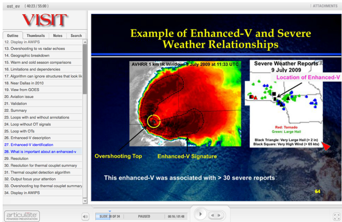
Figure 8.1. Screen capture from the Objective Satellite-Based Overshooting Top and Enhanced-V Anvil Thermal Couplet Signature Detection lesson, which is a component of the SHyMet: Severe Thunderstorm Forecasting track.
