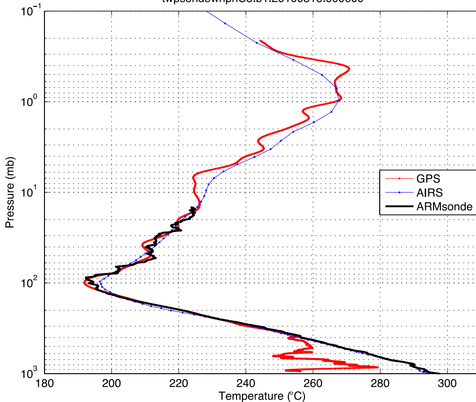
Figure 23.4.1. Example matchup between GPS RO, AIRS IR, and Vaisala radiosonde.
