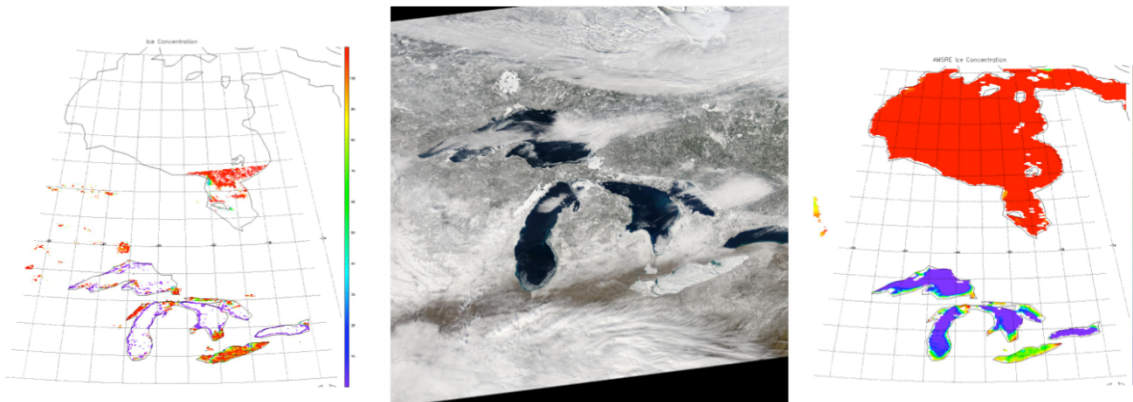
Figure 16.16.1. Lake ice concentration (%) with MODIS Aqua data (left), MODIS true color image (middle), and from AMSR-E (right) over Great Lakes on February 24 2008.
