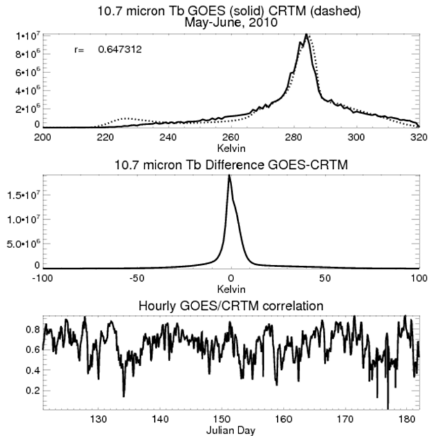
Figure 16.18.2. The upper panel shows histograms of GOES (solid) and CRTM (dashed) 10.7 micron brightness temperatures. The middle panel shows the histogram of 10.7 micron brightness temperature differences (GOES-CRTM), and the lower panel shows a time series of hourly spatial correlations between GOES and CRTM 10.7 micron brightness temperatures over the CalNex domain during May-June 2010.
