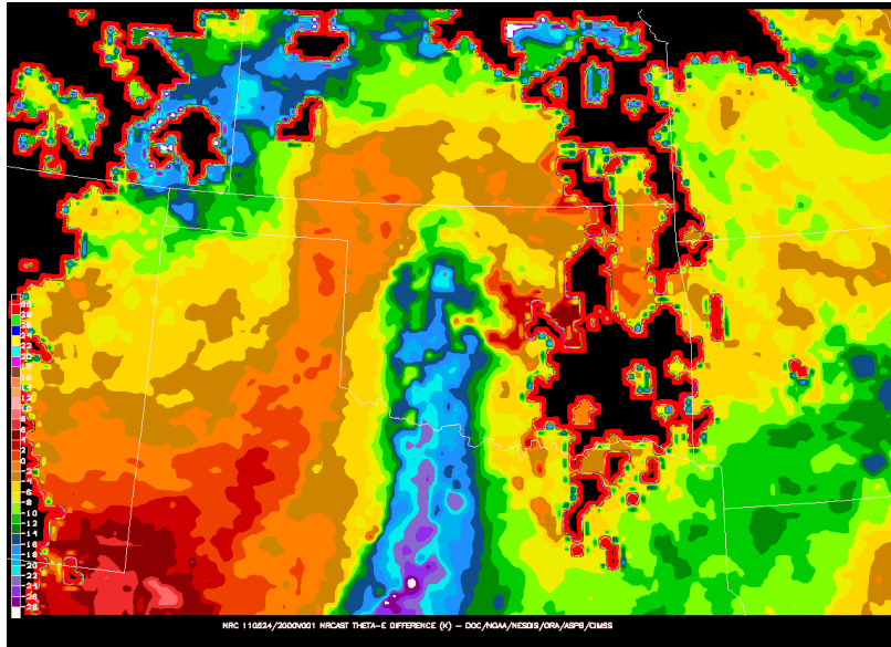
Figure 15.3. Nearcast differential theta-e product displayed within HWT N-AWIPS workstations at 2000 UTC on 24 May 2011.
