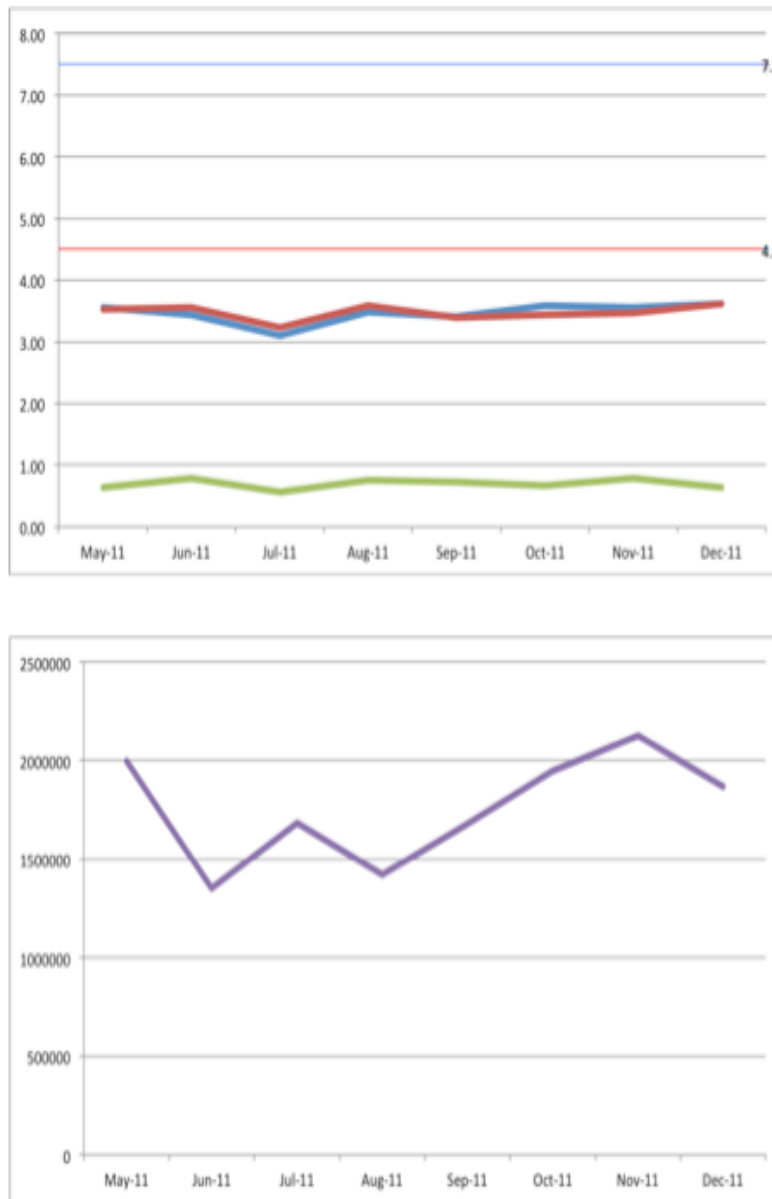
Figure 16.8.1. Monthly comparison statistics (ocean only) between AMVs computed using all bands and all levels from full disk Meteosat-9 and NCEP GFS Analysis winds (valid at all synoptic times) for the months of May 2011 through December 2011. Bottom image is the number of AMV GFS analysis matches.
