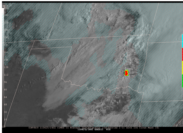
Figure 15.5. UWCI overlaid on GOES-13 visible imagery within HWT N-AWIPS workstations at 1402 UTC on 25 April 2011. Blue dashed areas indicate ice-cloud exclusion regions where the convective cloud mask has determined CI nowcasts cannot be made. Pre-CI growth is indicated by green filled areas, CI-likely is indicated by yellow filled areas, and CI-ongoing is indicated by red filled areas.
