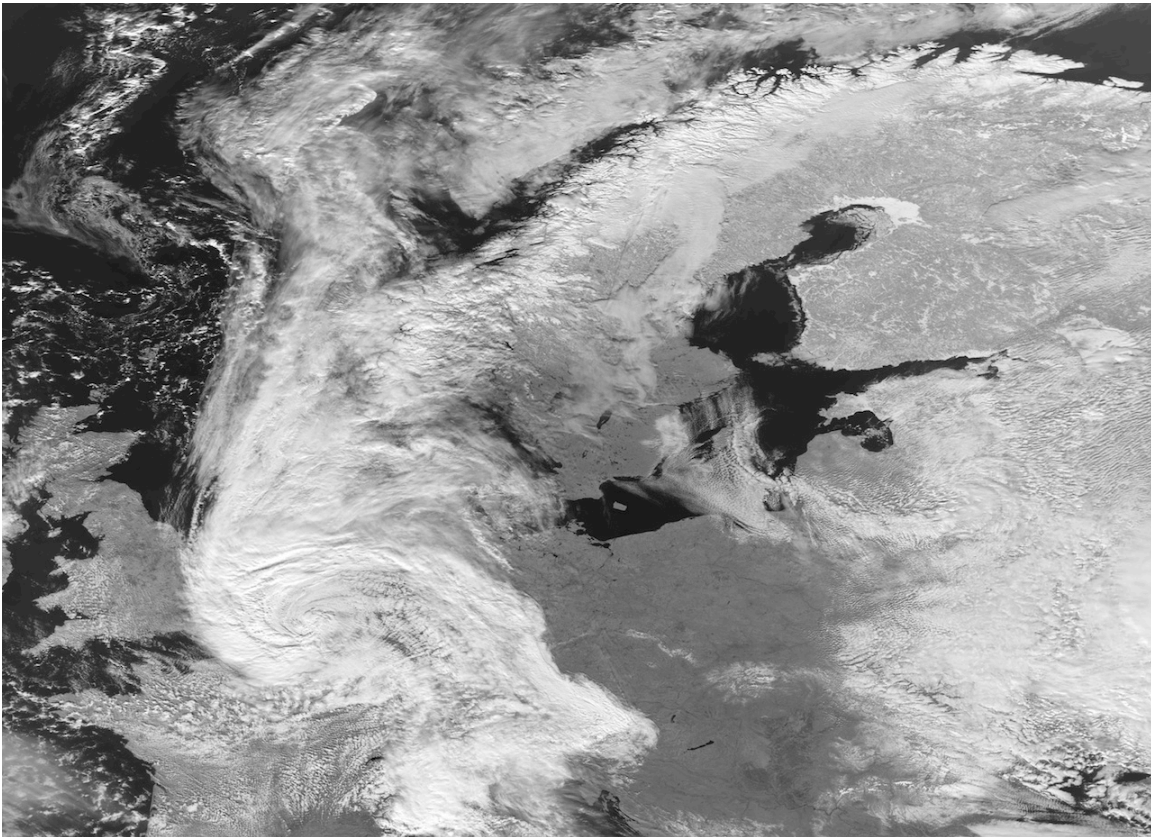
Figure 26.1. First VIIRS data received by FMI and processed by CSPP (2012/03/09).
