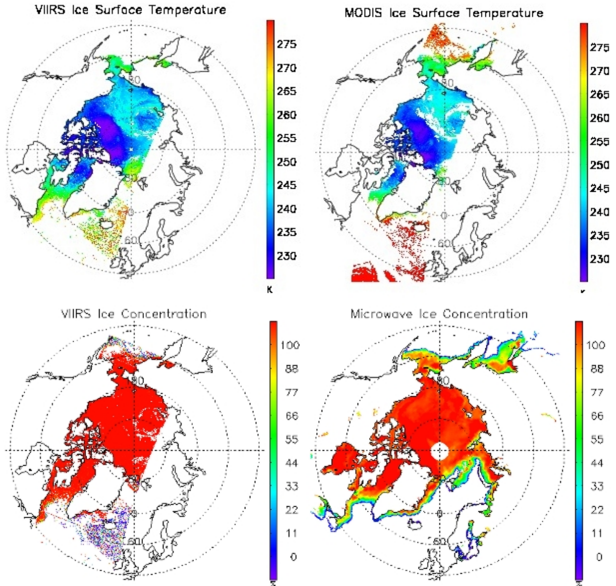
Figure 22.1. Ice surface temperature from VIIRS (upper left), MODIS (upper right) in 1 km EASE-Grid; Ice concentration from VIIRS (lower left), and SSM/I (lower right) in 25 km EASE-Grid over Arctic on March 7, 2012.
