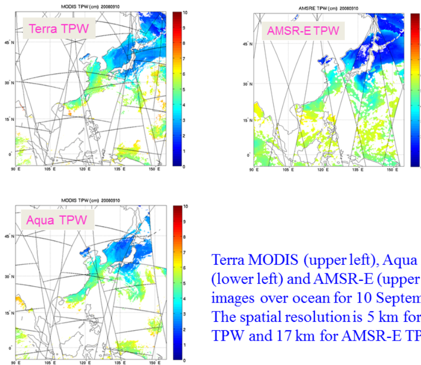
Figure 12.1. The Terra MODIS (upper left), Aqua MODIS (lower left) and Aqua AMSR-E (upper right) TPW images over ocean for 10 September 2008.
