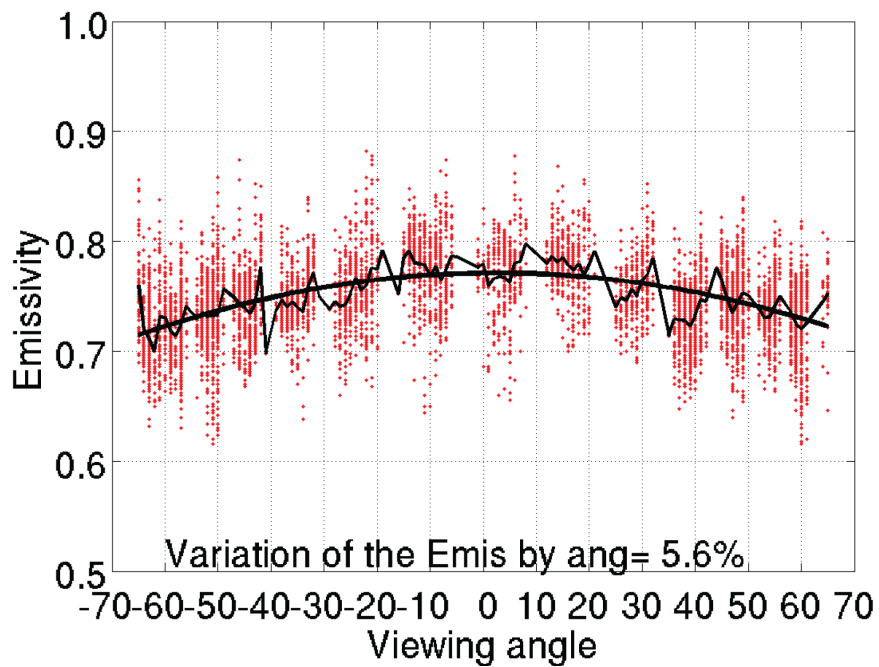
Figure 16.1.1. Top panel: Selected homogenous sandy area for the angular dependence study. The main picture shows the 8.3 \mu\text{m} MYD11C3 monthly mean emissivity for January 2011 and the sub-image shows the zoomed Google map image of that area. Bottom panel: Angular dependence of the MODIS MYD11C1 emissivity products at 8.3 \mu\text{m} for January 2011.
