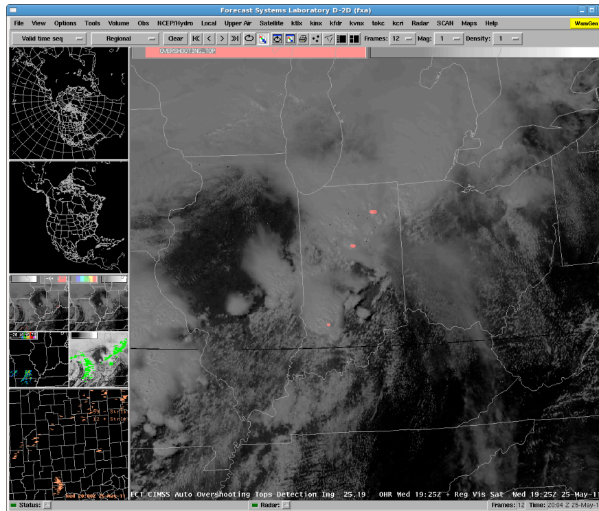
Figure 15.2. OTTC overlaid on GOES-13 visible imagery within HWT AWIPS workstations at 1925 UTC on 25 May 2011. Red areas indicate detections of overshooting-tops by the OTTC product.
