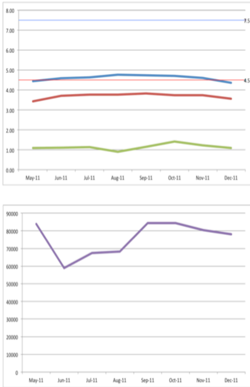
Figure 16.8.3. Monthly comparison statistics (ocean only) between AMVs computed using all bands at mid levels (400 – 700 hPa) from full disk Meteosat-9 and NCEP GFS Analysis winds (valid at all synoptic times) for the months of May 2011 through December 2011. Bottom image is the number of AMV GFS analysis matches.
