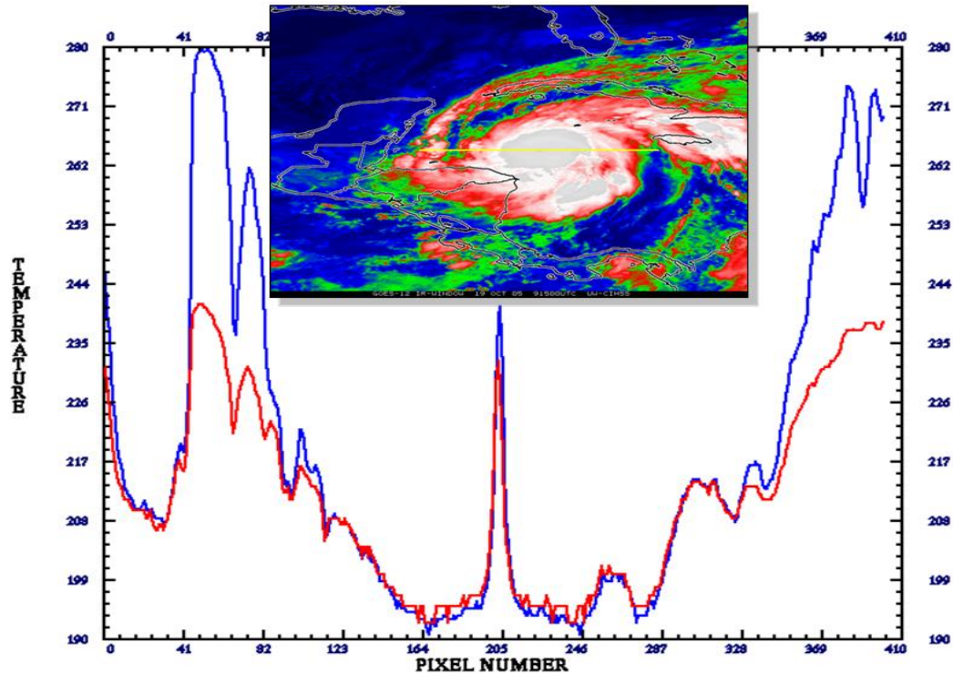
Figure 3.4.1. Cross section of GOES-12 brightness temperatures ( T_b ) during Hurricane Wilma (2005) near the time of its maximum intensity on 19 October/09:15UTC. The west to east cross section transverses the eyewall as well as the outer rainbands of the storm. In the outer regions of the TC, the clouds are typically less opaque or missing entirely, resulting in brightness temperature measurements in line with those expected; WV T_b s (red) are colder than the corresponding IRW values (blue). In the inner eyewall region, however, this relationship reverses as water vapor above the convection is forced through the tropopause and into the stratosphere where it re-emits in the WV emission bands at higher temperatures. Here, the IRW minus WV (IRWV) difference values are near zero or negative, indicating the presence of vigorous convection “overshooting” into the stratosphere.
