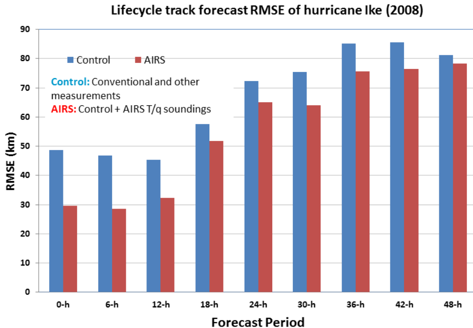
Figure 12.4. Lifecycle Hurricane Ike track forecast RMSE for 0-hour (analysis), 6-h, 12-h, 18-h, 24-h, 30-h, 36-h, 42-h and 48-h forecasts.
