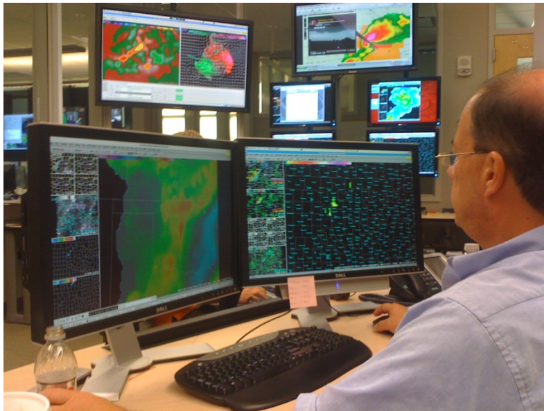
Figure 15.4. Nearcast differential theta-e product evaluated by NWS forecaster during EWP warning operations on 9 June 2011.
