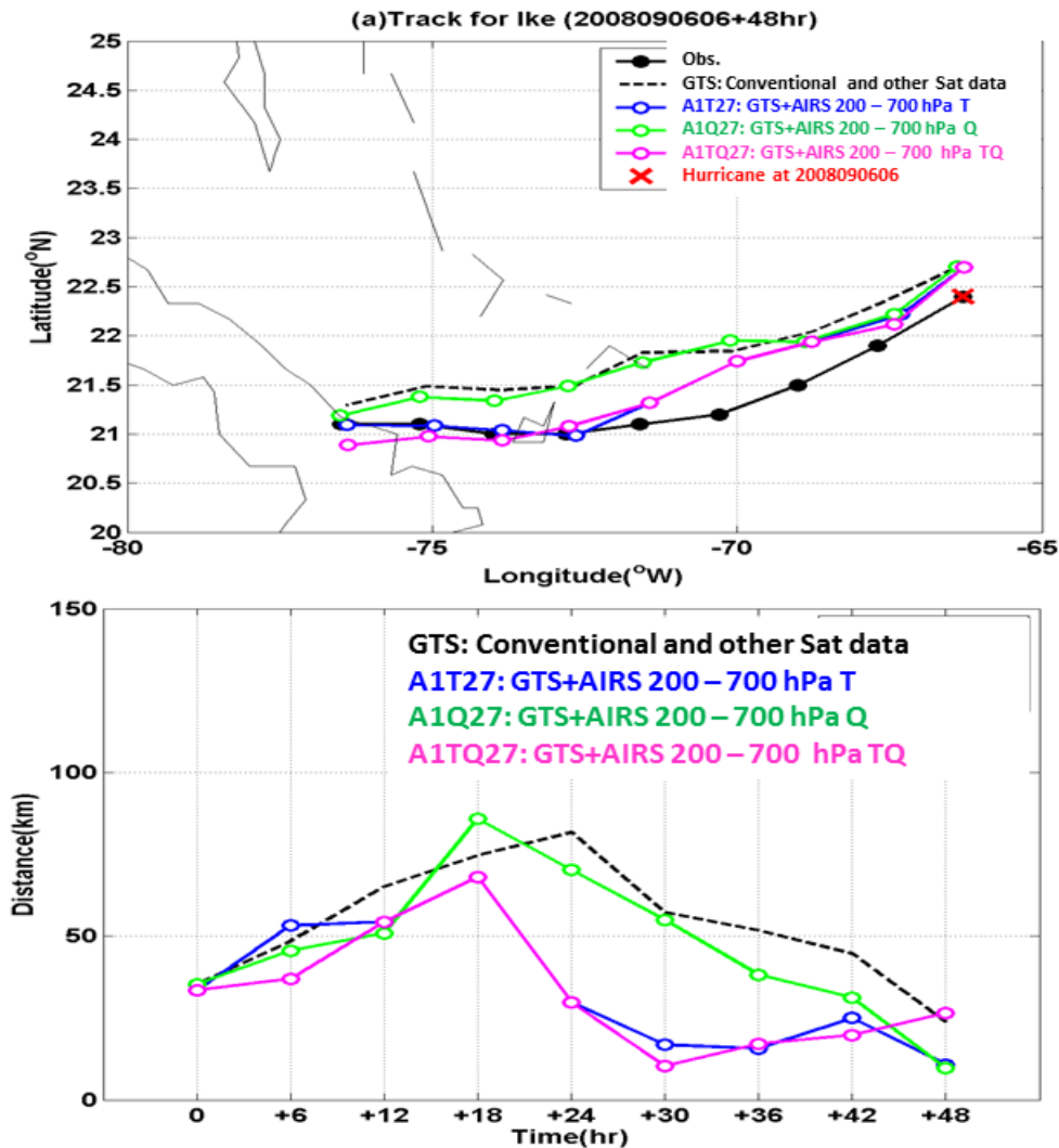
Figure 12.3. (Upper) The 48-hour forecasts with GTS (conventional data and other satellite measurements) (dashed black), GTS + AIRS temperature profile (blue), GTS + AIRS moisture profile (green), GTS + AIRS temperature and moisture profiles (pink) assimilated, respectively, for Hurricane Ike track forecasts. (Lower) The respective track forecast errors.
