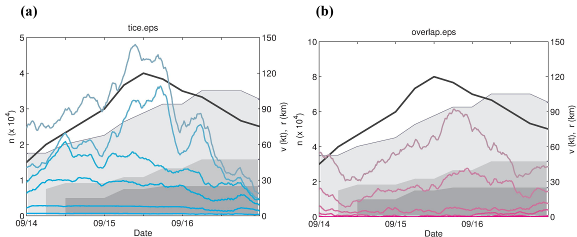
Figure 14.11.1. Julia's (2010) intensity (kt) (black) (from best track data), the radius (km) of 34-kt (light gray shading), 50-kt (medium gray), and 64-kt (dark gray shading) winds (from ATCF data), along with (a) the number of MSG-SEVIRI-based thick ice pixels within 50, 100, 200, 300, 500, and 1000 km of center (bright to dull blue), (b) the number of MSG-SEVIRI-based overlap cloud type pixels within 50, 100, 200, 300, 500, and 1000 km of center (bright to dull magenta).
