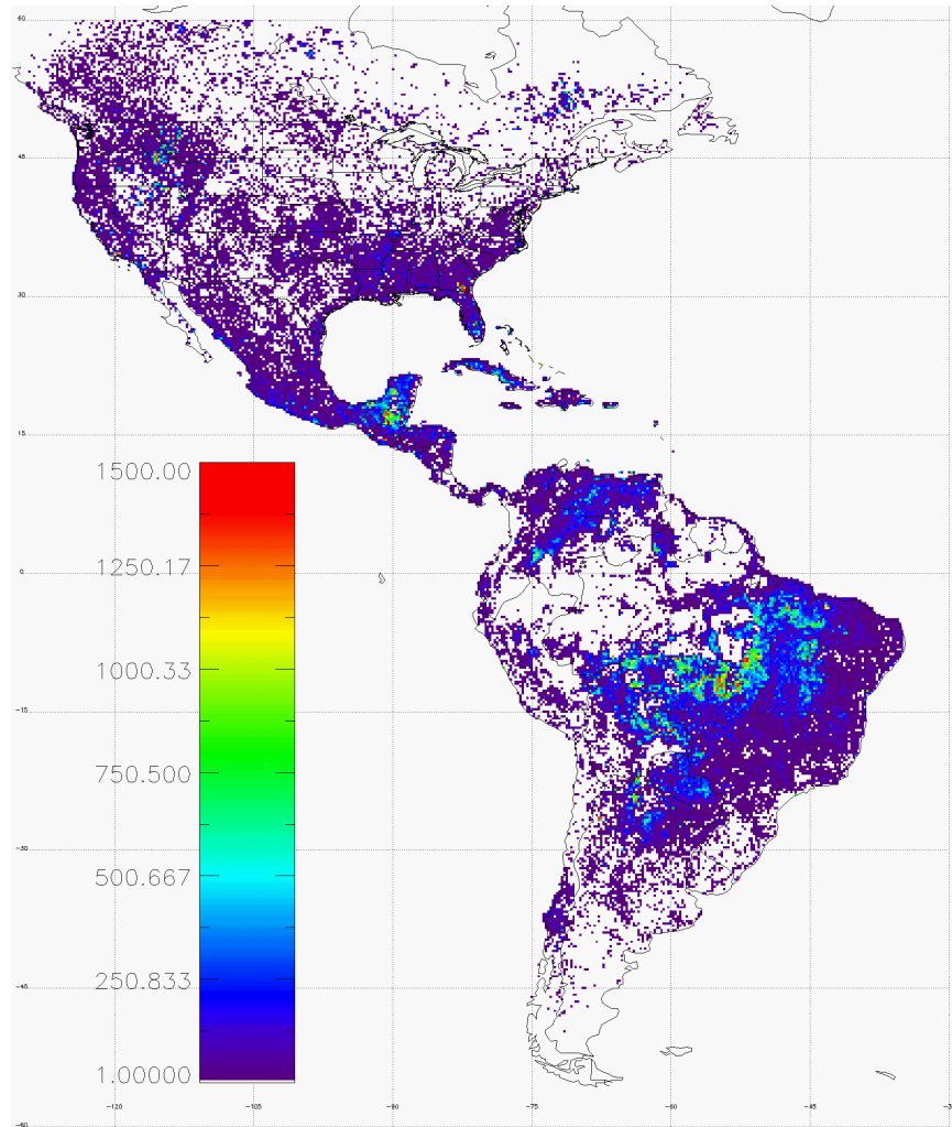
Figure 3.3.1. GOES East WF_ABBA v65 satellite coverage corrected 0.25 degree binned total number of fires (all fire categories included but low possibility) for 2007 over the Western Hemisphere.
