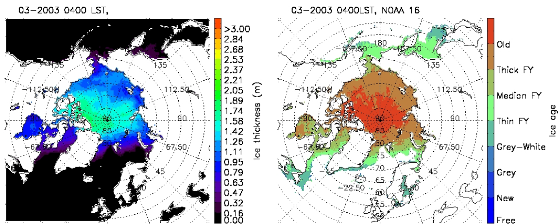
Figure 6.2.1. Ice thickness (left) and age (right) over the Arctic based on APP-x products. These two products will be part of the enhanced APP-x product set.
