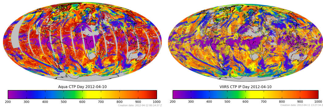
Figure 23.5.2. Global gridded CTP retrievals for MODIS Aqua (left figure) and VIIRS (right figure). The color scales are identical for each image.
