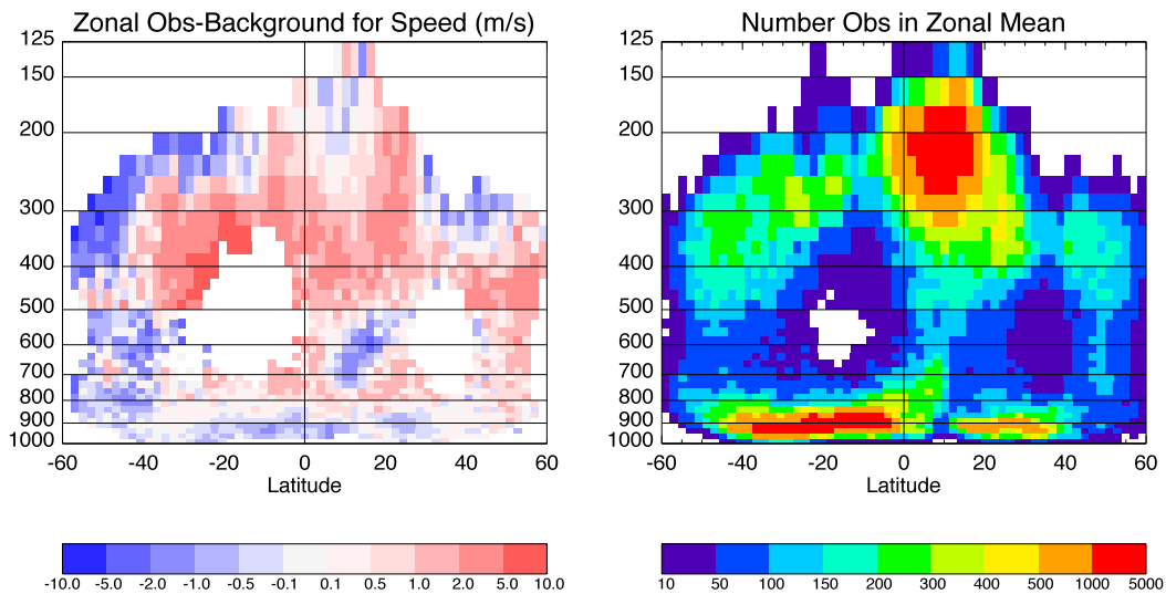
Figure 14.6.1. Zonal Mean for Observation minus Background GFS state of speed \text{m s}^{-1} and number of AMVs.
