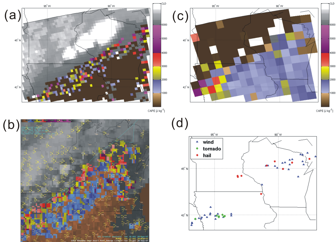
Figure 12.5. (a) The clear sky CAPE (color regions) from AIRS SFOV sounding overlaying the AIRS 11 \mu\text{m} brightness temperature image at 19:10 UTC 28 August 2007. (b) The clear sky CAPE (color regions) from GOES-12 DPI overlaying GOES-12 window channel brightness temperature image at 17:00 UTC 28 August 2007. (c) Corresponding science team AIRS/AMSU sounding CAPE at 19:10 UTC 28 August 2007. (d) The reported high wind, tornado and hail locations during 17:00 UTC and 23:50 UTC on 28 August 2007.
