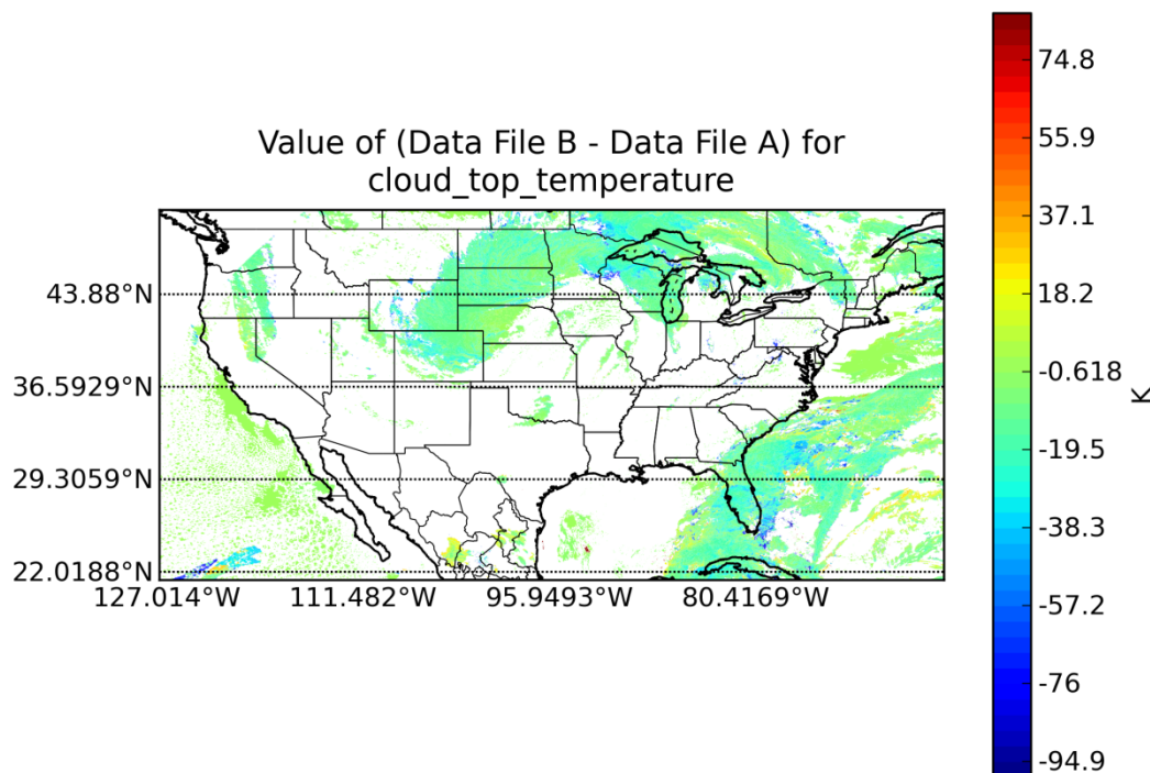
Figure 16.2.1. The difference in cloud top temperature between WRF model generated cloud top heights and those measured in WRF-generated (proxy) ABI data using the ABI cloud top temperature algorithm. A cold bias in the differences are seen, indicating that model cloud top temperatures are colder than those sensed by the ABI algorithm.
