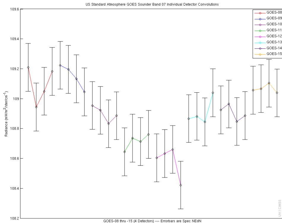
Figure 14.3.1. GOES Sounder Band 07 individual detector convolutions with the US Standard Atmosphere. The error bars represent NEdN (noise in radiance units); when the difference between two detectors exceeds NEdN it is considered “out of family” for the purposes of this study. GOES-8, -12, and -13 all have one detector that is out of family for this band in this atmosphere.
