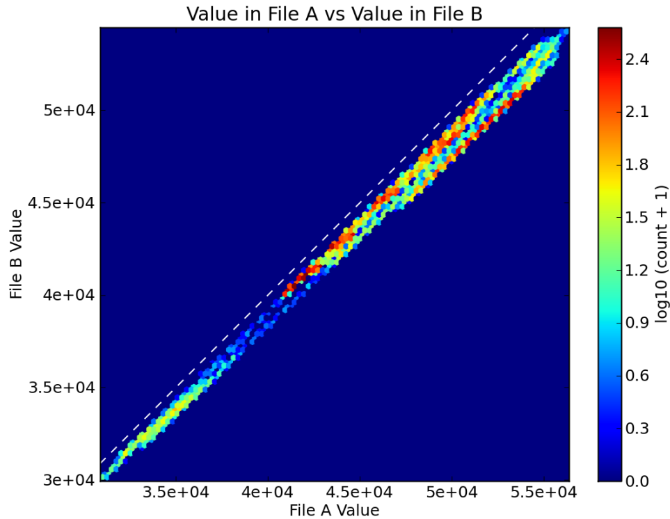
Figure 16.3.1. Sample diagnostic hex-density scatter plot of Suomi NPP ATMS unscaled brightness temperatures which was created as part of regression testing of data processing software. A semi-automated search for this systematic bias was implemented using glance, which pointed directly at a reconfiguration event and allowed rapid remediation by obtaining updated configuration data.
