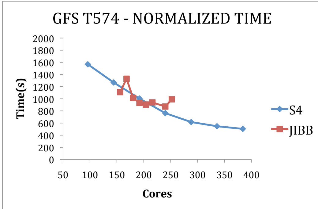
Figure 20.2. Scaling Performance vs. Number for Cores for S4 and JIBB/GSFC System.
