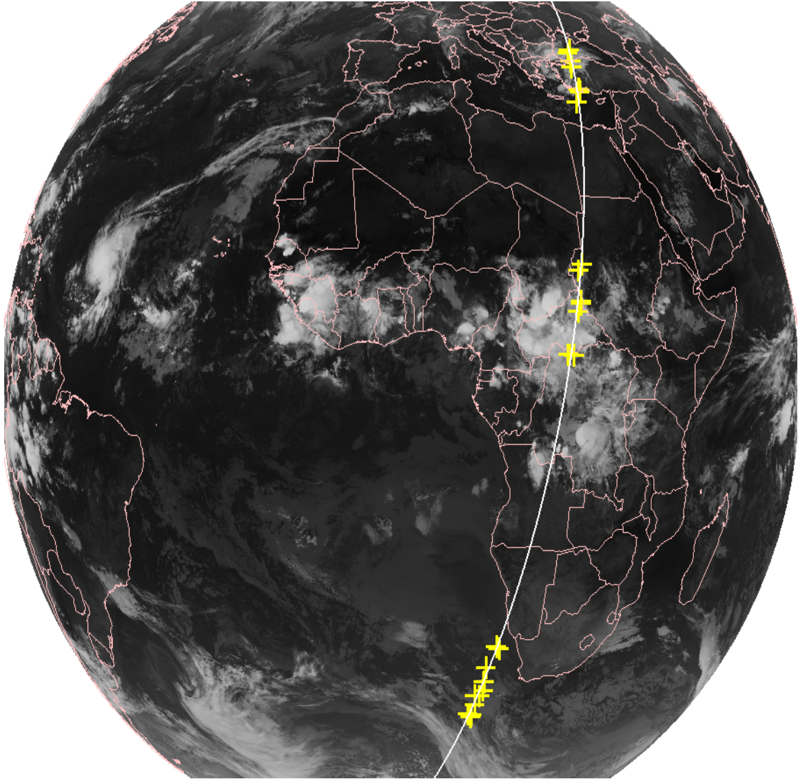
Figure 3.5.5. AMV CALIPSO match locations for 22 September 2011 at 00 UTC.
