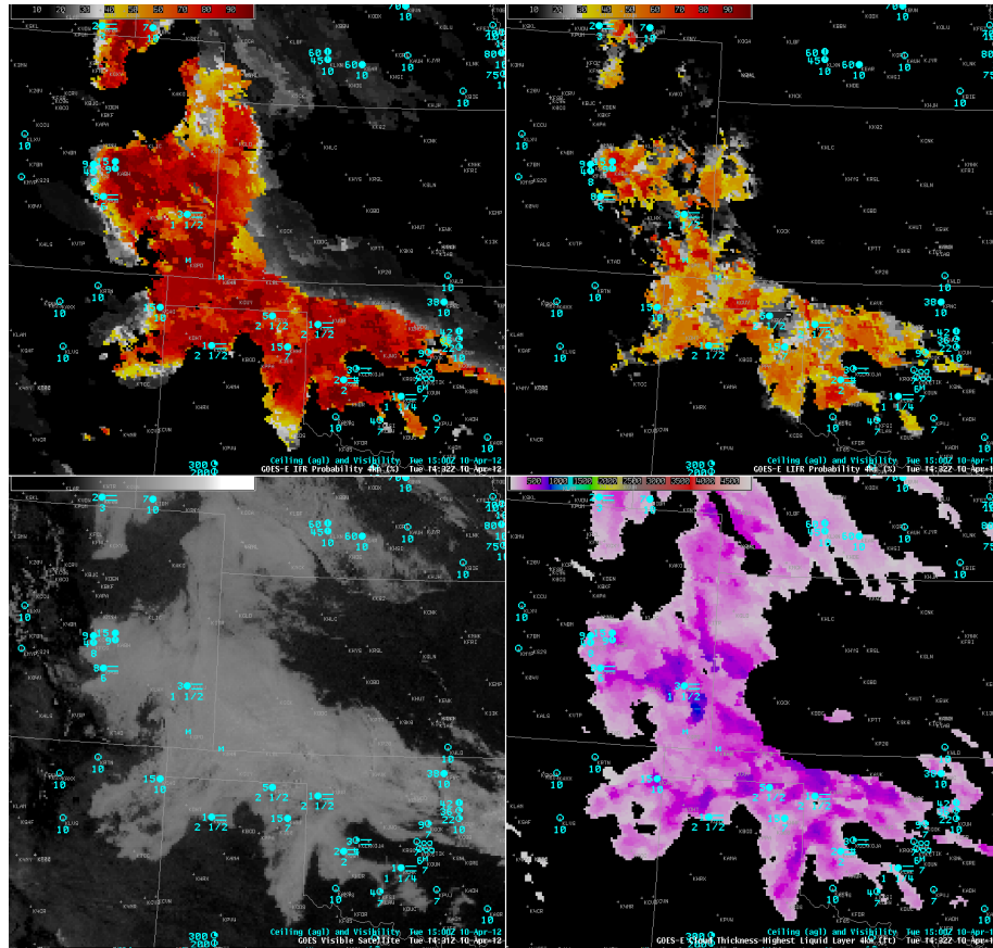
Figure 16.13.1. Example output from the GOES-R fog/low cloud algorithm from April 10, 2012 at 10:02 UTC (night) (top four images) and 14:32 UTC (day) (bottom four images) centered over N. Texas, E. Colorado and W. Kansas. The top, left panels in each 4-panel image are the probabilities that IFR conditions are present. The top, right panels are the probabilities that LIFR conditions are present. The bottom, right panels show the estimated thickness of the highest liquid water cloud layer. The bottom, left panels are the 11 \mu\text{m} brightness temperature (night) and 0.65 \mu\text{m} visible reflectance (day). The blue symbols are surface observations with surface visibility, in miles, on the bottom and cloud ceiling, in 100's of feet, on the left.
