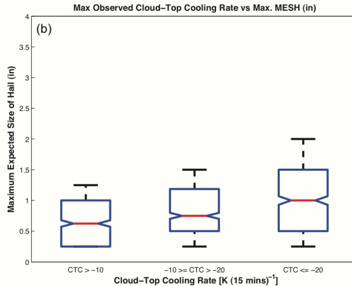
Figure 3.1.1. Comparison of maximum UWCI-CTC rates to maximum Maximum Expected Hail Size (MESH) for cloud objects that had both an UWCI-CTC rate and valid MESH at some point in their lifetime. UW-CTC rates are binned by intensity [ \text{K (15 min)}^{-1} ] with weak, moderate, and strong convective growth defined as UW-CTC > -10 , -10 \geq UW-CTC > -20 , and UW-CTC \leq -20 , respectively. For each boxplot, the median (red line), 25 th and 75 th percentiles (lower and upper bounds of blue box), and one standard deviation (whiskers) are shown. The medians of different intensity bins are significantly different at the 95% confidence level if the widths of the notches centered on the medians do not overlap.
