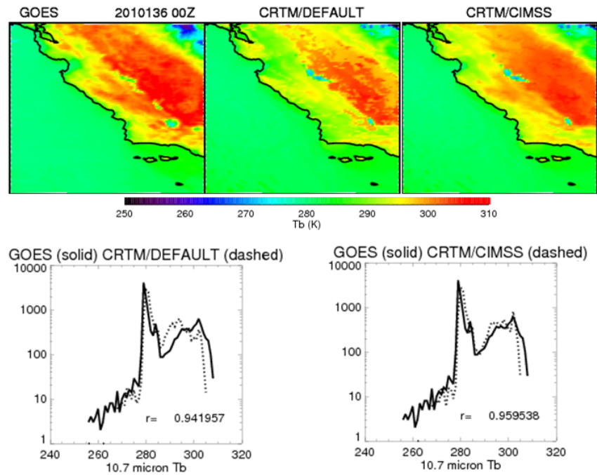
Figure 16.18.1. Comparison between GOES-11 (upper left) and CRTM 10.7 micron brightness temperatures at 00Z on May 16, 2010 using the default CRTM land emissivity LUT (upper center) and the CIMSS UWIREMIS land emissivity data base (upper right). The lower panels show histograms of GOES (solid) and default (dashed, lower left) and UWIREMIS (dashed, lower right) brightness temperatures.
