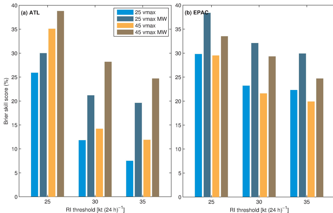
Figure 14.12.1. Comparative Brier skill scores (BSS) for TCs tested in the (a) Atlantic Ocean and (b) East Pacific Ocean, for RI thresholds of 25, 30, and 35 kt (24 h) -1 for the logistic RI scheme using no MI predictors [light blue for all TCs ( N = 1360 and 1120 for the ATL and EPAC, respectively); orange for TCs with v_{\max} of at least 45 kt ( N = 1013 and 733 for the ATL and EPAC, respectively)] and including MI predictors (dark blue for all TCs; brown for TCs with v_{\max} of at least 45 kt).
