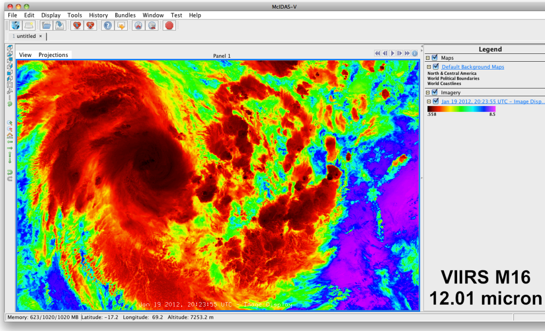
Figure 24.4.2. Tropical Cyclone Ethyl, visualized in McIDAS-V utilizing VIIRS M-Band 16 on January 19, 2012.
