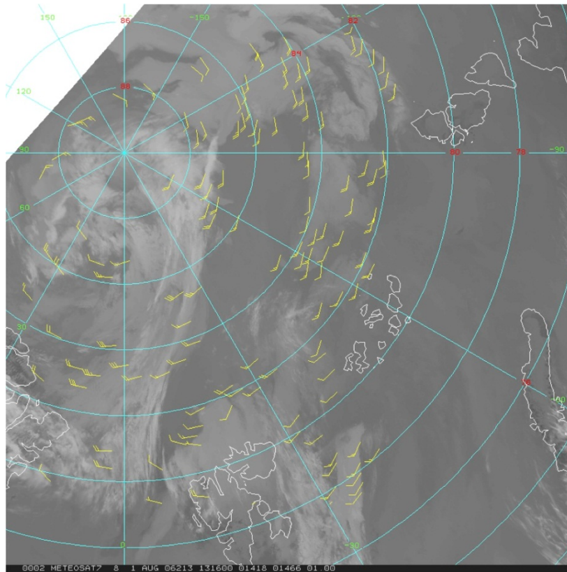
Figure 4.2.3. Polar winds based on MODIS data using the VIIRS/ABI processing system.
