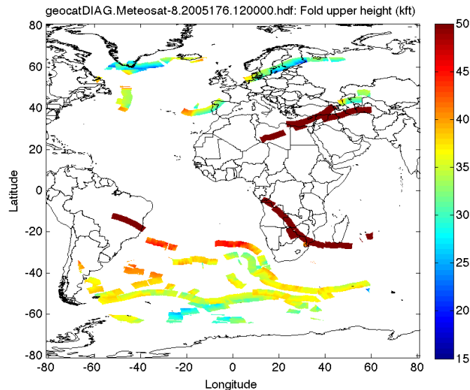
Figure 16.10.2. Tropopause folds for previous image, displayed as the maximum height (units: kft). In the midlatitudes of the northern hemisphere, significant tropopause folds occur at blocking boundaries in the North Atlantic and southern Greenland, at a low pressure system west of the Iberian peninsula, and in connection with a polar air mass front across Scandinavia.
