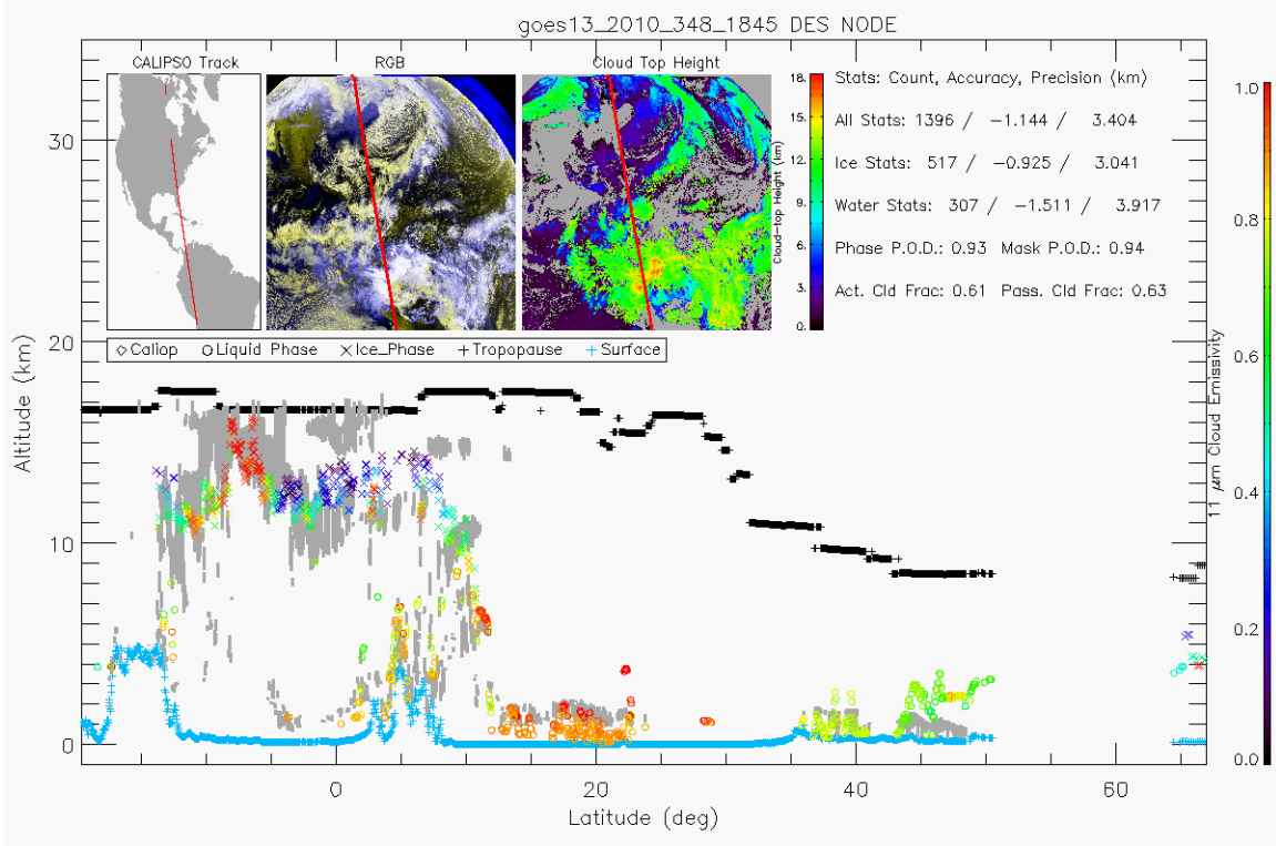
Figure 4.1.1. Comparison of cloud top height derived from ACHA to those derived from CALIOP as part of a validation effort. Figure above is an example from GOES-13.
