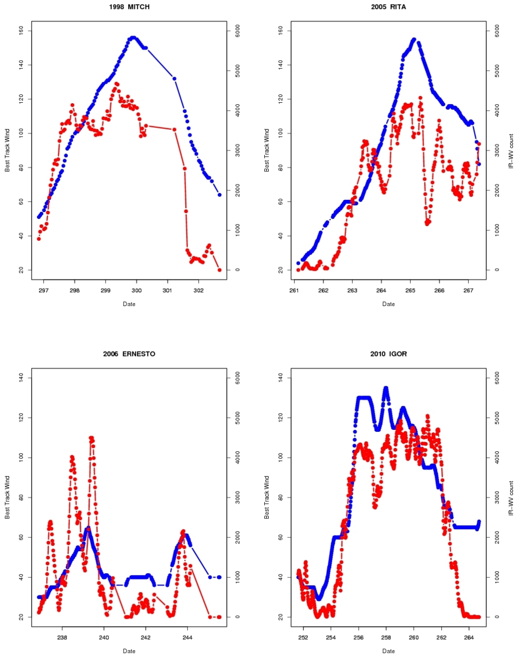
Figure 3.4.2. IR-WV pixel count values less than zero (Y-axis/right side; red lines/dots) versus NHC Best Track wind speed estimates (Y-axis/left side) blue lines/dots) for four storms in rapid intensification (RI) study sample. Hurricanes Mitch, Rita and Igor all exceeded the NHC criteria for RI and were correctly identified by the IR-WV RI identification scheme prior to the onset of RI in the NHC Best Track. Hurricane Ernesto was falsely identified as a potential RI storm with the IR-WV methodology, but did not meet the NHC criteria during its lifecycle possibly due to land interaction after reaching its maximum intensity of 65 knots on August 29 (Julian day 239).
