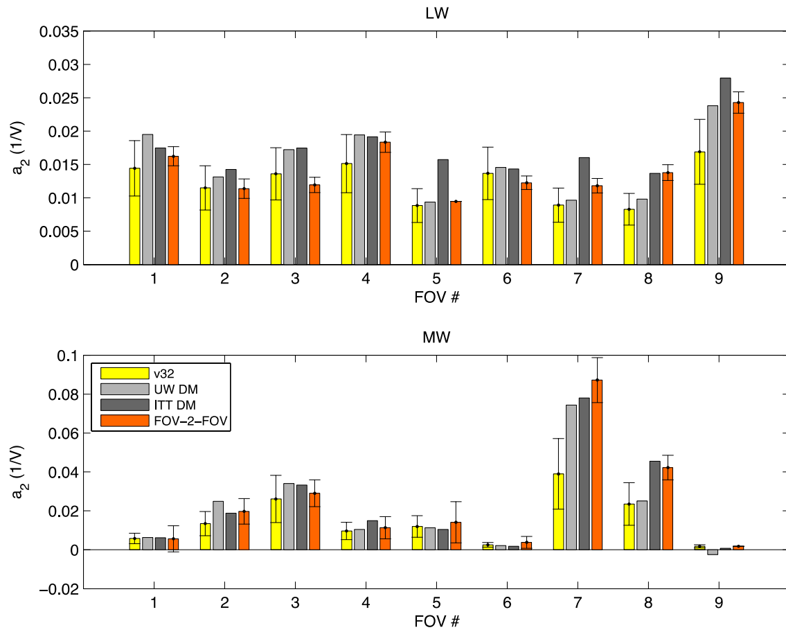
Figure 23.1.1. CrIS radiometric nonlinearity correction coefficients, a_2 , determined during thermal vacuum testing (yellow), from in-orbit Diagnostic Mode data and analysis (by UW, light grey, and ITT/Exelis, dark grey), and from in-orbit FOV-2-FOV consistency analysis (orange). The CrIS longwave and midwave bands exhibit quadratic nonlinearity and this accounts for a significant portion of the CrIS Radiometric Uncertainty. To reduce the overall Radiometric Uncertainty and to create optimal agreement between the nine CrIS FOVs in each band, we have performed analyses to determine the optimal a_2 values. At-launch a_2 values were determined from thermal vacuum testing (v32 Eng. Packet, yellow) and the refined values were determined from FOV-2-FOV Earth view analysis (v33 Eng. Packet, orange).
