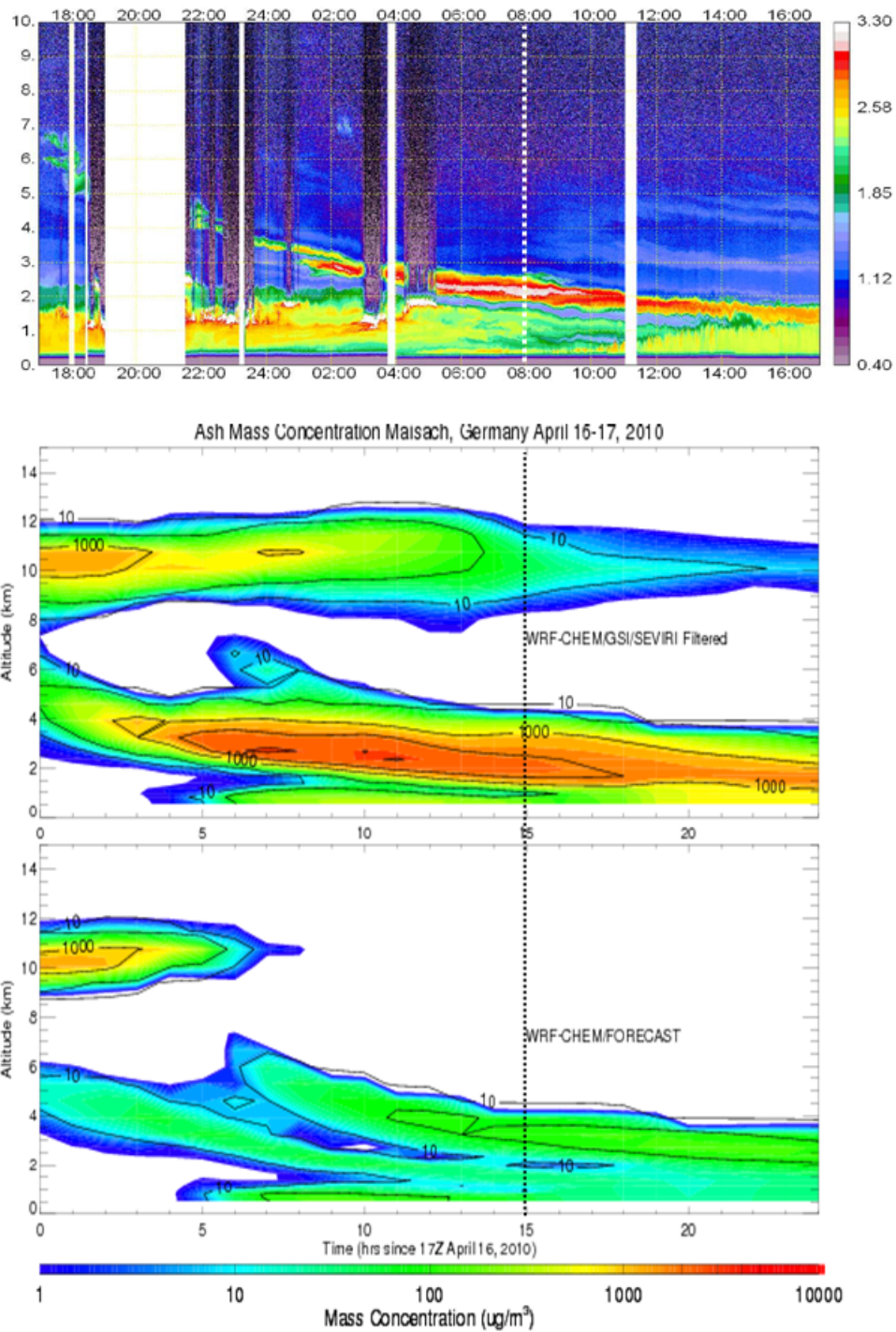
Figure 27.2. The upper panel shows the logarithm of range-corrected aerosol backscatter at 1064 nm over Maisach from 16 April 2010 17:00 UTC to 17 April 2010 17:00 UTC (reproduced from Gasteiger et al., 2011). The middle panel shows time height cross sections of the logarithm of volcanic ash mass concentration ( \mu\text{g}/\text{m}^3 ) from WRF-CHEM GSI/SEVIRI experiment and the lower panel shows volcanic ash mass concentrations from the baseline experiment.
