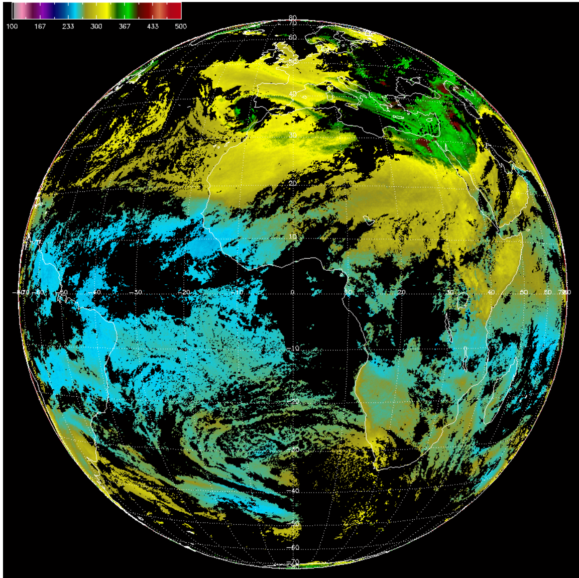
Figure 16.4.1. SEVIRI Total Column Ozone on 30 March 2012 at 8:30 UTC. A cut-off low pressure system is seen off the coast of Spain. Pixels with fully transparent clouds have been excluded. Some surface features, such as along the south western coast of Africa, can be seen contaminating the ozone field. Additionally, there are suggestions of surface contamination in the Middle East as well.
