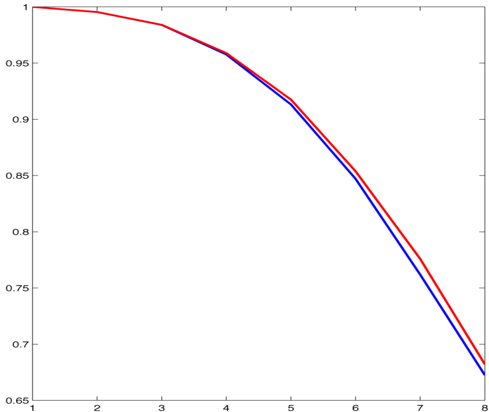
Figure 14.13.2. The Anomaly Correlation Coefficient (ACC) vs. forecast day for the 500 hPa heights in the southern hemisphere for the control (blue) and experiment (red). This is an average over 12 weeks: 02 May 2011 – 24 July 2011.
