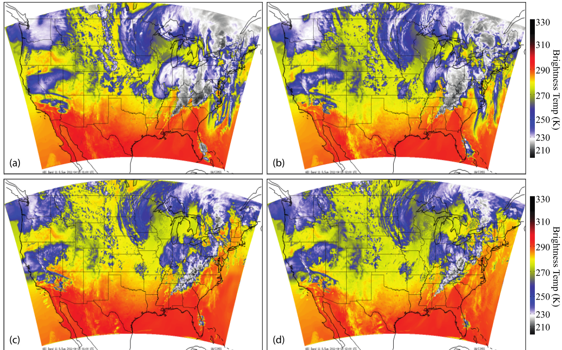
Figure 14.9.1. Simulated ABI 8.5 \mu\text{m} brightness temperatures (K) valid at 0100 UTC on 28 April 2011 for four of the CAPS ensemble members.
