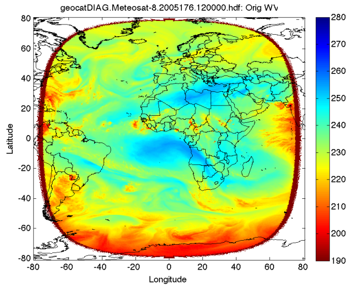
Figure 16.10.1. Meteosat-8 Water vapor channel (brightness temperature) for 1200 UTC on June 25, 2005.
