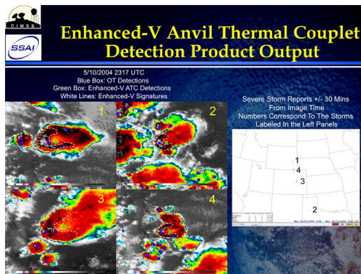
Figure 16.14.2. ABI proxy IRW (10.7 \mu\text{m} brightness temperature) 2 km imagery of a set of four enhanced-V producing severe storms that occurred on 10 May 2004 at 2317 UTC. Each enhanced-V signature is outlined with a white dashed line. Overshooting top detections are shown with blue squares and anvil thermal couplet detections are shown with green squares.
