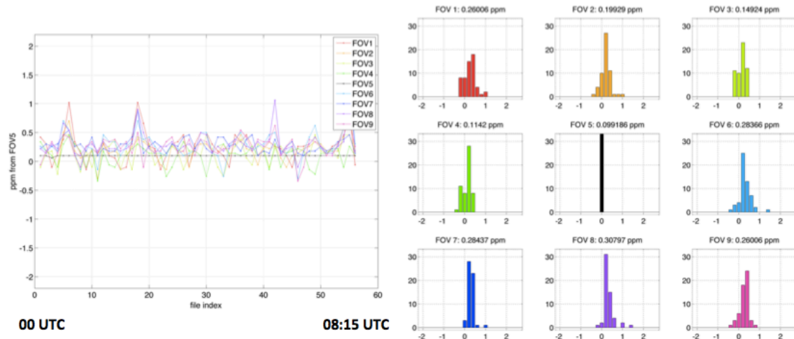
Figure 23.1.3. The results of an example analysis of inter-FOV spectral calibration analysis, for data following a sensor/platform warm-up/cool-down event on 24/25 March. As part of the CrIS spectral characterization and ILS parameter refinement in the Early Cal/Val phase, we have contributed a unique analysis technique and results for determining the inter-FOV spectral calibration for all three spectral bands, including the lower resolution shortwave band. This analysis and results are reflected in the FOV positions in the v33 Eng. Packet. In this figure, the left hand plot shows a time series of inter-fov spectral shifts from the center FOV5 in parts per million (ppm), and the right hand panels show a histogram of the shifts for each FOV. This shows excellent spectral performance of the sensor as well as the ability to characterize this performance with this technique, with inter-FOV spectral shifts less than a few tenths ppm.
