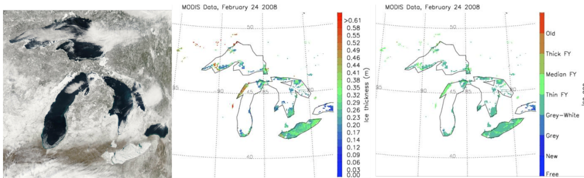
Figure 16.16.2. MODIS Aqua true color image (left) on February 24, 2008 over Great Lakes, retrieved ice thickness (middle) in meter, and ice age (right).
