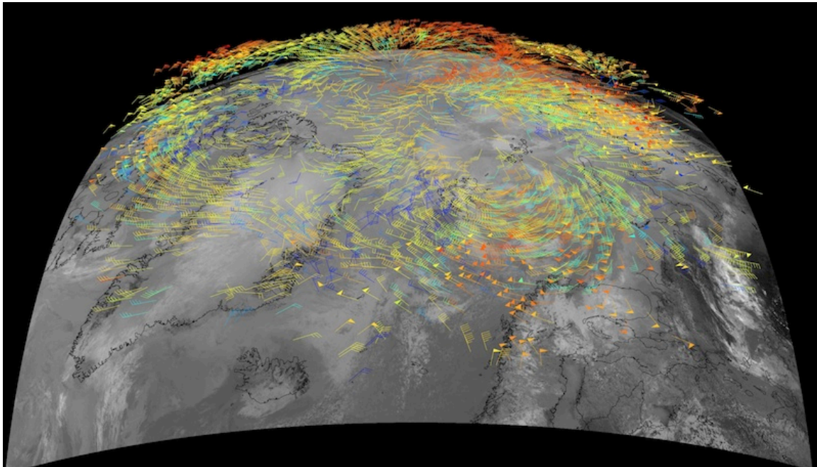
Figure 14.4.1. MODIS derived polar winds over the Arctic. The McIDAS-V globe projection is used to display the winds.
