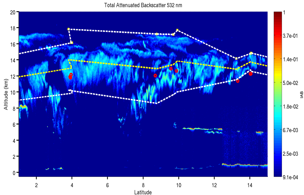
Figure 3.5.7. CALIPSO total attenuated backscatter with collocated AMV locations plotted in red. The white lines are the CALIPSO cloud top altitude and cloud base altitude. The yellow line represents the midpoint of the cloud layer.
