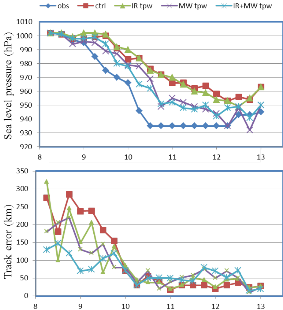
Figure 12.2. The sea level pressure (upper) and track (lower) errors of analysis (Typhoon Sinlaku 2008) with MODIS (IR)TPW, AMSR-E (MW) TPW, and IR+MW TPW, respectively.
