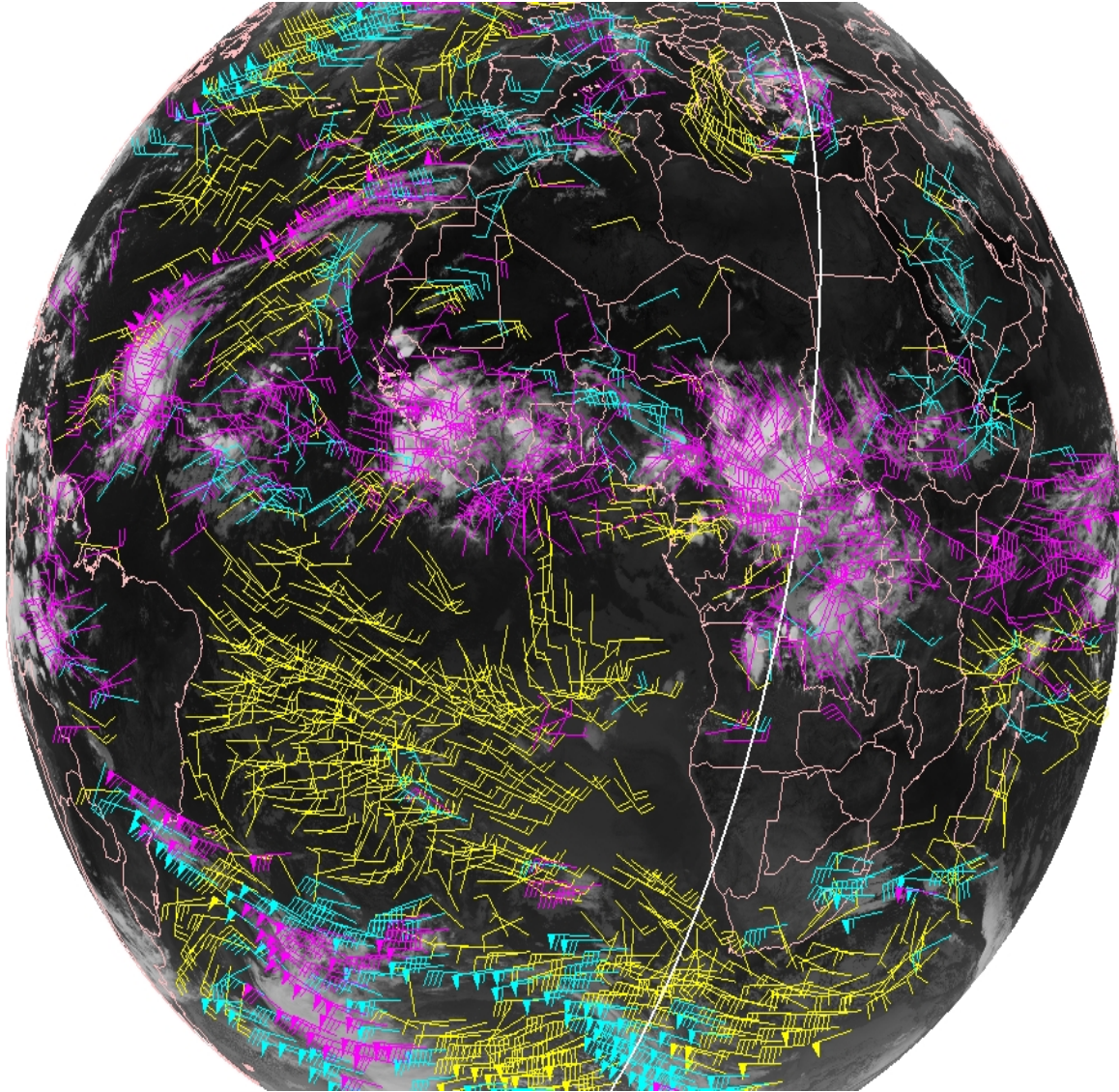
Figure 3.5.4. LWIR AMVs from Meteosat-9 for 22 September 2011 at 00 UTC plotted with the CALIPSO transect locations in white.
