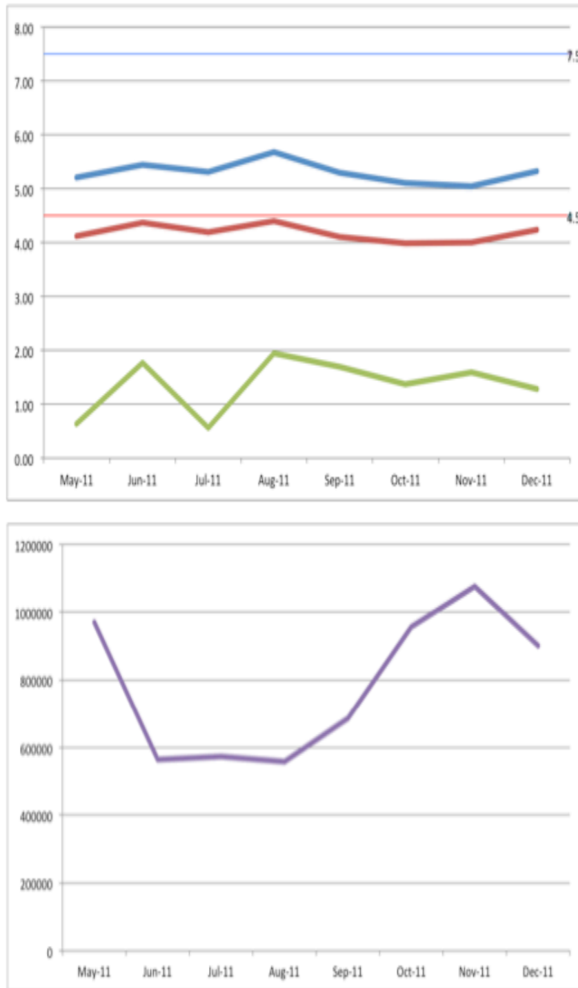
Figure 16.8.2. Monthly comparison statistics (ocean only) between AMVs computed using all bands at upper levels (100 – 400 hPa) from full disk Meteosat-9 and NCEP GFS Analysis winds (valid at all synoptic times) for the months of May 2011 through December 2011. Bottom image is the number of AMV GFS analysis matches.
