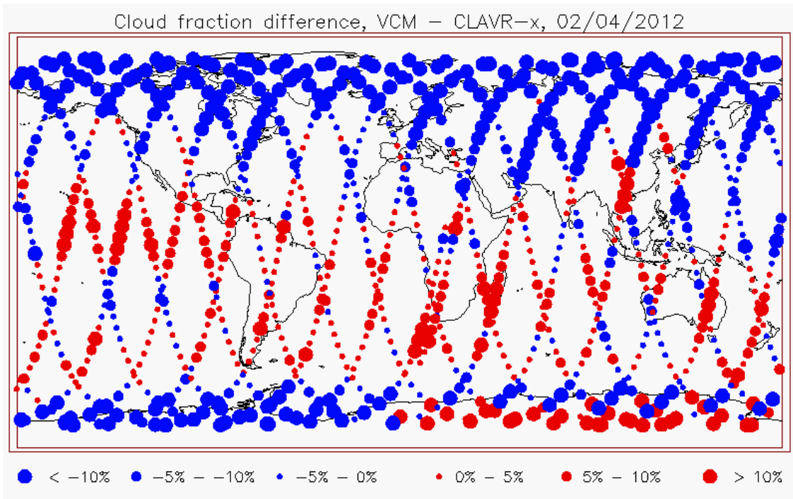
Figure 21.2. Global comparison between VIIRS cloud mask and a cloud mask produced in CLAVR-x.
