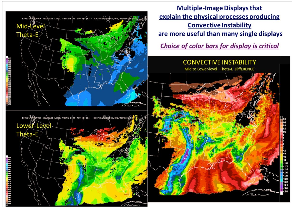
Figure 14.7.2. Example of multiple panel display of a 6 hour NearCast of derived Convective Instability (right panel) and component parameter fields (left panels) from 0000 UTC 25 May 2011. Reds and yellows in left panels indicate areas of lower \theta_E (cooler, drier air) and greens and blues indicate higher \theta_E (warmer, moister air). Scales change from lower to upper panels. Red areas in right panel are convectively stable ( \theta_E increases with height) and blue/purple/white regions indicate greatest convective instability ( \theta_E increases with height).
