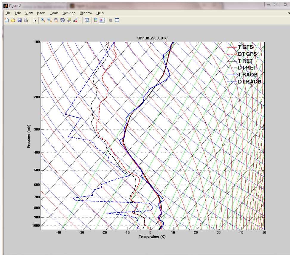
Figure 16.7.2. The skew-T diagram includes the temperature and dewpoint temperature profiles for GFS, GOES Sounder physical retrieval (with GOES-R LAP algorithm), and radiosonde measurement on 2011.01.26 00UTC over ARM CART site.
