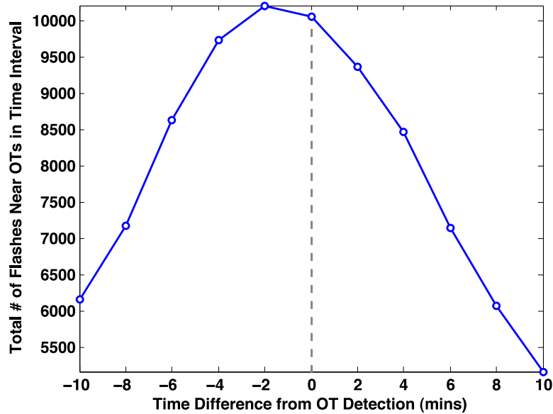
Figure 14.2.2. Total number of lightning flashes near overshooting-tops vs. time difference from GOES imager overshoot detection in minutes.
