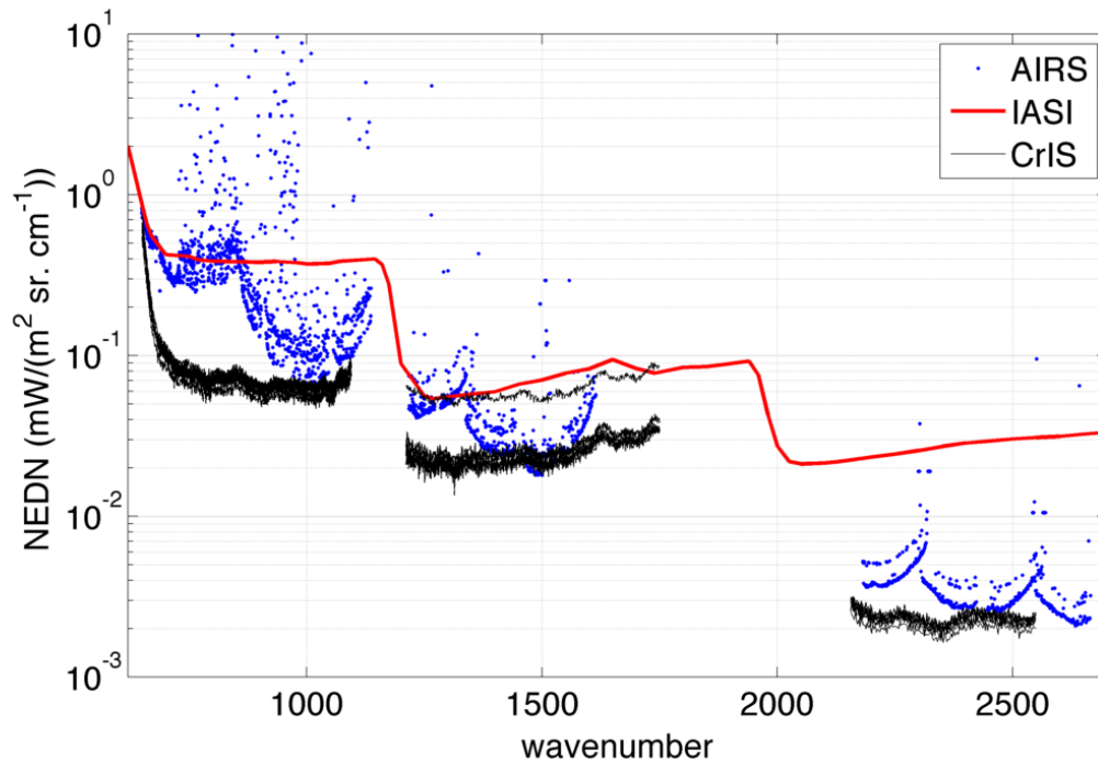
Figure 23.1.4. CrIS in-flight noise performance (black) as compared to the noise performance of AIRS (blue) and IASI (red). (Noise is shown here for each sensor for their native spectral resolutions and FOV sizes). This CrIS random noise estimate was produced from analysis of ensembles of ICT and Space view data collected on 21 January. Spectrally correlated noise is very small and difficult to estimate. As expected, the noise performance of CrIS is very good. It is lower than AIRS and IASI by roughly a factor of 5 in the longwave region, slightly better than AIRS in the midwave region, and also slightly better than AIRS (and significantly better than IASI) in the shortwave region.
