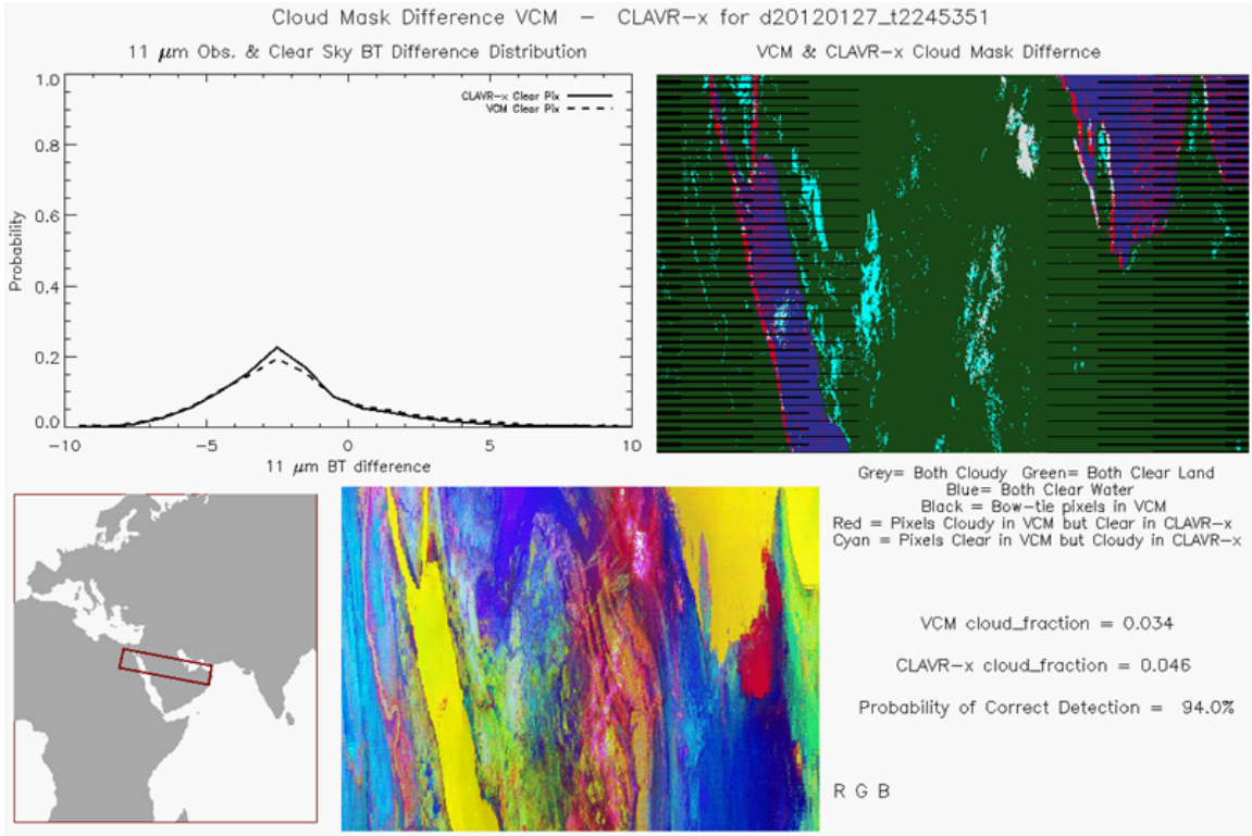
Figure 21.1. Comparison between the VIIRS cloud mask (VCM) and a cloud mask produced in CLAVR-x over the Arabian peninsula, showing geo-location errors leading to false cloudiness along some coastlines.
