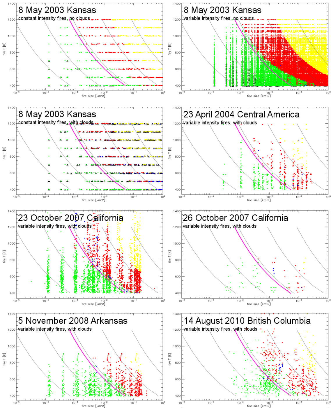
Figure 16.6.1. Scatter plots developed at CIMSS from the 8 ABI model-derived proxy cases developed at CIRA. Fires detected by the current GOES WF_ABBA were used as inputs. The horizontal axis is a logarithmic scale of fire size, and the vertical scale is fire temperature. The color coding indicates the type of fire or whether the fire was detected at all. Green indicates that the fire was not detected, red indicates a detected fire that was characterized, yellow indicates a saturated fire pixel, magenta indicates a cloud covered pixel, orange a high possibility fire pixel, and blue a medium possibility fire pixel. The curved lines are lines of constant FRP, in powers of 10 MW. The heavy magenta line is the 75 MW line, below which very few fires are detected.
