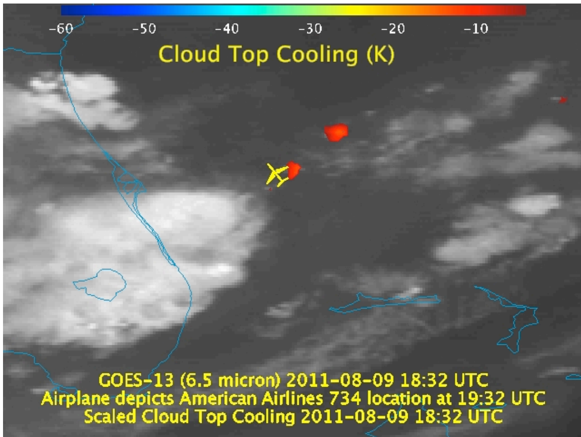
Figure 14.4.2. GOES image over Florida and Bahama Islands, with location of cloud top cooling maxima and location where airplane encountered turbulence on 9 August 2011.
