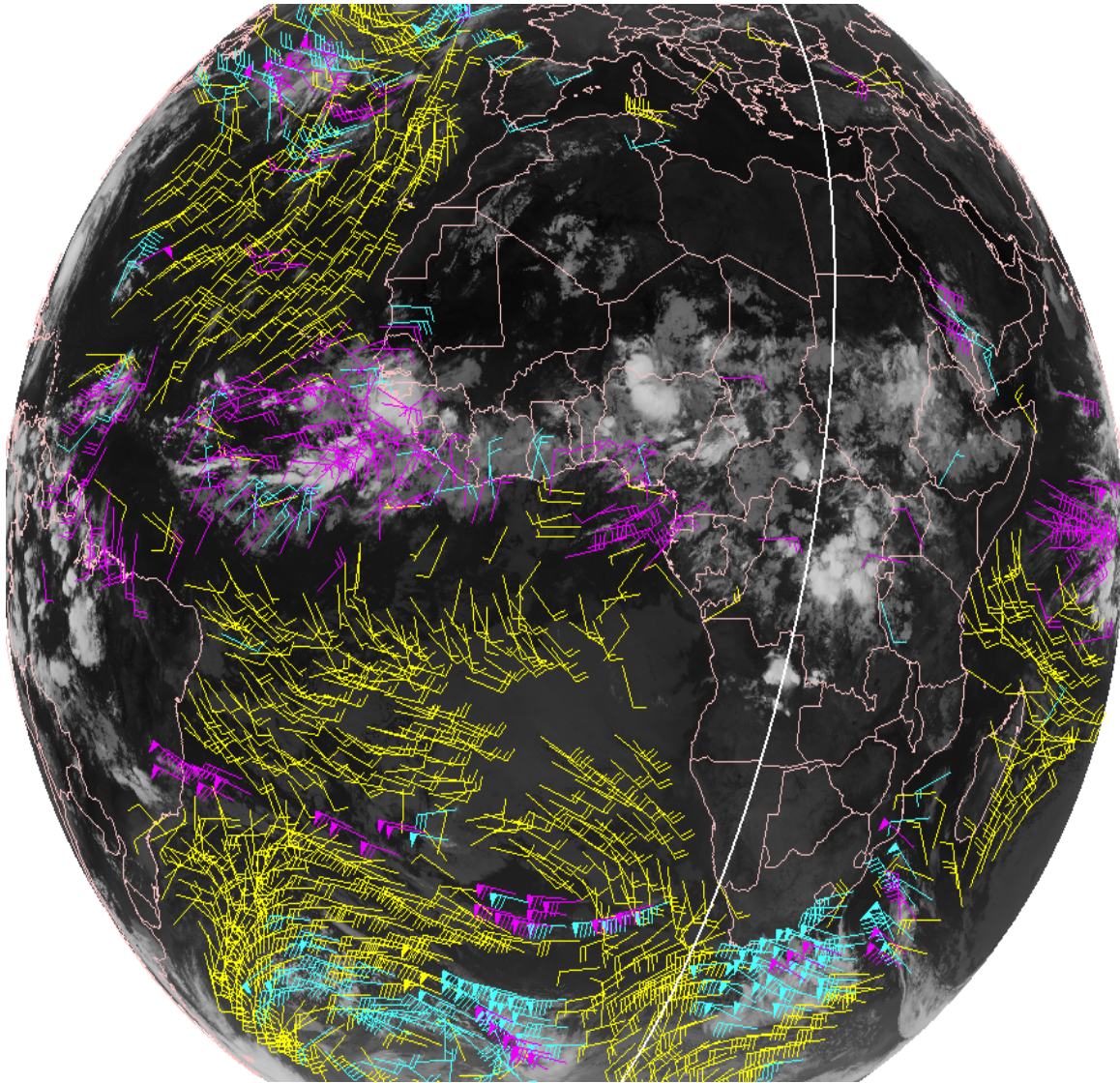
Figure 3.5.1. LWIR AMVs from Meteosat-9 for 15 September 2011 at 00 UTC plotted with the CALIPSO transect locations in white.
