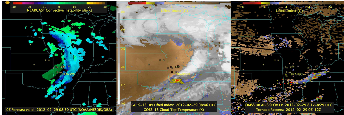
Figure 14.4.4. Comparison between the results of the CIMSS NEARCAST convective instability, the GOES sounder lifted index derived product imagery and the AIRS Dual Regression Lifted Index from an overpass near to a reported tornado formation near Branson, MO on 29 February 2012.
