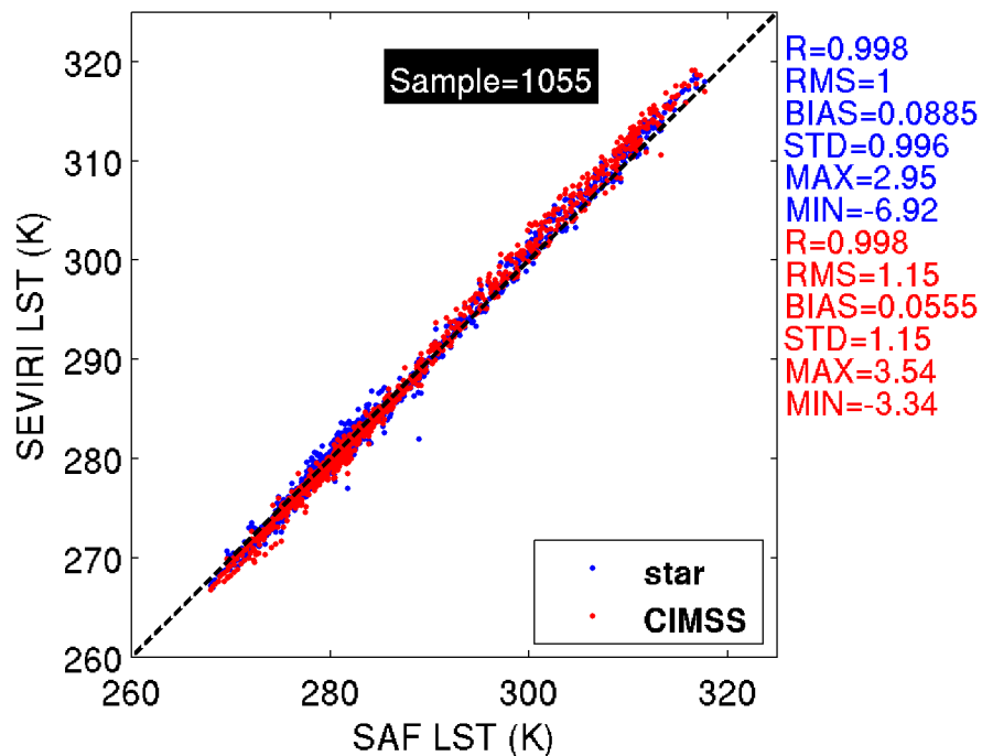
Figure 16.7.6. Same as Figure 16.7.4 except that retrievals with averaged BT residuals larger than 0.2 K are not included.
