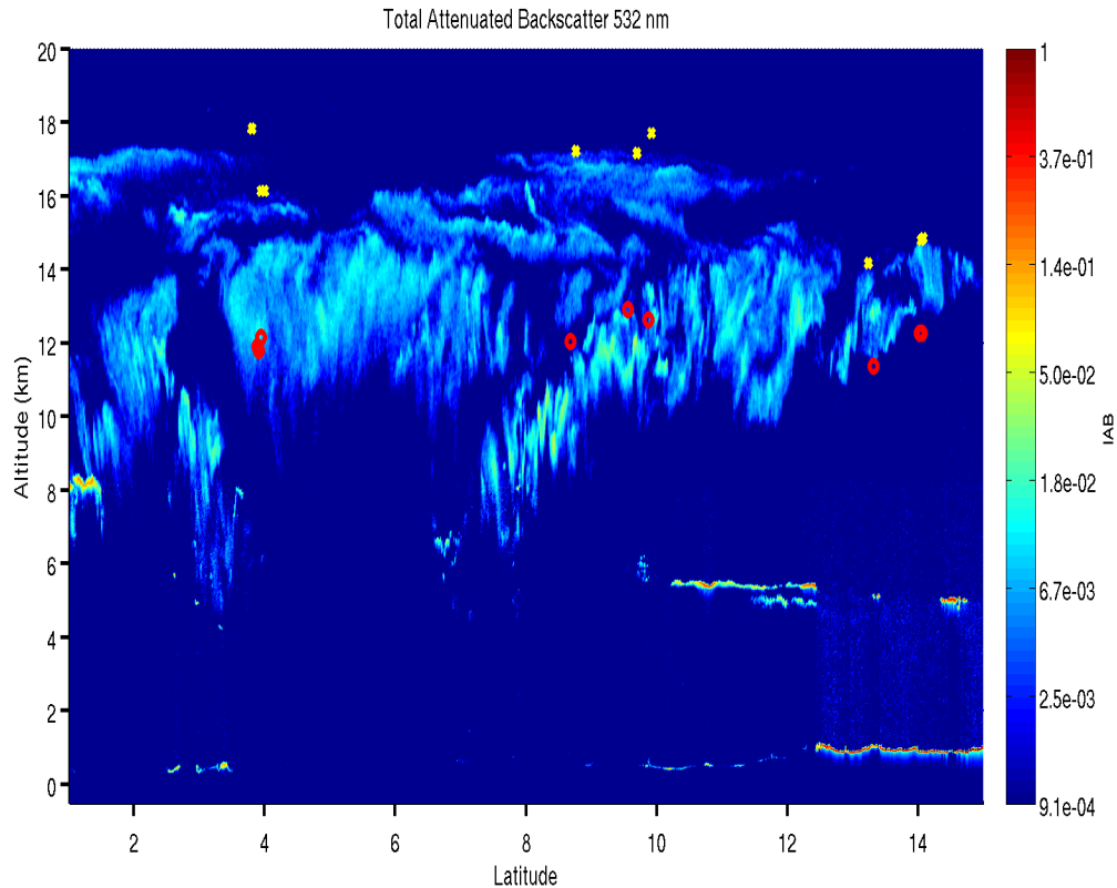
Figure 3.5.6. CALIPSO total attenuated backscatter with collocated AMV locations plotted in red and CALIPSO clouds in yellow.
