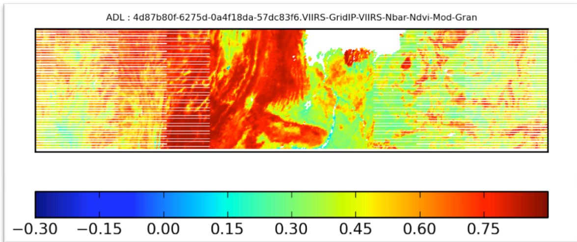
Figure 25.1: NDVI ancillary data processed in IDPS.
