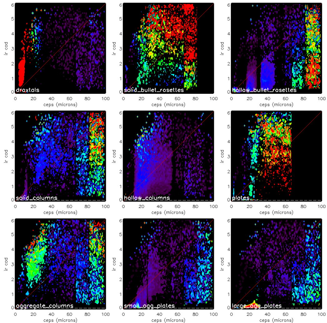
Figure 11.1. Relative frequency of occurrence of the habits from the Ping Yang Spectral Library relative to optical depth and particle size. Habits were detected when their effective radius differences between the 8.5/11\mu\text{m} and 11/12\mu\text{m} \beta values were smallest in magnitudes compared to the values from all habits.
