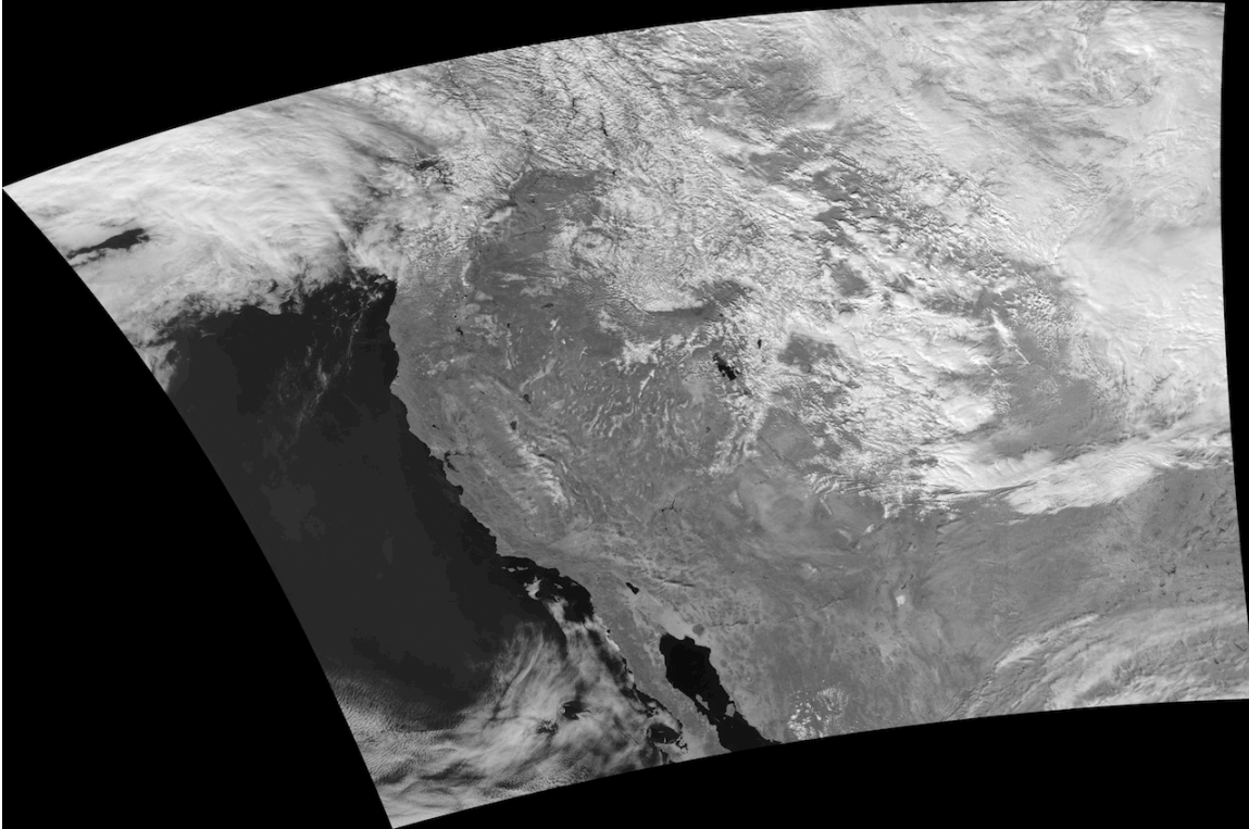
Figure 26.2. First VIIRS data received at SSEC and processed using CSPP (2012/02/23)
