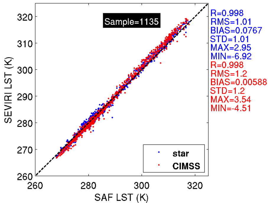
Figure 16.7.4. Scatter plots of LST from CIMSS and STAR using SAF (satellite application facility) LST measurements as reference.
