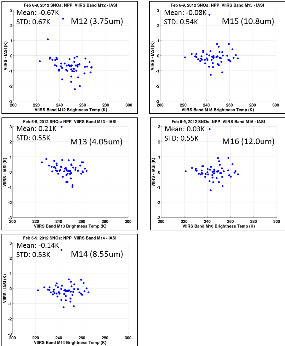
Figure 23.2.1. Calibration comparison of pre-Beta designation NPP VIIRS and Metop-A IASI instruments using simultaneous nadir overpasses (SNOs) from Feb 6-9, 2012. SNOs within +/- 10 minutes are collected to evaluate VIIRS radiance calibration against IASI. These early VIIRS SDR results are favorable, showing biases near to zero for all bands and without any apparent scene temperature dependence.
