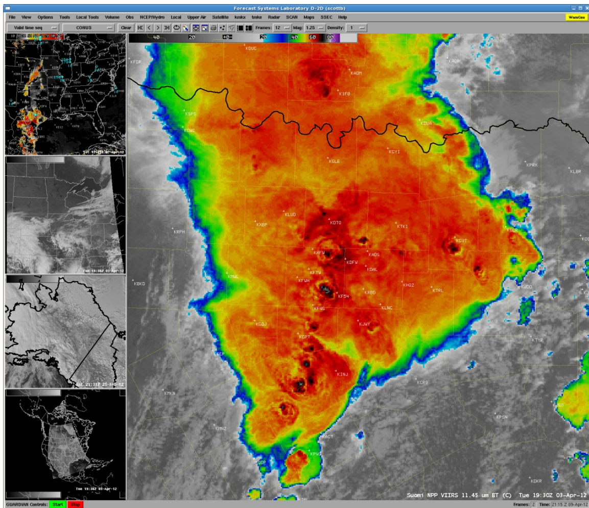
Figure 7.1. AWIPS screen capture of a Suomi NPP VIIRS infrared image of the thunderstorm complex that produced an outbreak of tornadoes and large hail in the Dallas-Fort Worth, Texas region on 03 April 2012. Examples of similar VIIRS imagery will be used in the development of a new VISIT lesson “Suomi NPP VIIRS Imagery in AWIPS.”
