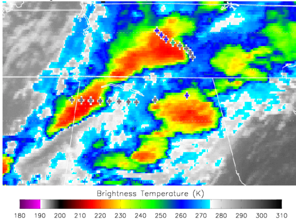
Figure 14.2.1. 10.7 micron infrared window imagery from GOES-12 and United Airline flight tracks of EDR objectively determined turbulence (grey – null, blue –weak, green –moderate) from May 2, 2010 at 2302 UTC.
