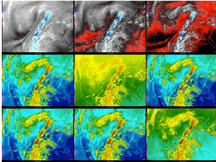
Figure 15.1. UW-CIMSS NSSL-WRF simulated GOES-R ABI IR imagery. All 9 non-solar bands can be produced from the NSSL-WRF.
