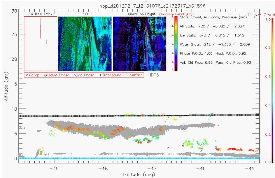
Figure 23.5.1. VIIRS cloud top height granule for February 17 th 2012 on the top of the figure. The bottom figure overlays the VIIRS cloud top height on a CALIOP attenuated backscatter profile.
