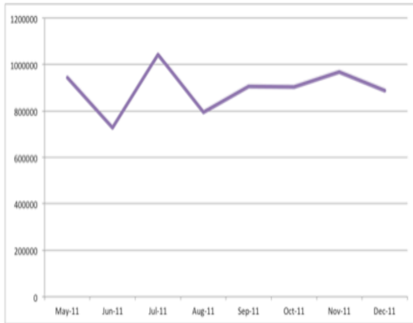
Figure 16.8.4. Monthly comparison statistics (ocean only) between AMVs computed using all bands at low levels (below 700 hPa) from full disk Meteosat-9 and NCEP GFS Analysis winds (valid at all synoptic times) for the months of May 2011 through December 2011. Bottom image is the number of AMV GFS analysis matches.
