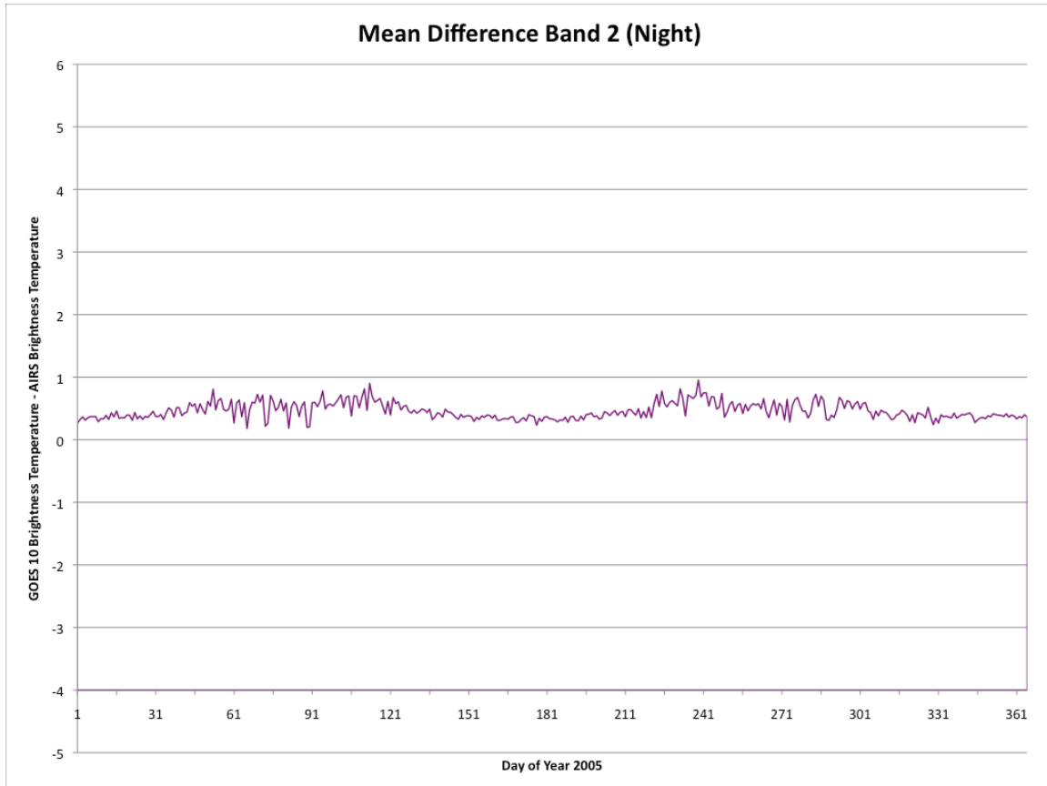
Figure 10.1. GSICS Intercalibration results for band 2 (3.9 micrometer) of the GOES-10 Imager compared to AIRS; GOES is slightly warmer than AIRS by approximately 0.5 K. Only night-time results are shown since reflected solar radiation during the day creates difficulties for comparisons in this shortwave band. The results shown are just for the year 2005.
