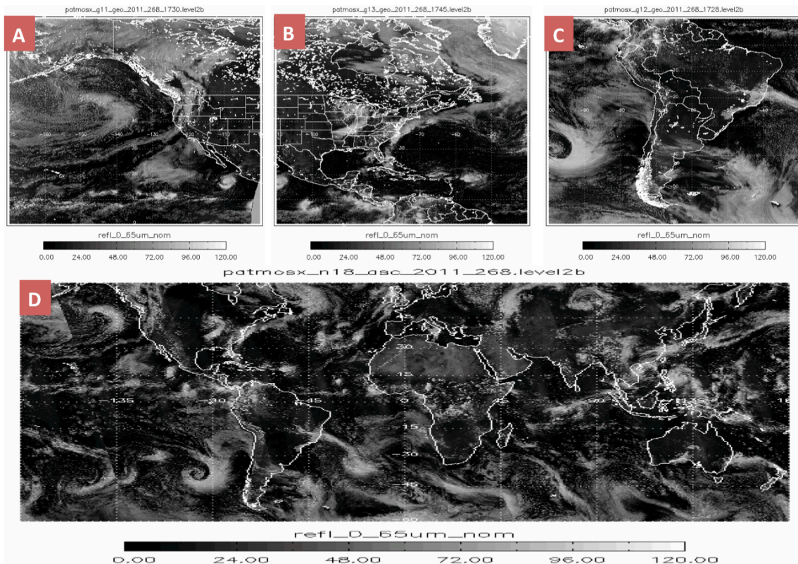
Figure 3.2.1. Illustration of the data domains used for GOES/West (A), GOES/EAST(B) and GOES/South(C). Global domain used for AVHRR PATMOS-x given by (D).
