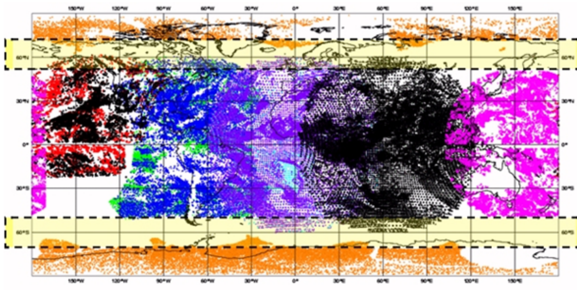
Figure 14.13.1. Daily satellite-derived AMV coverage from polar (orange) and geostationary (other colors) satellites. The yellow-filled rectangles denote the approximate gap in coverage.
