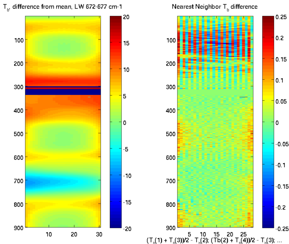
Figure 23.1.5. The left hand panel shows a cross section of brightness temperature variations in the longwave CO 2 (672-677) spectral region with 30 cross track FORs and time increasing from y-axis indices 0 to 900. The right hand panel shows the difference between adjacent FORs in each scan line, and in the upper portion of the figure clearly shows a FOR (interferometer sweep direction) dependent bias in the radiometric calibration. This “striping” effect has largest brightness temperature biases in this spectral region. At 16:15 on April 18 (approximately scan line 300 in these figures), the new on-board FIR filter was uploaded, greatly reducing the size of this effect.
