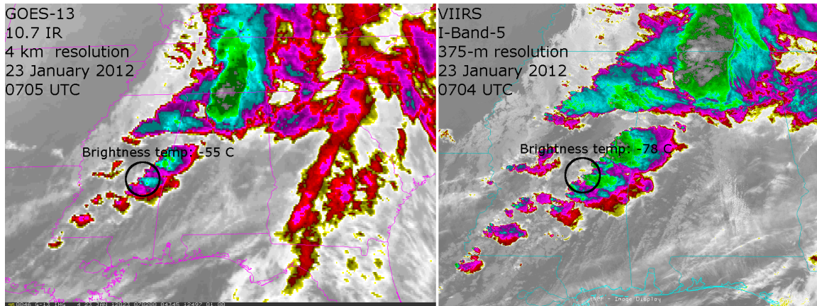
Figure 24.4.1. High spatial resolution thermal band (I-Band 5, 375 m resolution) on VIIRS captures cloud structure not detectable from GOES. In this case, cloud-top temperature difference over 20 deg C.
