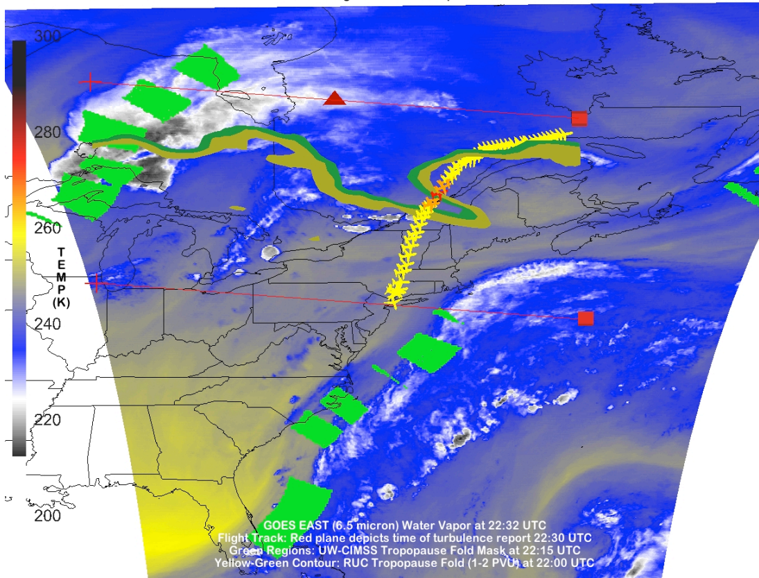
Figure 14.4.3. GOES-East water vapor image; enhancement shows water vapor gradient and associated troposphere fold. Yellow airplanes indicate flight path through troposphere fold.
