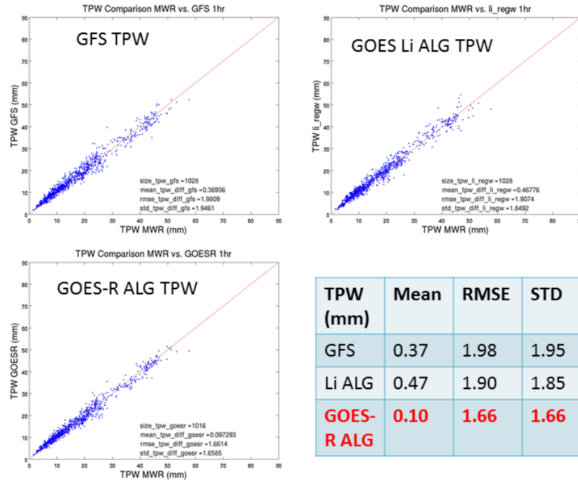
Figure 16.7.1. Scatter plot of GFS TPW (upper left), GOES Sounder Li-ALG TPW (upper right) and GOES-R ALG TPW (lower left) using MWR as reference. The biases, RMSE and Standard Deviation (STD) are also shown the in the table (lower right).
