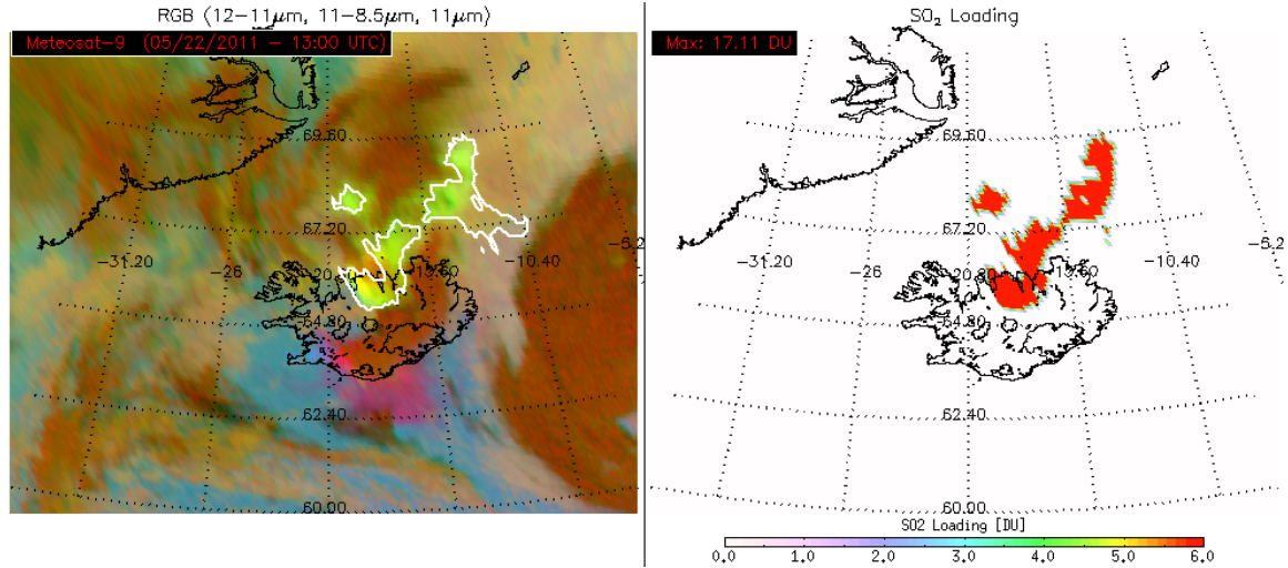
Figure 16.12.1. The results of the binary (e.g., yes/no) GOES-R SO 2 detection algorithm are overlaid on a false color image (left panel) and estimates of the total SO 2 loading are shown in the right panel. The SO 2 cloud shown in this example was produced by an eruption of Grimsvotn (Iceland) on May 22, 2011.
