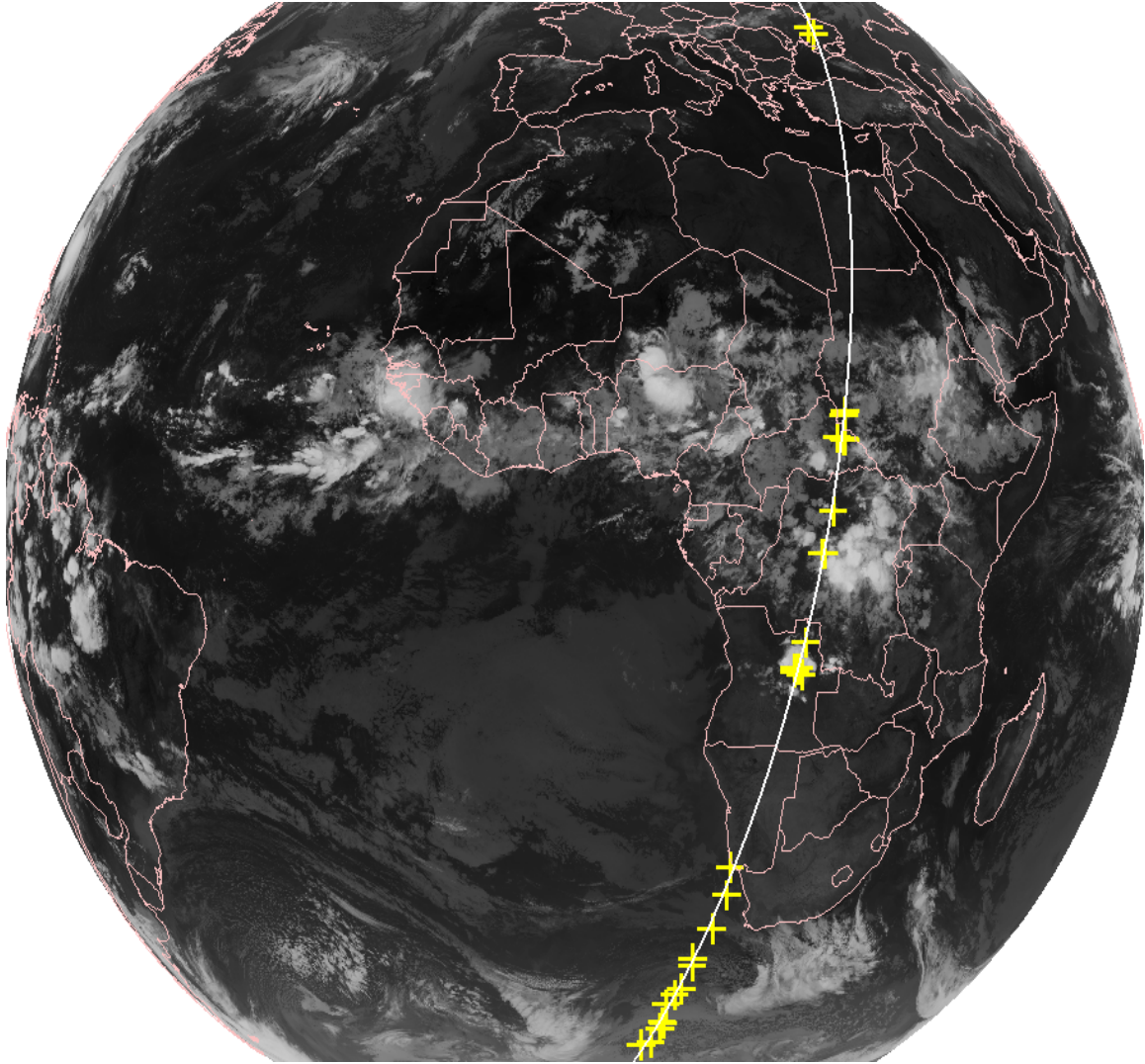
Figure 3.5.2. AMV CALIPSO match locations for 15 September 2011 at 00 UTC.
