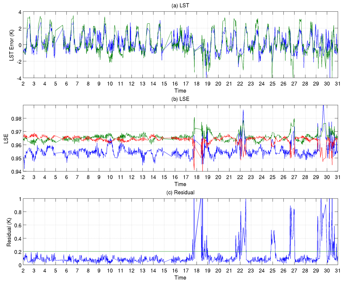
Figure 16.7.5. Time series of (a) retrieved LST errors (green is CIMSS LST, blue is STAR LST), (b) retrieved LSE, and (c) averaged residual.
