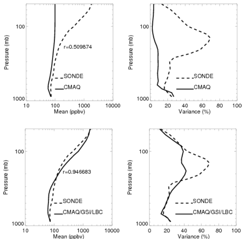
Figure 5.2.1. Comparison between Beltsville and Edgewood, MD ozonesondes and NMMB-CMAQ baseline (upper panels) and GOES TCO assimilation experiments using GFS LBC (lower panels) for 63 ozonesondes during July 2011. The left hand panels show vertical profiles of mean CMAQ (solid) and SONDE (dashed) ozone profiles (ppbv), the right hand panels show vertical profiles of ozone variance (%) for CMAQ (solid) and SONDE (dashed).
