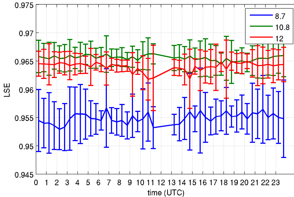
Figure 16.7.3. The daily average of the 3 SEVIRI window channel emissivities retrieved using GOES-R ABI emissivity algorithm. The bar denotes the standard deviations.
