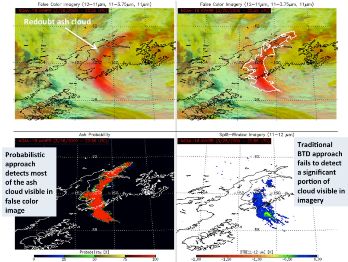
Figure 14.1.1. An example of the probabilistic ash detection scheme developed for the GOES-R Volcanic ash alert system. Top left is a false color image of the Redoubt volcano ash cloud (red areas). Top right is the same false color image with the probabilistic ash cloud object outlined in white. Bottom left are the pixel-level ash probabilities. Bottom right is the traditional 11-12 \mu\text{m} brightness temperature difference used to detect volcanic ash. Note the probabilistic methodology captures most of the ash cloud visible in the false color imager, while the traditional brightness temperature difference method fails to detect a significant portion of the ash cloud.
