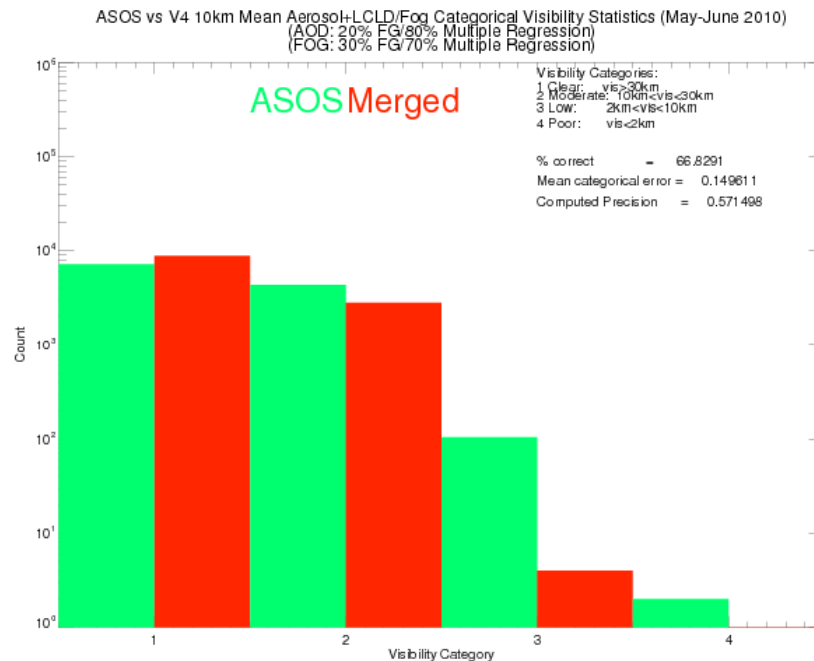
Figure 16.15.1. Categorical Histogram of V4 Merged ABI (red) and ASOS (green) aerosol and fog/low cloud visibility for May-June 2010 coincident pairs.
