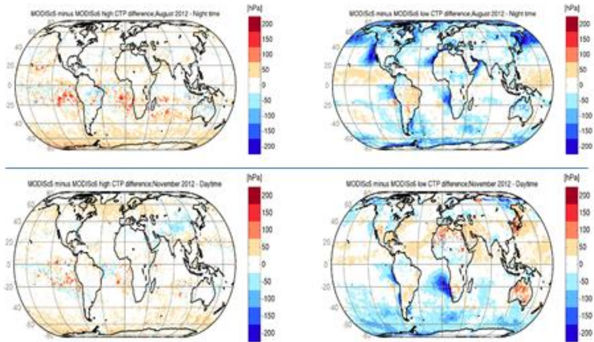
Figure 17: Global Distribution of C5 minus C6 CTP Differences. CTPs from Aqua C5 and C6 for August and November 2012 have been compared. More transmissive cirrus are being reported as high cloud both day and night. C6 high cloud CTPs in mid-latitude oceans have decreased by ~50 hPa. C6 low marine stratus CTPs have increased by ~150 hPa. C5 to C6 adjustments vary seasonally.
