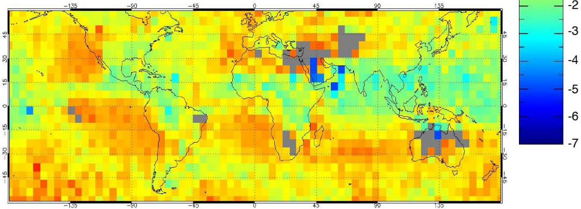
b. MODIS Collection 6 CTH - CALIOP
