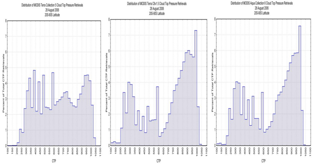
Figure 16: Vertical distribution of clouds (percent of CTP retrievals on y-axis, CTP in 100 hPa bins on x-axis) for 28 August 2006 with Terra C5 (left) & C6 (middle) along with Aqua C6 (right) results for 90°S-20°S. C6 results show better Terra and Aqua agreement.
