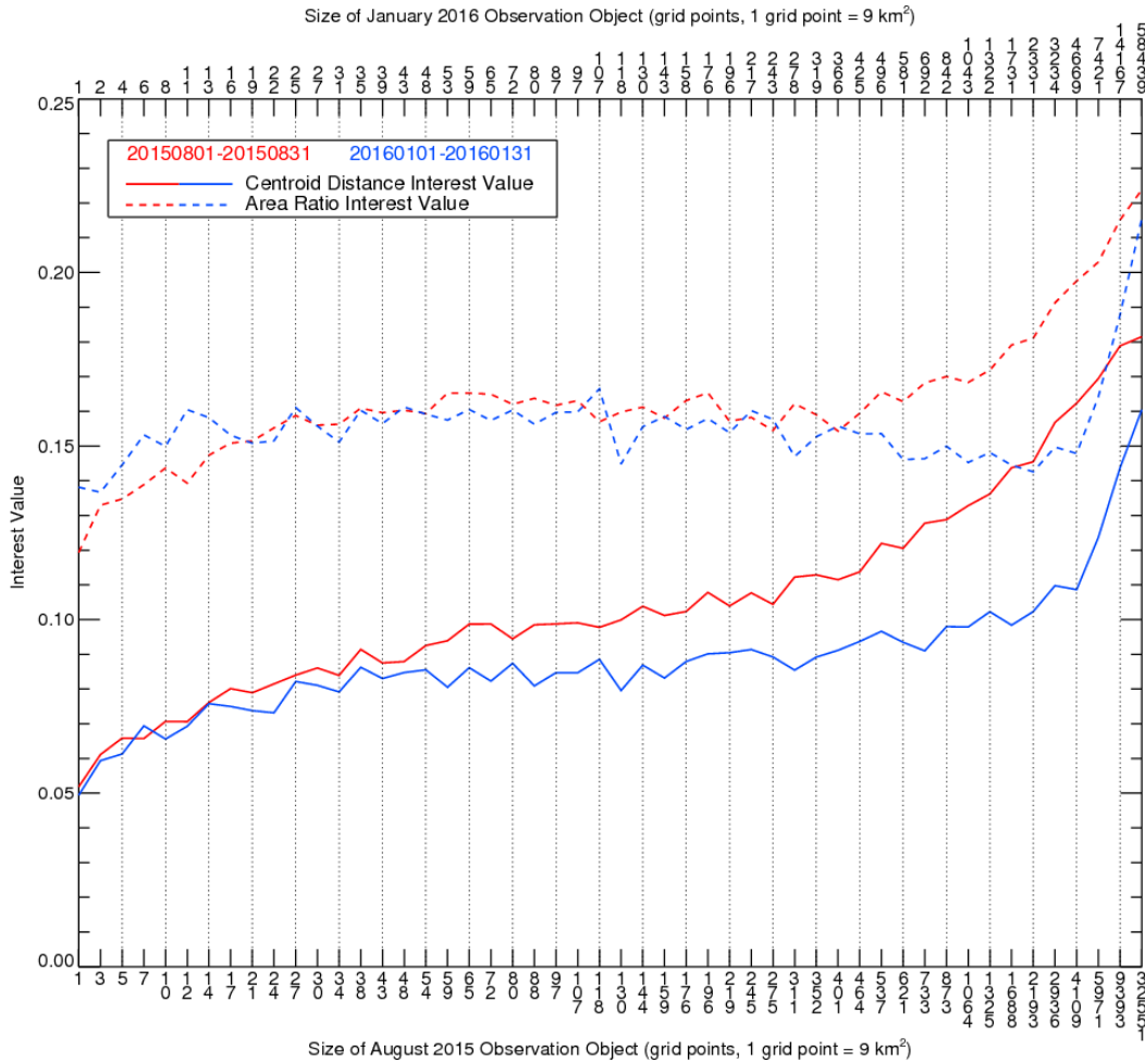
Figure 45. Line plot depicting interest values for the centroid distance (solid) and area ratio (dashed) object attributes for August 2015 (red) and January 2016 (blue) plotted as a function of observed object size. The matched observed objects are separated into 50 bins, based on the observed object size, and the interest values and observed object sizes for each bin are averaged.
