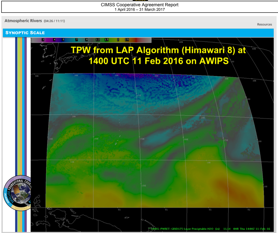
Figure 43. AHI all-sky TPW image at 14:00 UTC on 11 February 2016 from AWIPS-II showing atmospheric rivers.
