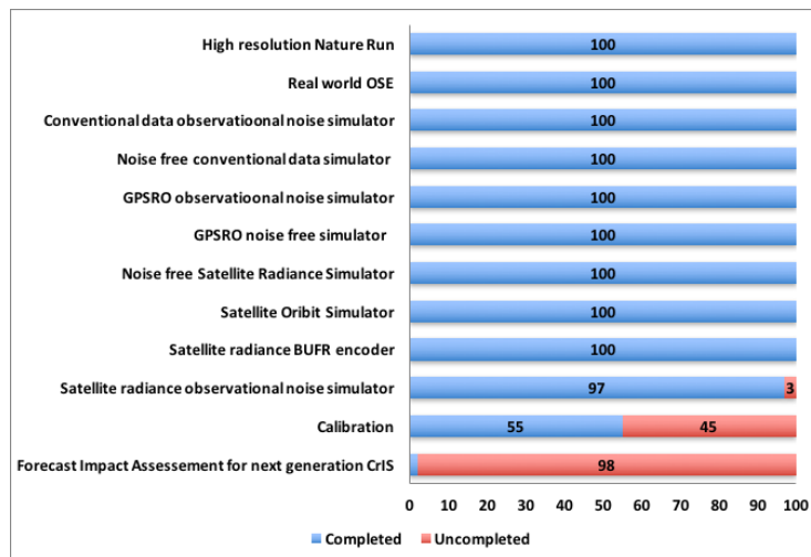
Figure 99. Progress of various components of the OSSE as of March 2017.
