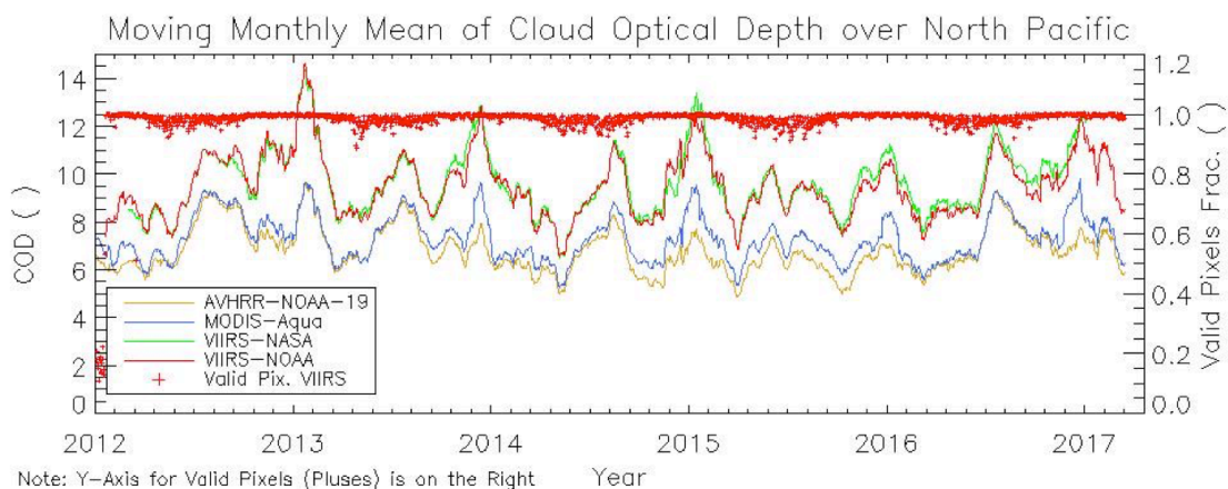
Figure 73. Time series of cloud optical depth as retrieved using the DCOMP algorithm from AVHRR/NOAA-19 (yellow line), MODIS/Aqua (blue line), Suomi NPP/VIIRS using NASA calibration (green line), and Suomi NPP/VIIRS using NOAA calibration (red line). The fraction of valid VIIRS pixels are tracked using red plus symbols.
