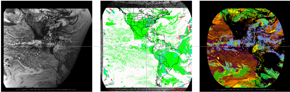
Figure 21. Simulated GOES-R ABI data with products from CLAVRx. Left most image is the simulated 0.65 um reflectance data. Middle image shows the results of the cloud mask. The right most image is the retrieved cloud top height (CTH) product.
