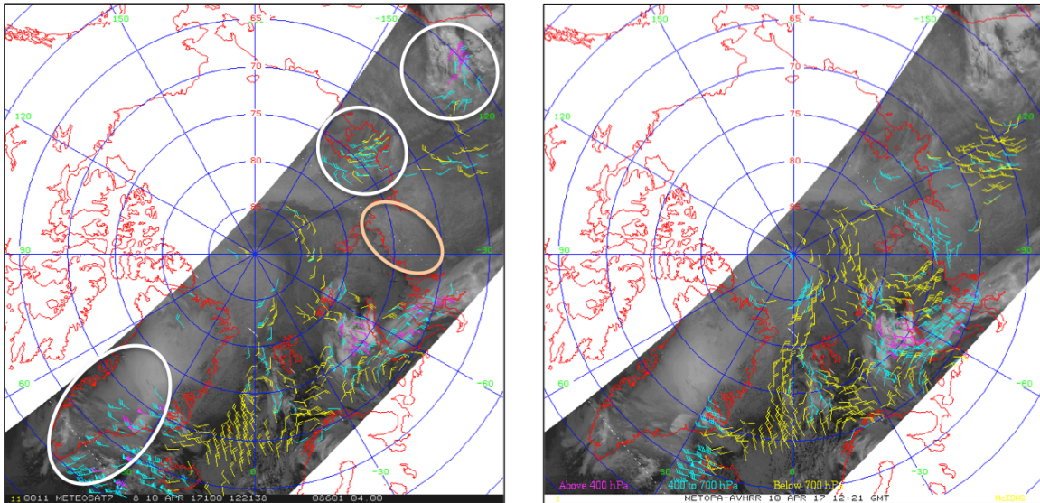
Figure 102. Metop polar winds from alternating Metop-A and Metop-B passes (left) and three successive Metop-A passes (right) on 10 April 2017 at 1221 UTC. Colors represent the height of the wind vectors: Yellow (1000 to 700 hPa), cyan (700 to 400 hPa), magenta (about 400 hPa). The white circles denote regions where the mixed-satellite passes retrieved additional winds over the single-satellite mode. The orange circle is a region where fewer winds were retrieved, due to a missing scan of Metop-B IR data.
