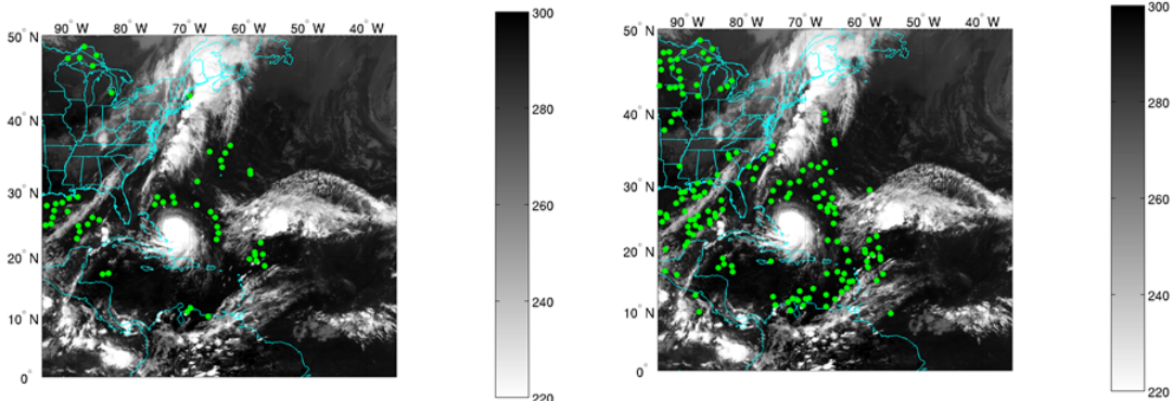
CrIS Original data assimilated at 09-30 18z of channel 130
