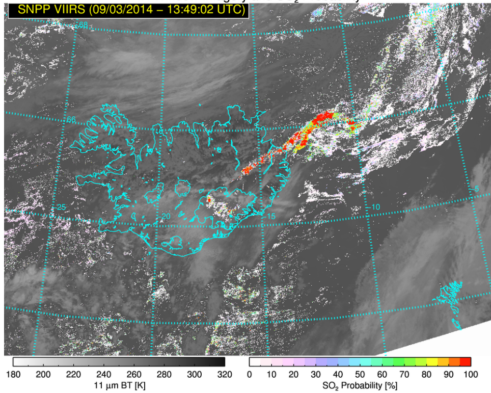
IR Window Imagery and SO 2 Probability
