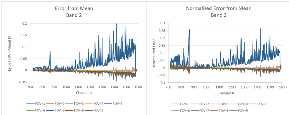
Figure 101. CrIS detector differences for band 2 (midwave). Left panel are errors in degrees Kelvin. Right panel are normalized errors. Detector 7 errors are up to 0.2K or 25% higher than the other detectors.
