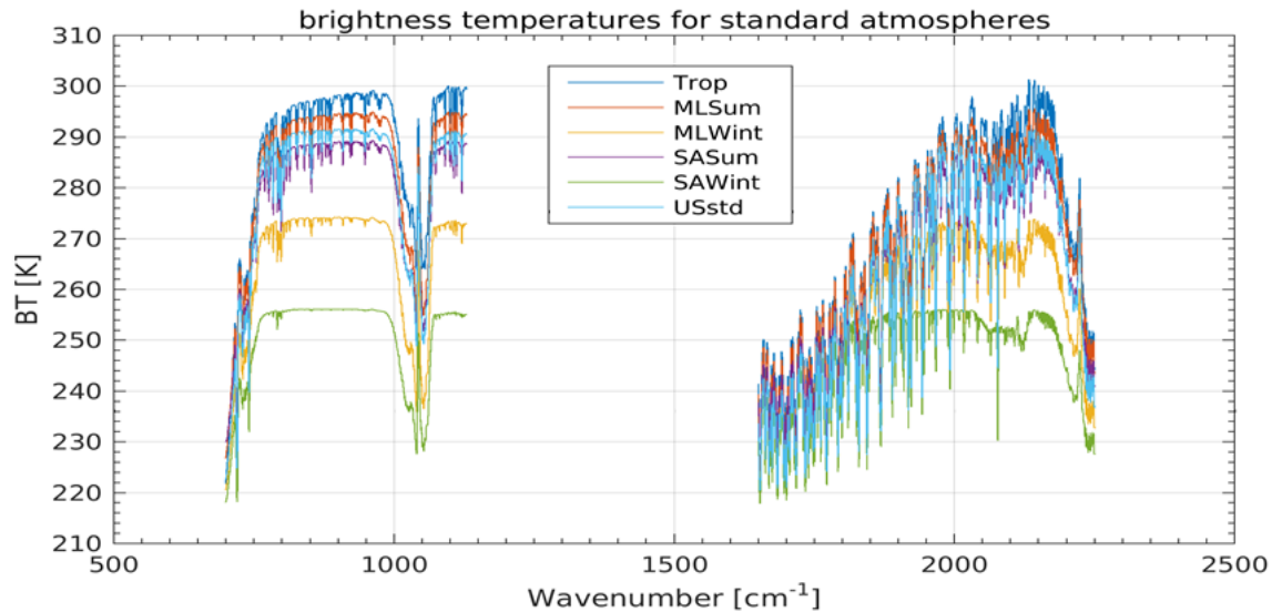
Figure 41. GIIRS Spectra for various standard atmospheres.
