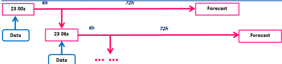
Figure 33. Data assimilation and forecast experiment schemes for hurricane Harvey (2017).
