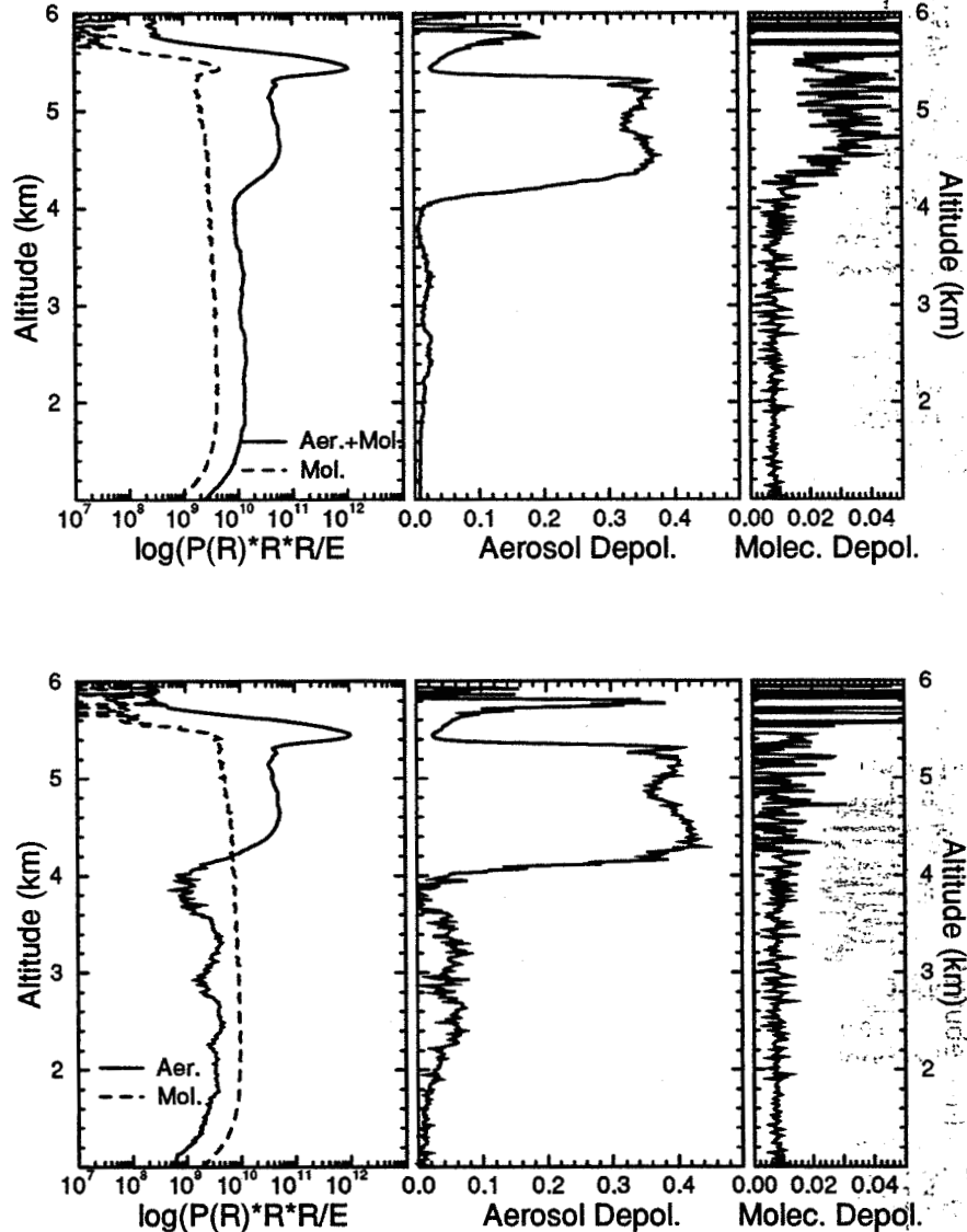
Figure 29. Raw and inverted depolarization ratios of a thin cirrus cloud and a thin water cloud with an ice crystal precipitation (November 11,1993 01:55-02:01 UT). The upper set shows the raw aerosol and molecular profiles along with the raw depolarization ratios. The lower set shows the inverted profiles with the inverted depolarization ratios. The water cloud at 5.5 km has a low depolarization value \sim 1.5\% at the cloud base and it increases towards the cloud top due to the multiple scattering. The dense ice crystal precipitation is visible between 4 and 5.4 km. Because the ice crystal content of the precipitation is large compared to the molecular backscatter, only small difference between raw and inverted aerosol depolarizations is observed. The raw molecular depolarization shows a small increase for the cloud, but after the inversion a constant 0.8% depolarization is observed.
