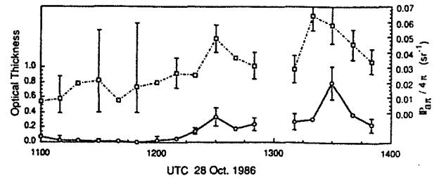
FIG. 9. Time history of the total cloud optical depth (—) and bulk normalized backscatter phase function (---, sr ^{-1} ) coincident with the backscatter cross sections plotted in Fig. 8. Ten minute averaging has been applied (see section 3) to smooth the data. The largest values of backscatter phase function values in this record coincide with the cirrus regions containing altocumulus cells.
