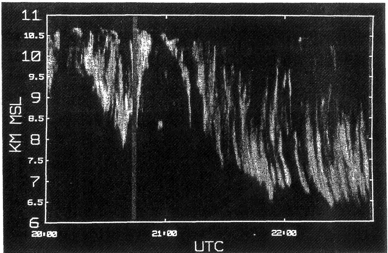
FIG. 12. Intensity modulated height time display of the R^2 corrected HSRL aerosol channel signal. The image has 10 times the temporal resolution necessary to produce the calibrated attenuation corrected cross section plotted in Fig. 10. The image reveals an \sim 5 minute structure ( \sim 9 – 11 km wide) imbedded in the larger scale organization shown in Fig. 10.
