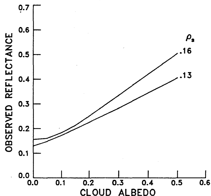
FIG. 22a. Theoretical top-of-the-atmosphere visible reflectance over WAU for 1400 UTC ( \rho_s = 0.13 ) and for 1800 UTC ( \rho_s = 0.16 ).
