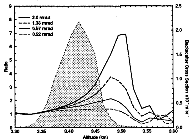
Figure 1. Ratios of the WFOV signals to the signal in the 0.16 mr spectrometer channel. WFOV acceptance angles of 0.22, 0.57, 1.38 and 3.0 mrad are shown. The backscatter cross section is shaded.
