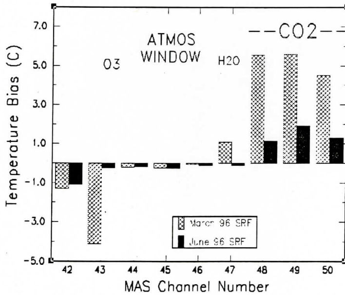
Figure 4. MAS-HIS biases on 13 April 1996 using March '96 MAS spectral response (SRF) compared to June '96 SRF. Biases are strongly reduced using the June '96 SRF indicating that during SUCCESS, the MAS spectral characteristics were closely matched by the June '96 SRF.
