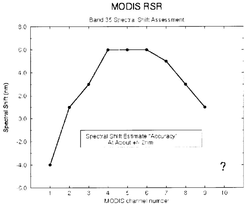
Figure 2. MODIS band 35 spectral correction for each channel. The estimated spectral correction is arrived at by matching spectral features of observed RSR data with that of forward model transmittances. “?” indicates that channel 10 yielded ambiguous results for spectral correction estimate and at this time is considered to be “out of family”. Uncertainty of spectral correction considered to be about +/- 2nm.
