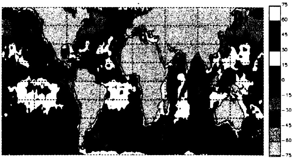
July 1994 CHAPS-ISCCP Cloud Amount Difference (%)
