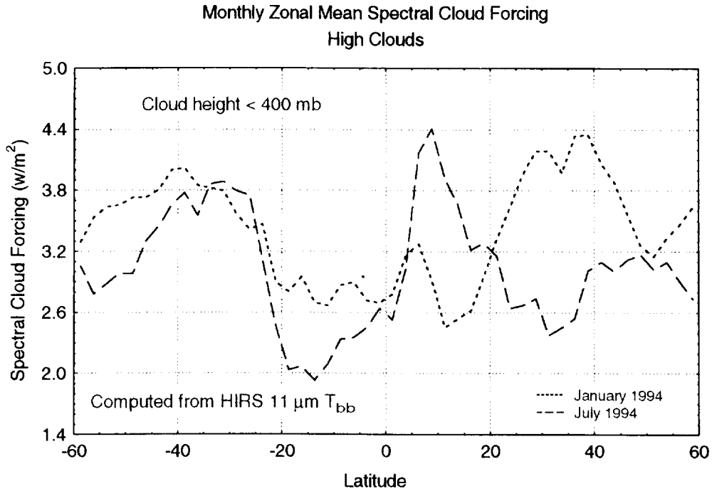
Figure 17. Zonal distribution of 11 \mu\text{m} spectral cloud forcing for January and July 1994, for cloud top pressure less than 400 mb.
