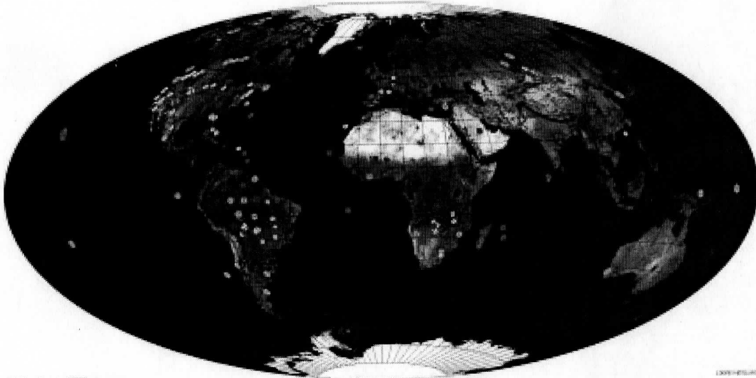
Figure 1. Current and anticipated distribution of AERONET federated sites available for the planned launch of Terra in July 1999. The red symbols denote permanent sites, green seasonal sites, yellow for temporary sites, and blue for future sites. Figure courtesy of Jacques Descloitres, University of Maryland, and is based on a composite of clear-sky SeaWiFS data over a one year period from 1997-1998.
