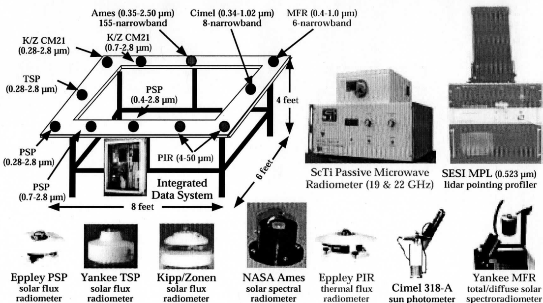
Figure 6. Current and anticipated components of the Mobile Surface Radiation Network (MSRN).
