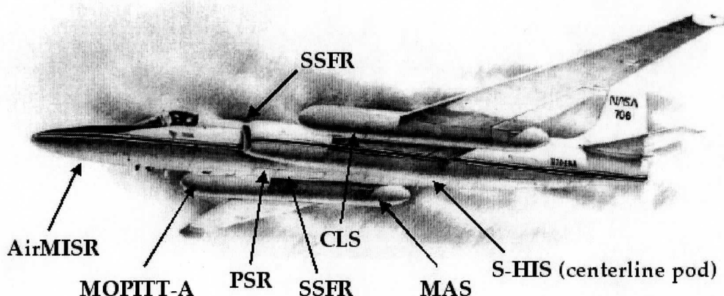
Figure 11. NASA ER-2 configuration for SAFARI 2000.
