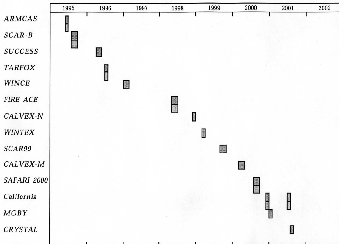
Figure 12. Airborne validation strategy for the MODIS Atmosphere Group from 1995 (pre-launch) through 2002 (post-launch). The blue boxes are for the NASA ER-2 and the gray boxes denote the University of Washington C-131A or CV-580 research aircraft.
