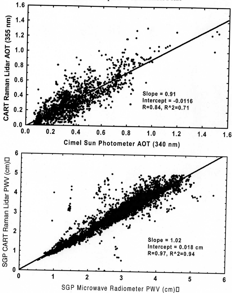
Figure 7. Comparison between CART Raman lidar and (a) Cimel sunphotometer analyses of aerosol optical thickness, and (b) microwave radiometer analyses of precipitable water over the SGP CART site (Ferrare et al.).
